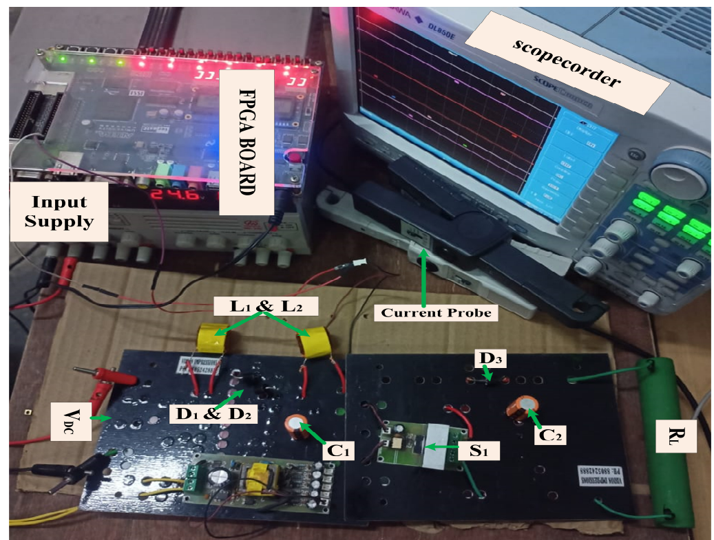
Figure 8. Hardware setups of conventional quadratic boost converter.
