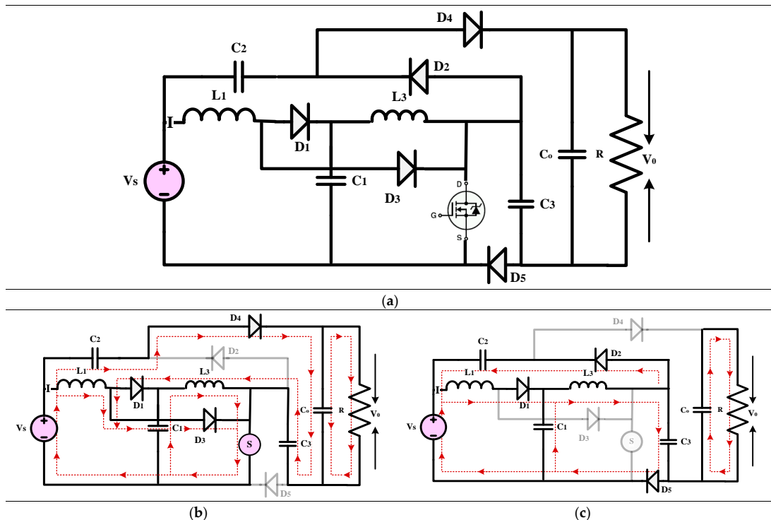
Figure 17. (a) Circuit diagram of QBC based high-gain converter (b) Mode-I Operation (c) Mode-II Operation.
