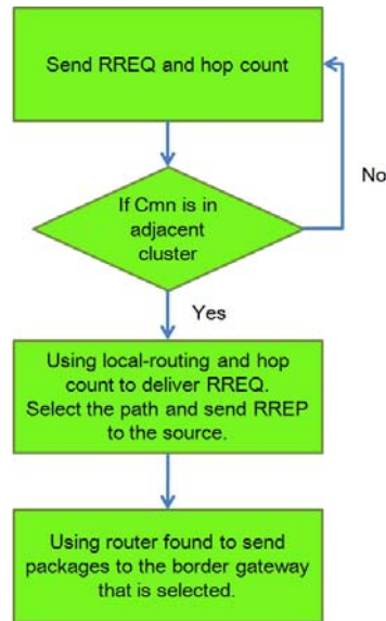
Figure 10. Inter-cluster search for routing algorithm.
