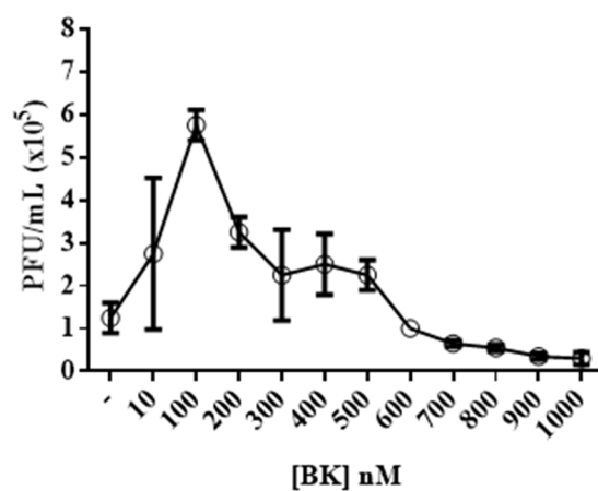
Figure S1. BK dose response of DENV increased replication in HBMEC.
