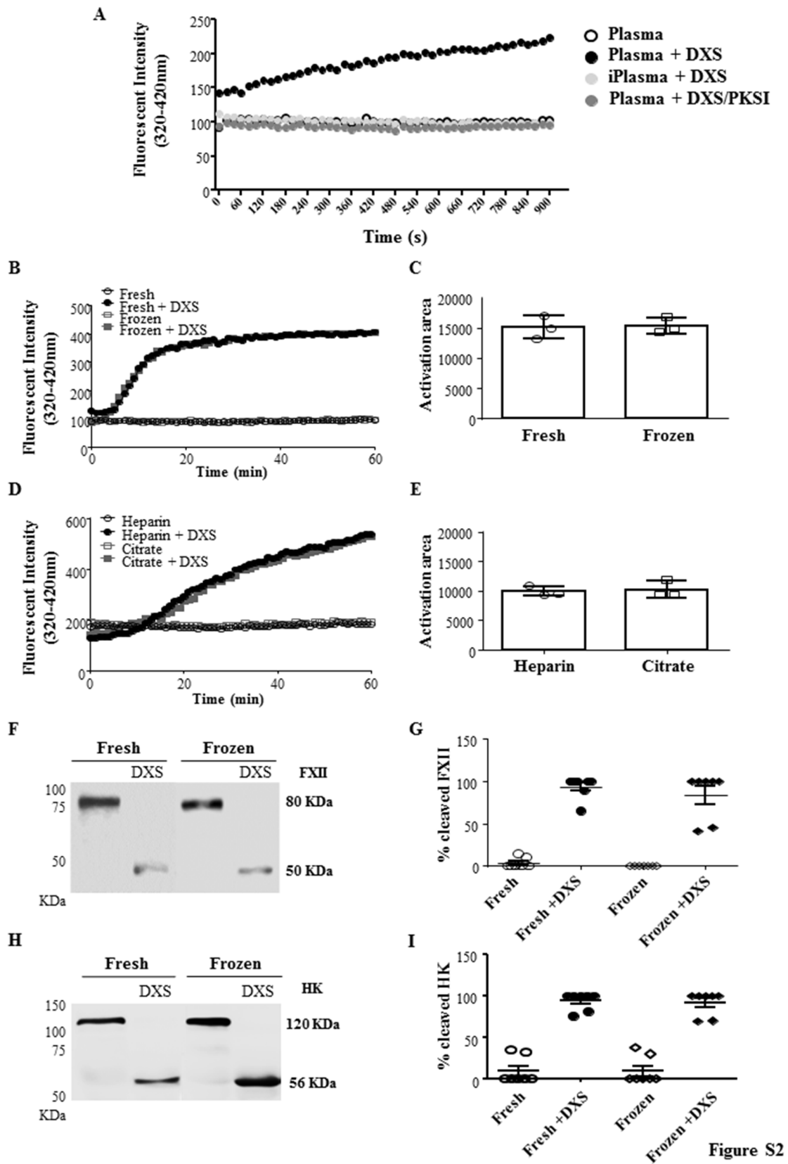
Figure S2. Evaluation of the interference of the plasmas stock condition for the hydrolysis assay.
