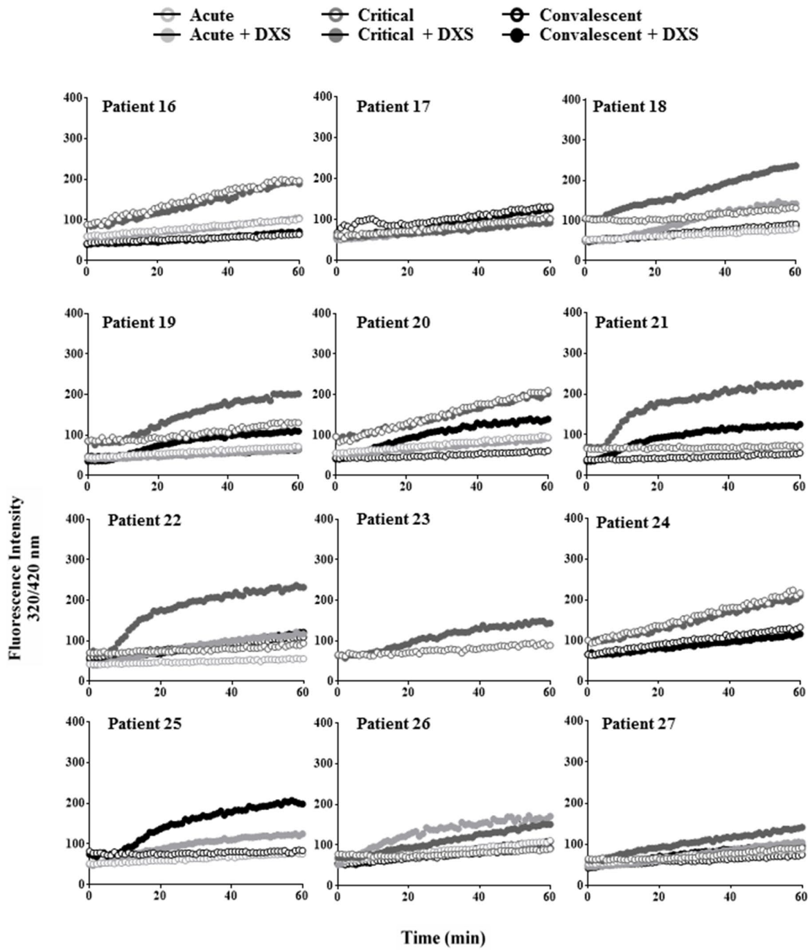
Figure S3. Hydrolysis of all DENV samples at different time points upon the symptom's onset.
