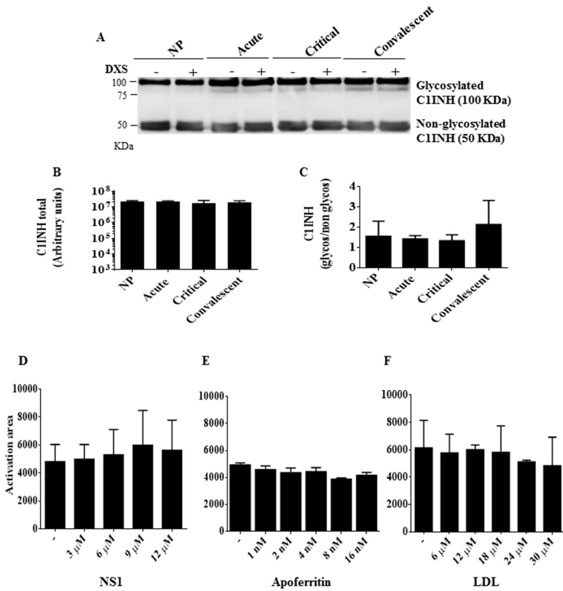
Figure S4. Lower DXS-driven KKS activation in the plasmas from dengue patients is not due to C1inhibitor, NS1, ferritinemia, or increased LDL.
