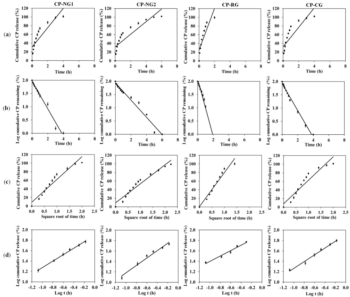
Figure S1: Release kinetics of CP from gel formulations according to (a) zero-order kinetics, (b) first-order kinetics, (c) Higuchi model, and (d) Korsmeyer–Peppas model.
