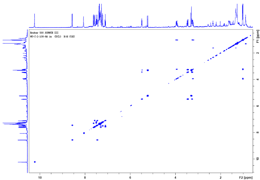
Figure S6. COSY-2 in CDCl 3 for compound 1.
