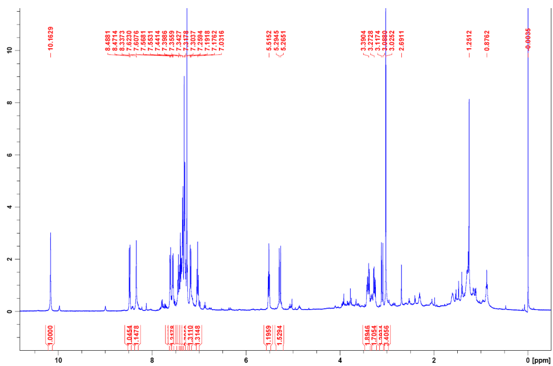
Figure S10. 1 H NMR in CDCl 3 for compound 2.
