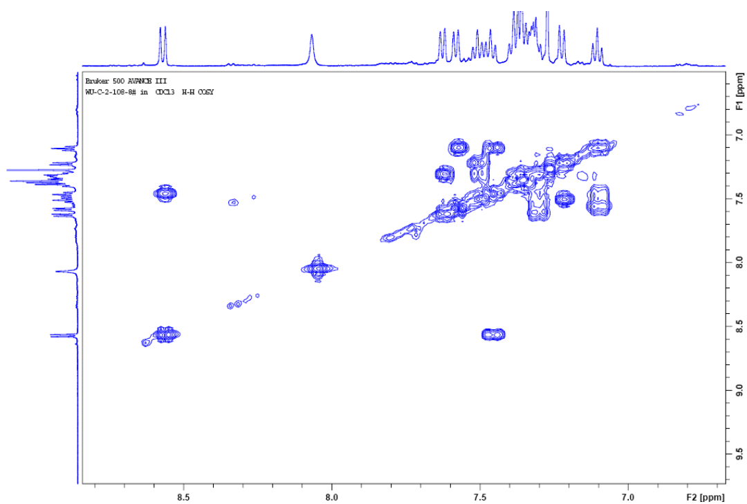
Figure S6. COSY-2 in CDCl 3 for compound 1.
