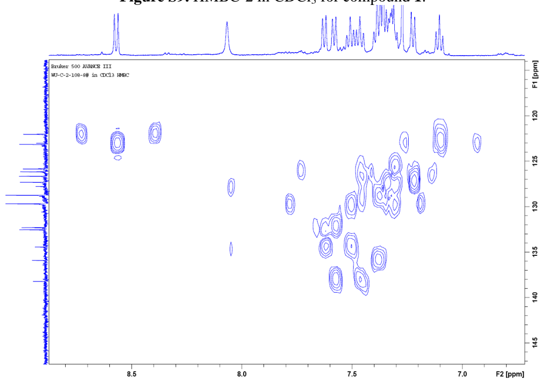
Figure S10. 1 H NMR in CDCl 3 for compound 2.
