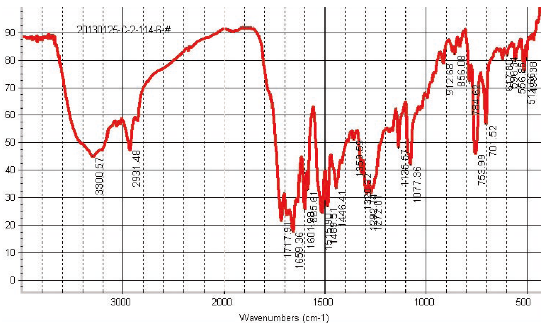
Figure S20. IR for compound 2.
