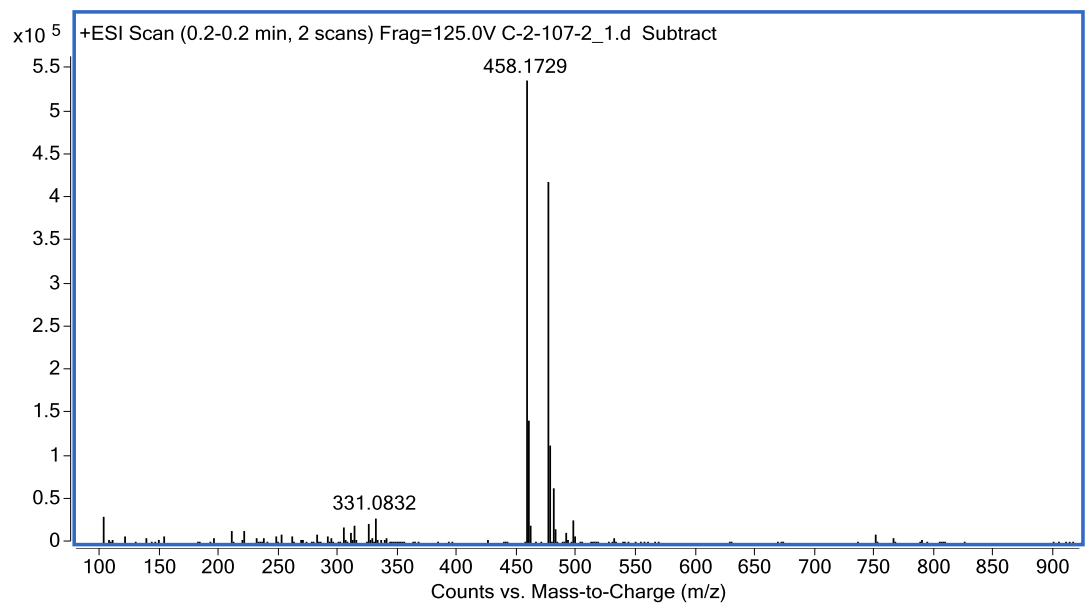
Figure S22. HR-TOF-MS for compound 2.
