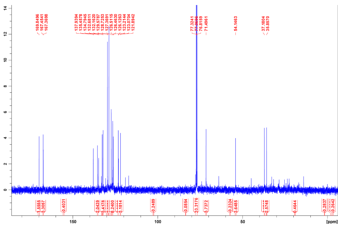
Figure S12. ^{13}\text{C} NMR in \text{CDCl}_3 for compound 2.
