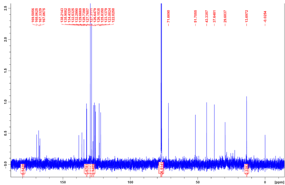
Figure S4. DEPT in \text{CDCl}_3 for compound 1.
