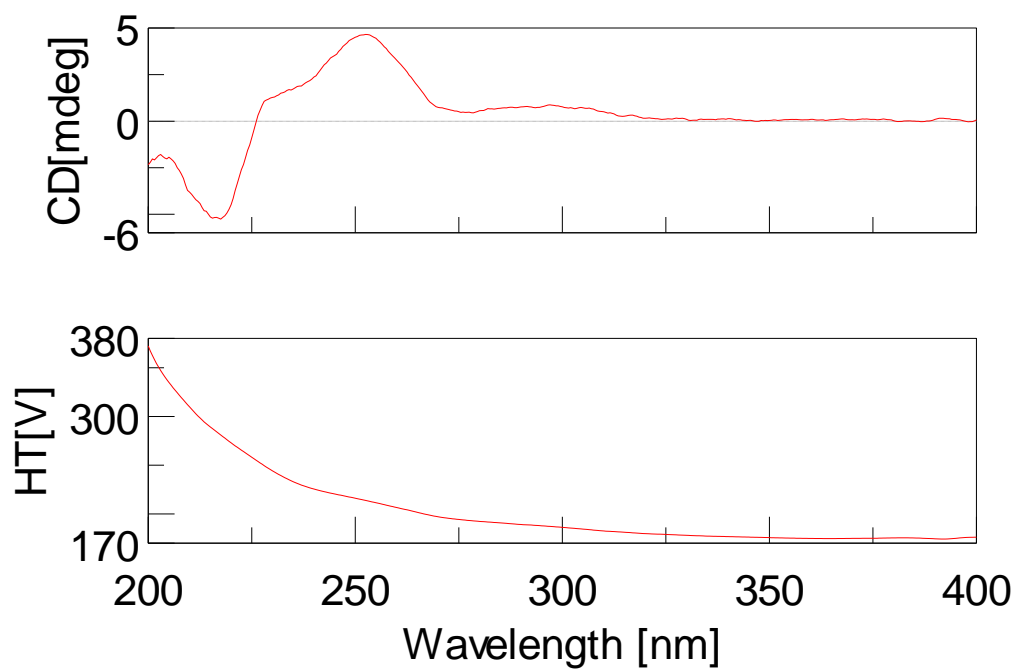
Figure S24. CD for compound 2.
