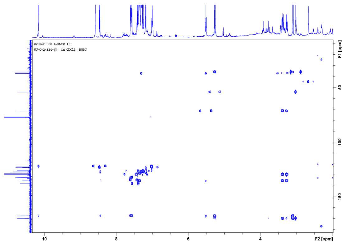
Figure S18. HMBC-2 in CDCl 3 for compound 2.
