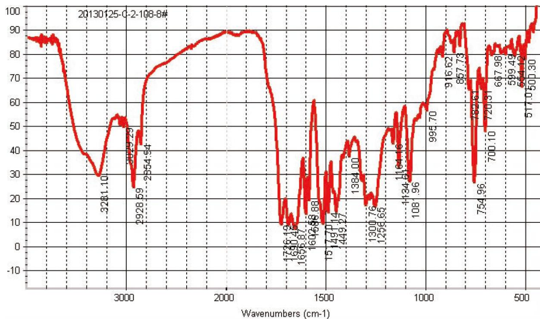
Figure S20. IR for compound 2.
