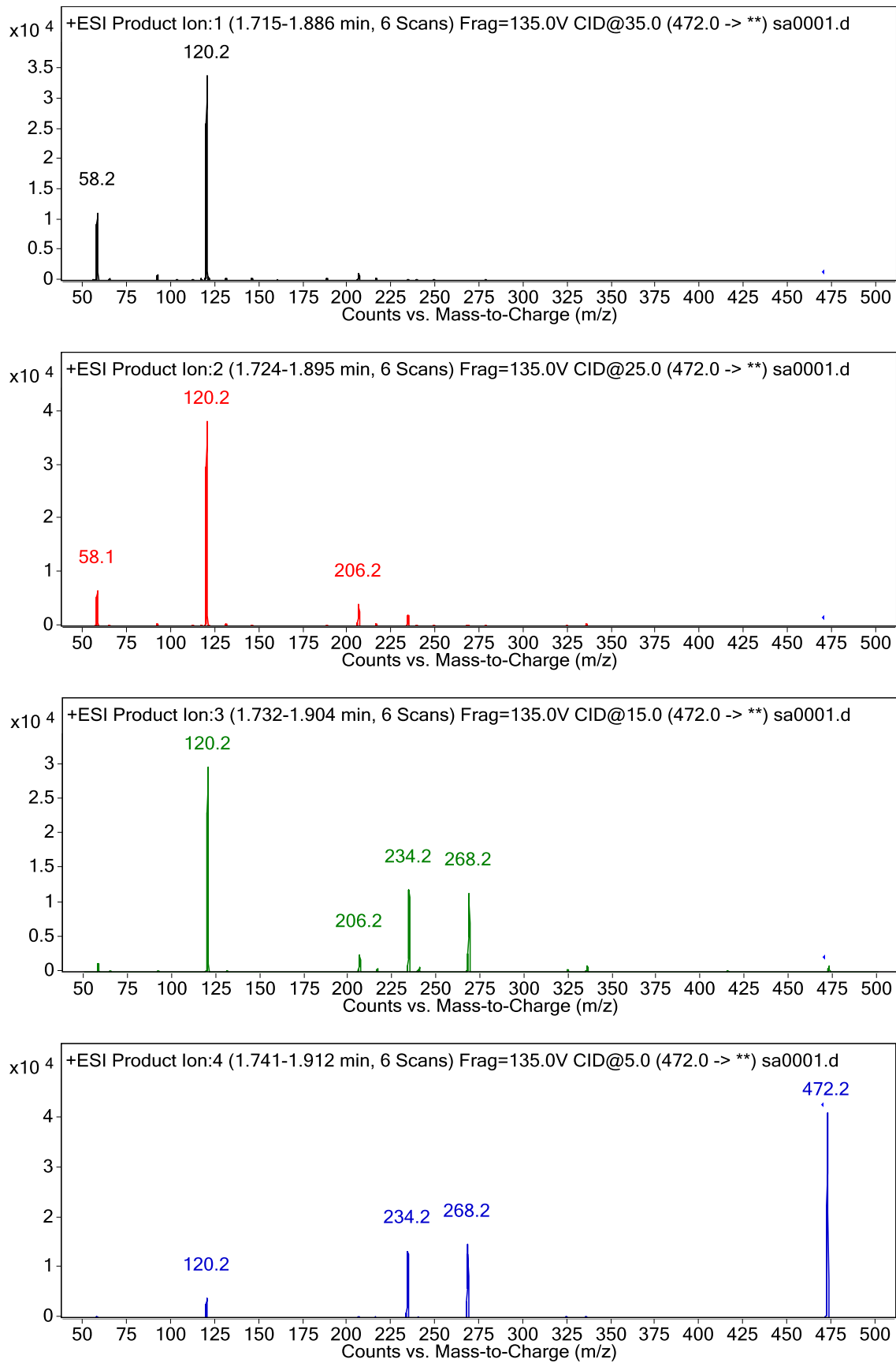
Figure S25. CID for compound 1.
