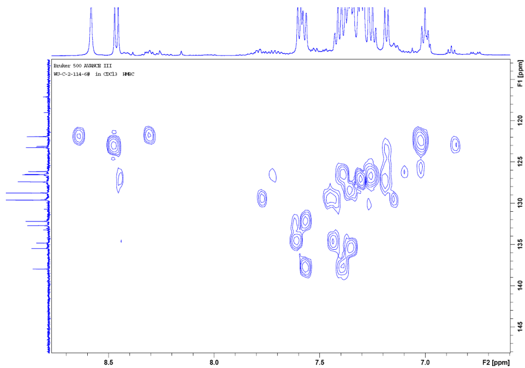
Figure S18. HMBC-2 in CDCl 3 for compound 2.
