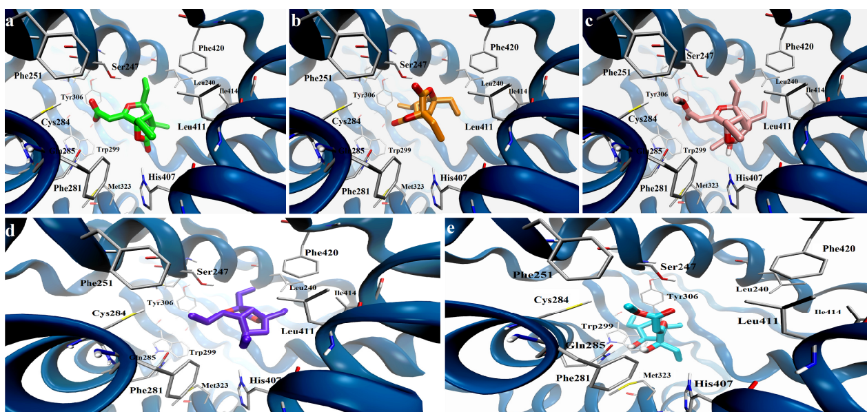
Figure 2. Docking model of gracilioethers 1–5 in the ligand binding domain (LBD) of hPXR (secondary structure represented in blue): (a) 1 (pose n. 4, colored by atom types: C green, O red); (b) 2 (pose n. 27, colored by atom types: C orange, O red); (c) 3 (pose n. 2, colored by atom types: C pink, O red, H light grey); (d) 4 (pose n. 11, colored by atom types: C violet, O red); (e) 5 (pose n. 1, colored by atom types: C cyan, O red, H light grey).
