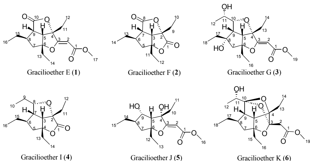
Figure 1. Gracilioethers from the sponge Plakinastrella mamillaris .
