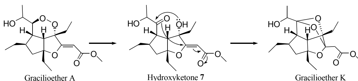
Figure 4. Biosynthetic pathway to gracilioether K, involving endoperoxy rearrangement, hemiacetal formation and Michael-type attack on the \alpha,\beta -unsaturated ester group.
