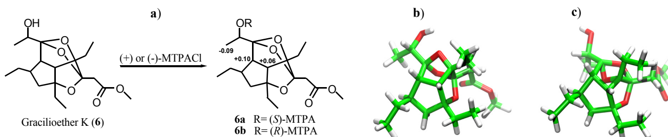
Figure 5. (a) \Delta\delta_{S-R} values (ppm) of MTPA esters 6a and 6b ; 3D model for (b) 10 R configuration and (c) 10 S configuration.
