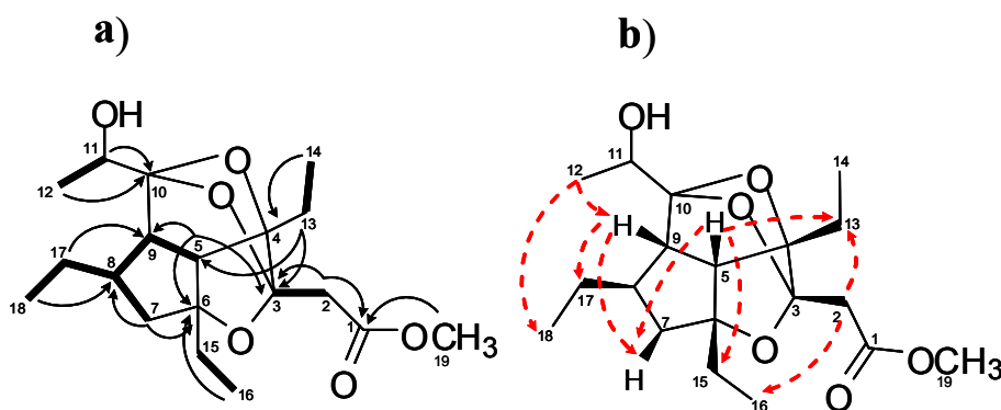
Figure 3. (a) COSY connectivities (bold bonds), and key HMBC (black arrows) correlations; (b) Key ROE (red dashed arrows) correlations for gracilioether K ( 6 ).
