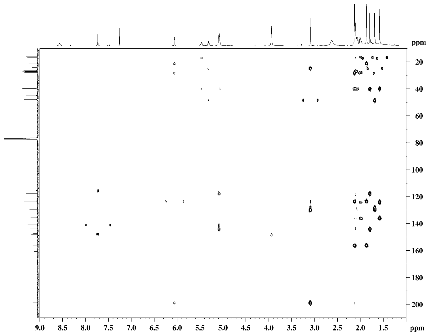
Figure S11. HMBC spectrum of Malonganenone M (2).
