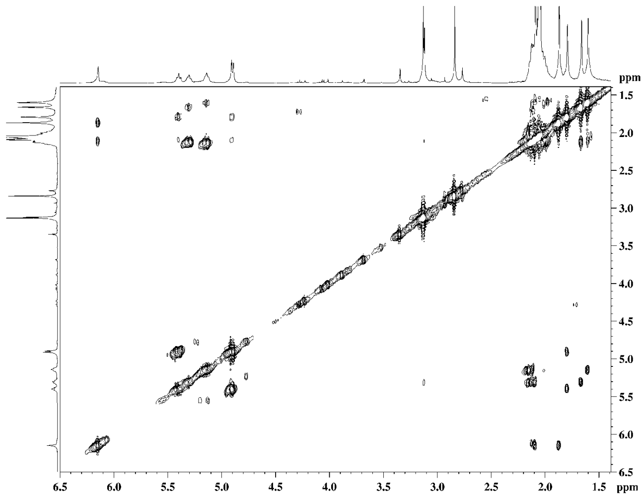
Figure S25. ^1\text{H} - ^1\text{H} COSY spectrum of Malonganenone P (5).
