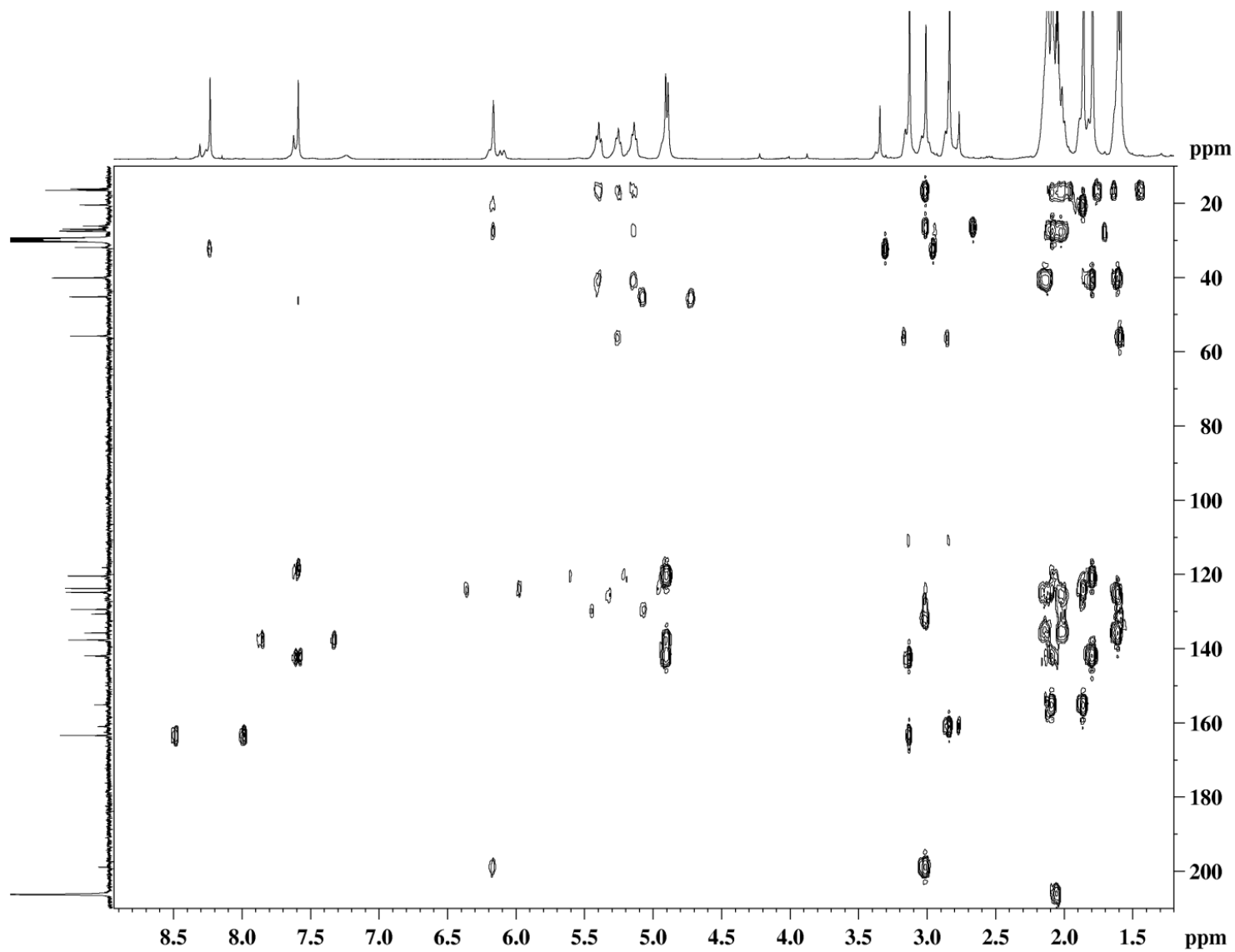
Figure S21. HMBC spectrum of Malonganenone O (4).
