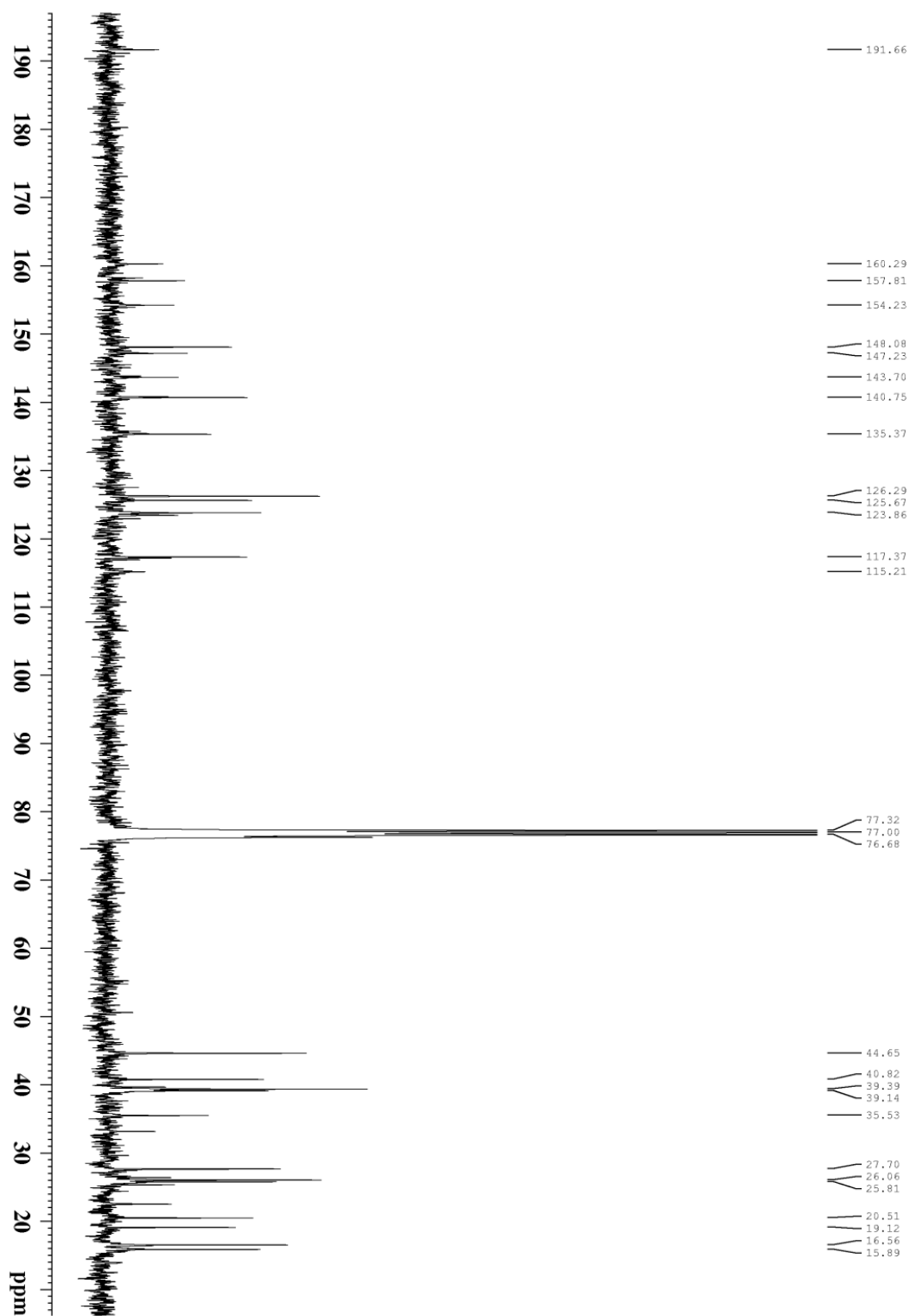
Figure S13. ^{13}\text{C} NMR spectrum of Malonganenone N (3).
