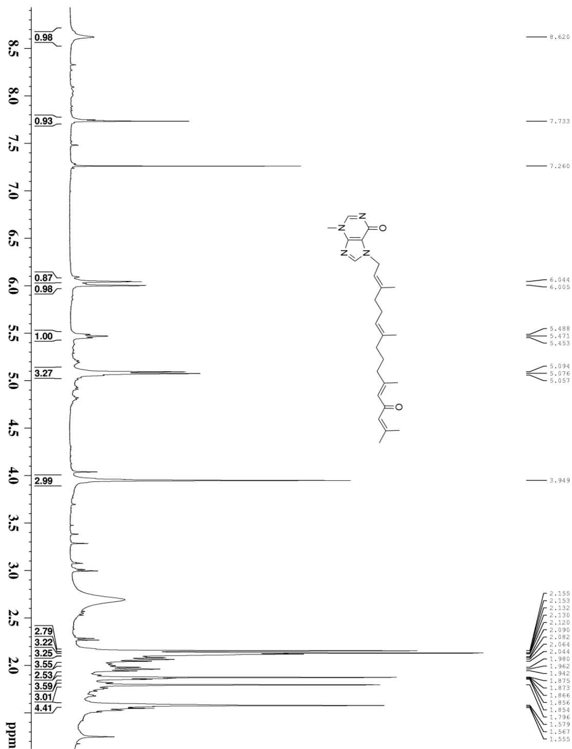
Figure S12. 1 H NMR spectrum of Malonganenone N (3).
