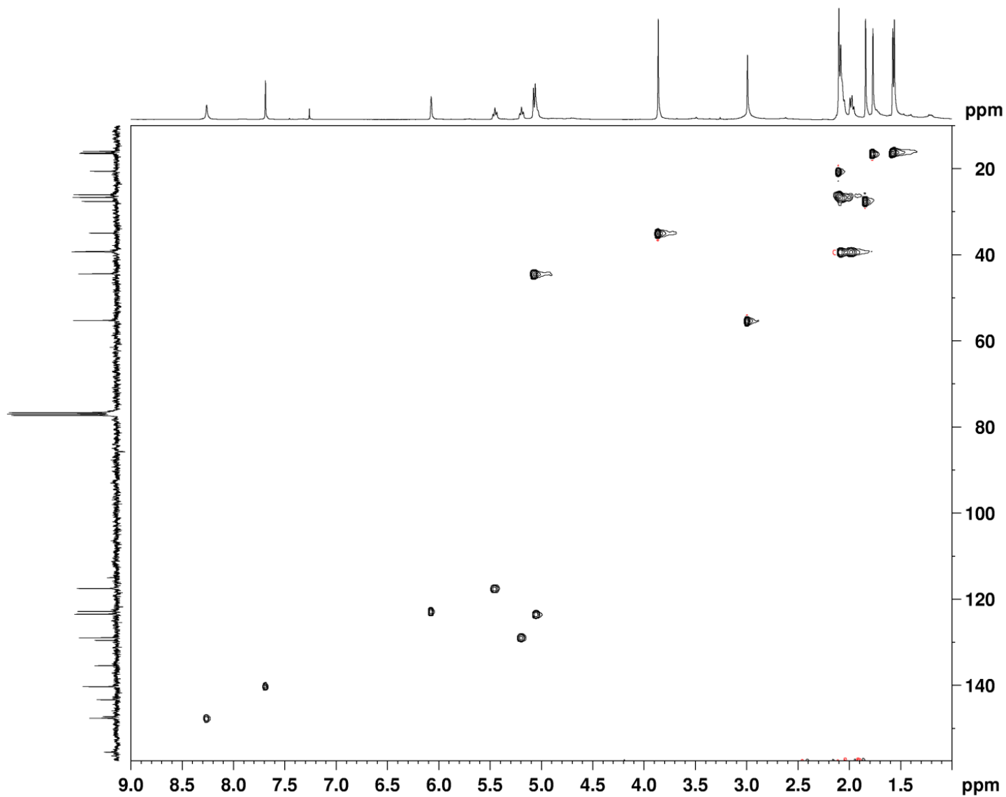
Figure S3. HSQC Spectrum of Malonganenone L (1).
