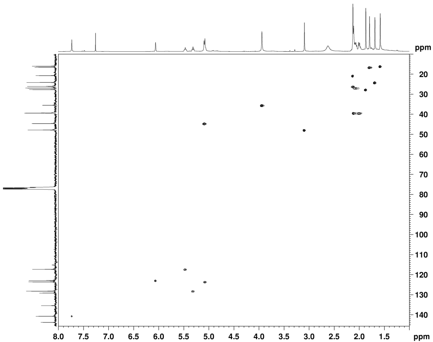
Figure S9. HSQC Spectrum of Malonganenone M (2).
