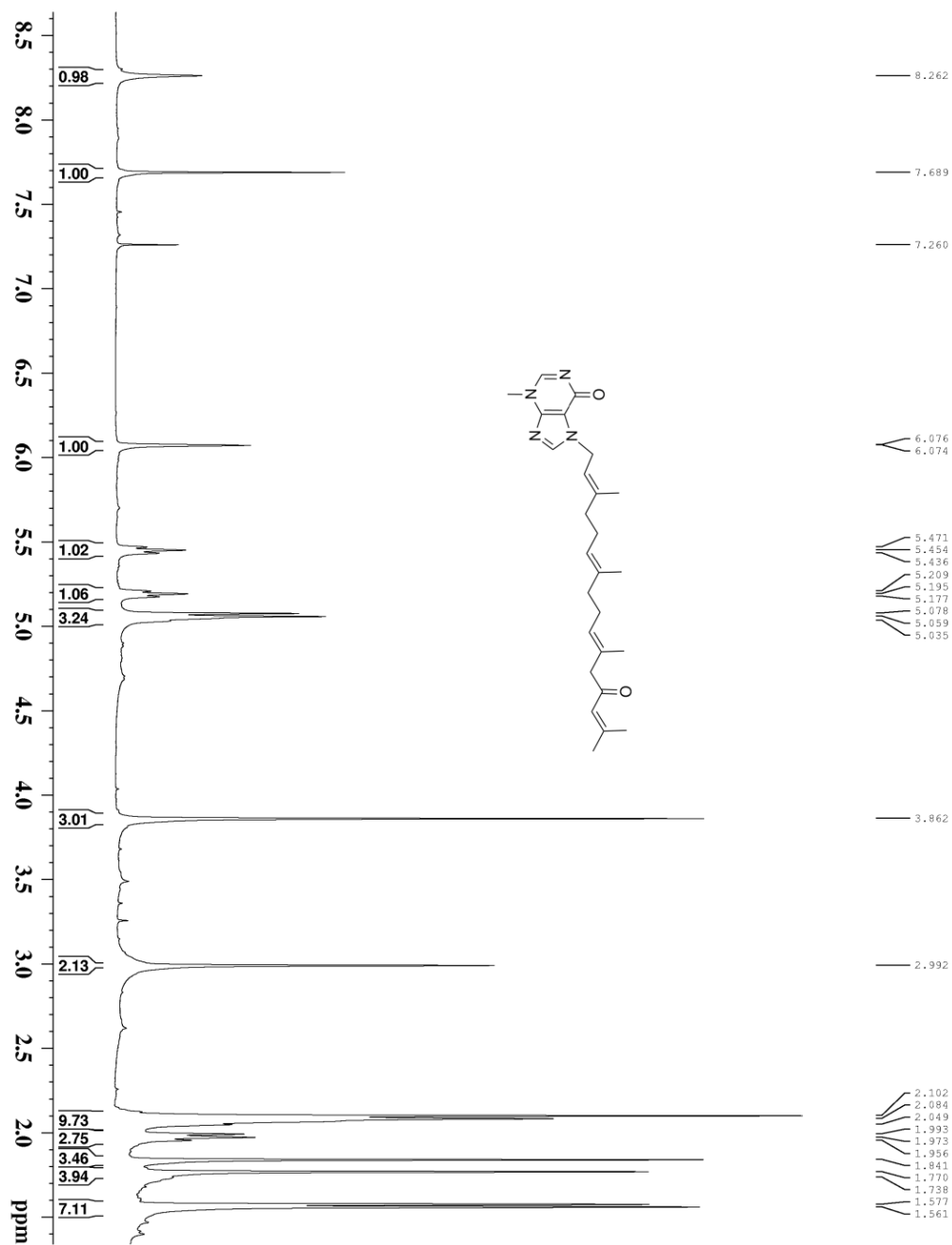
Figure S1. ^1\text{H} NMR spectrum of Malonganenone L (1).
