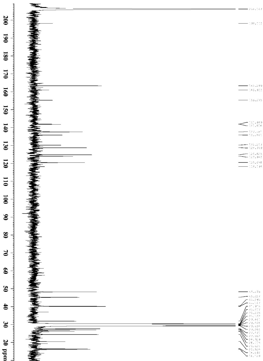
Figure S23. 13 C NMR spectrum of Malonganenone P (5).
