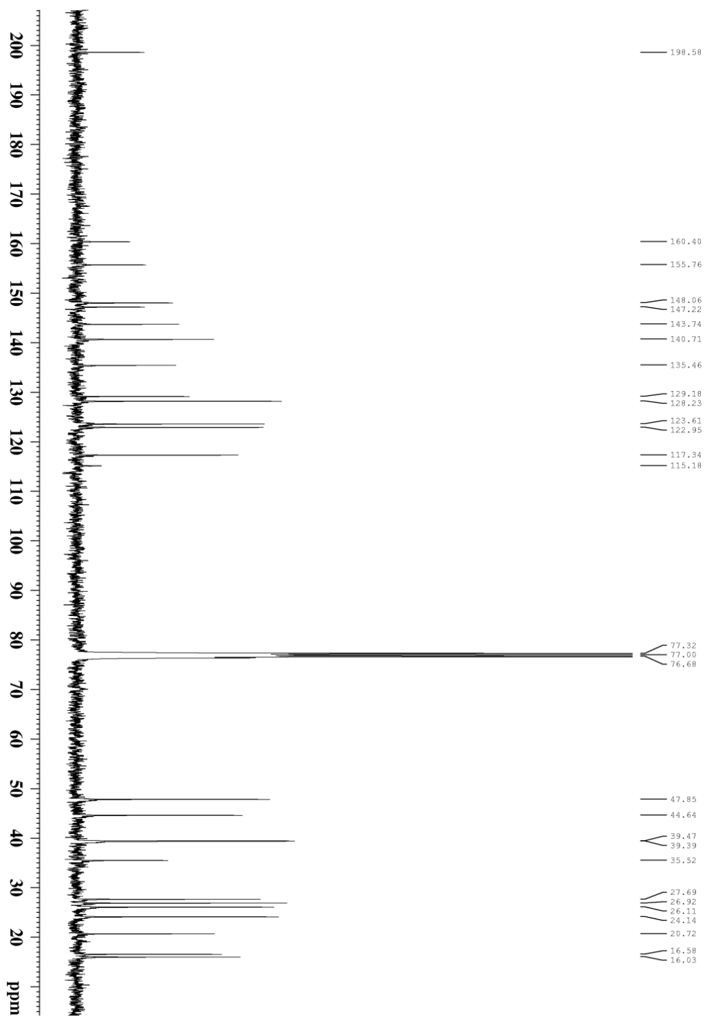
Figure S8. ^{13}\text{C} NMR spectrum of Malonganenone M (2).
