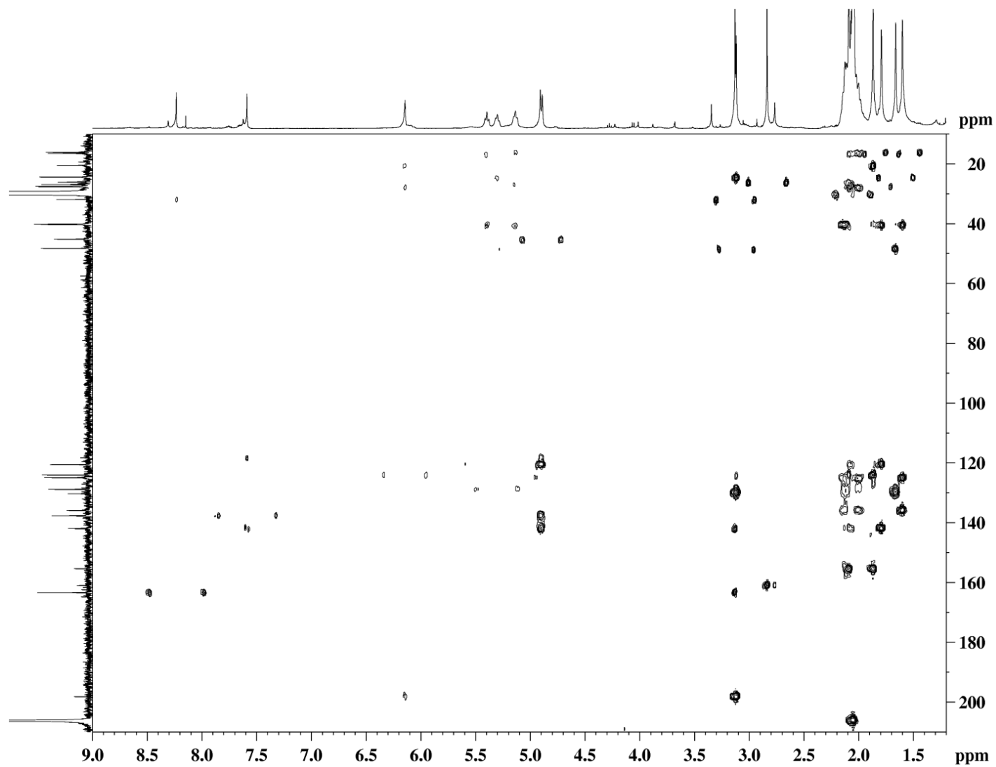
Figure S26. HMBC spectrum of Malonganenone P (5).
