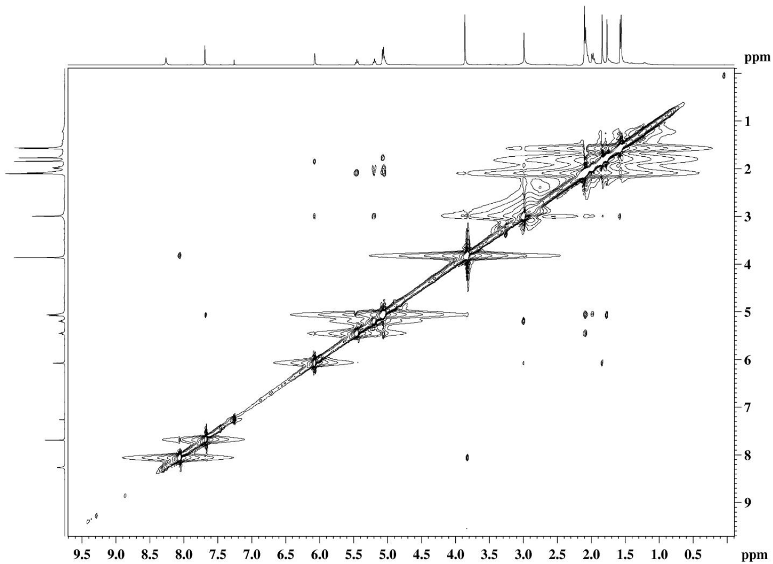
Figure S6. NOESY spectrum of Malonganenone L (1).
