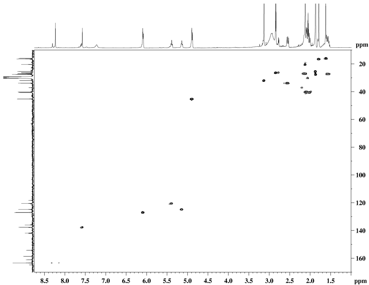
Figure S29. HSQC Spectrum of Malonganenone Q (6).
