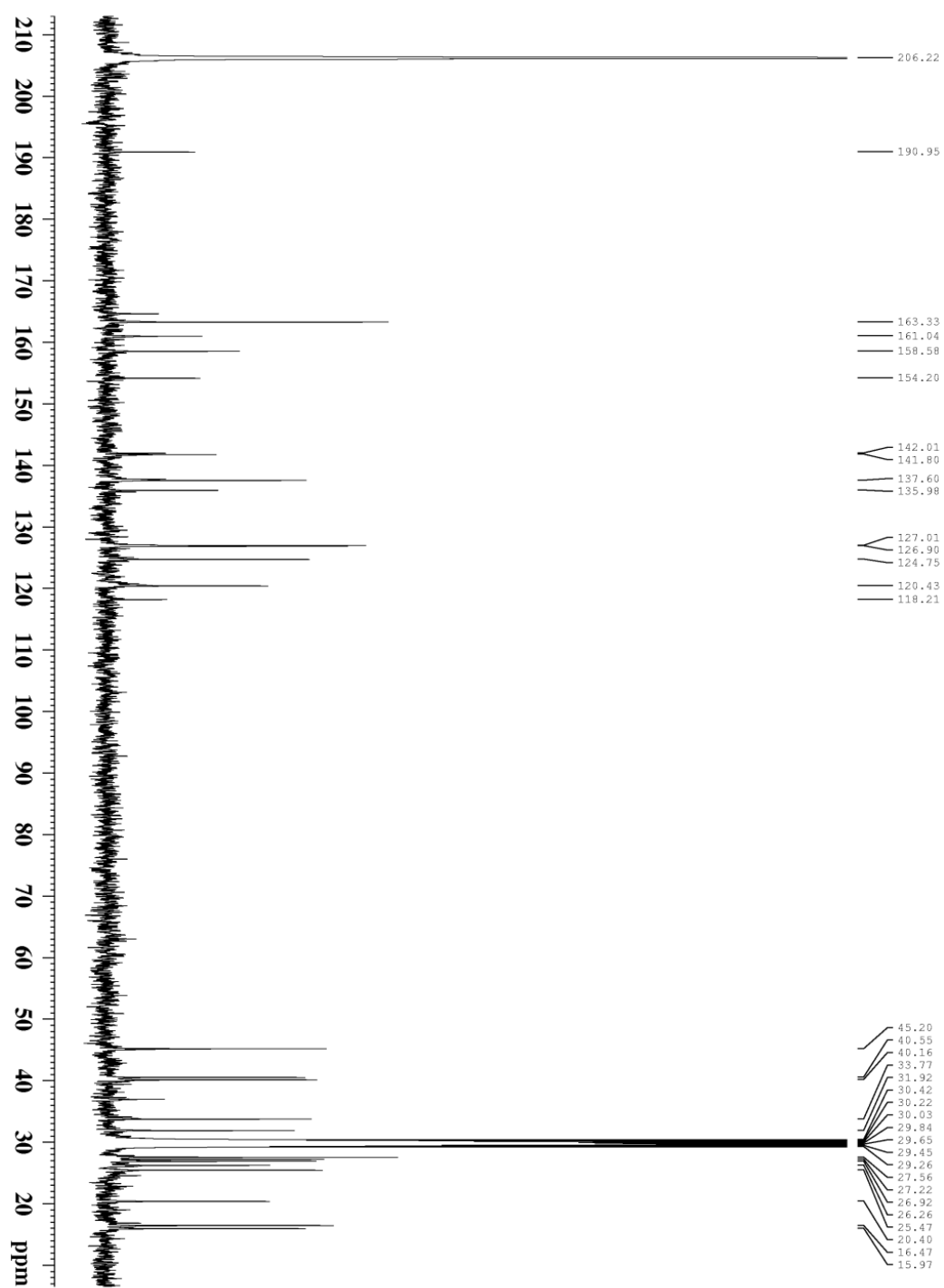
Figure S28. ^{13}\text{C} NMR spectrum of Malonganenone Q (6).
