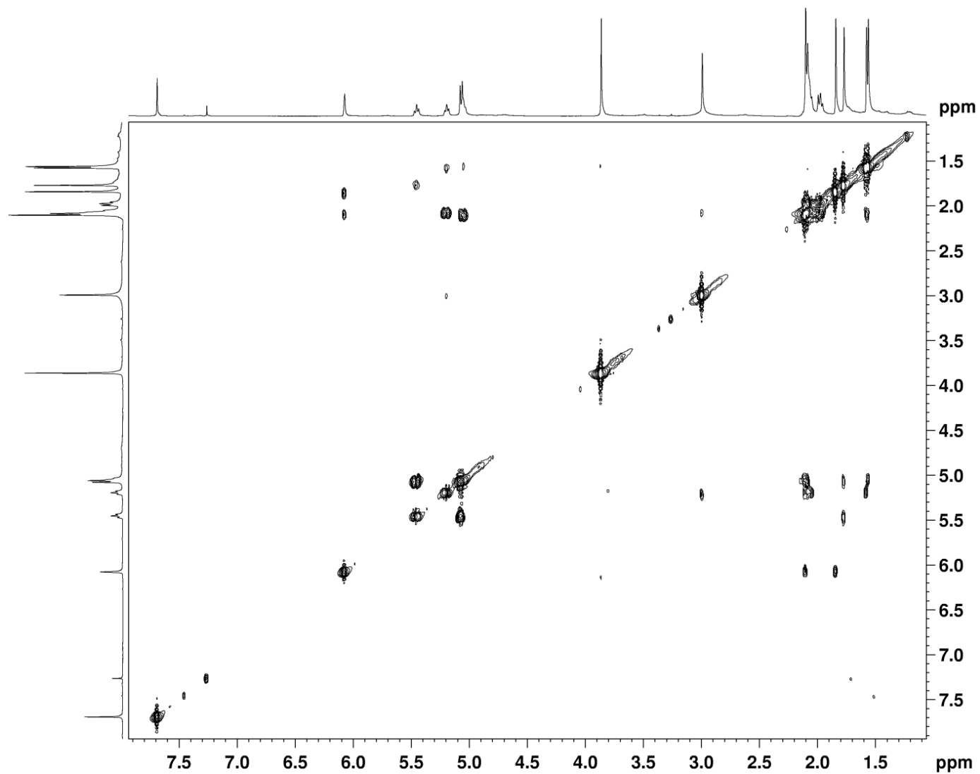
Figure S4. ^1\text{H} - ^1\text{H} COSY spectrum of Malonganenone L (1).
