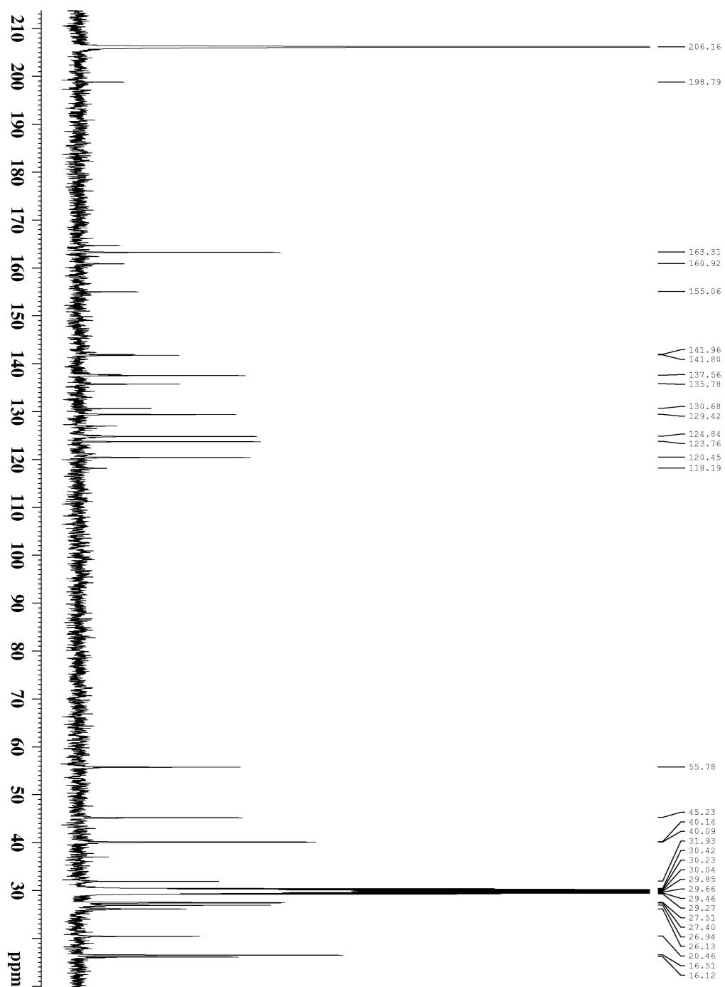
Figure S18. ^{13}\text{C} NMR spectrum of Malonganenone O (4).
