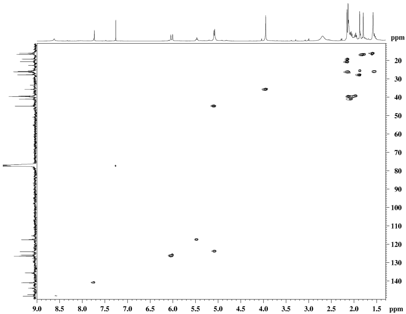
Figure S14. HSQC Spectrum of Malonganone N (3).
