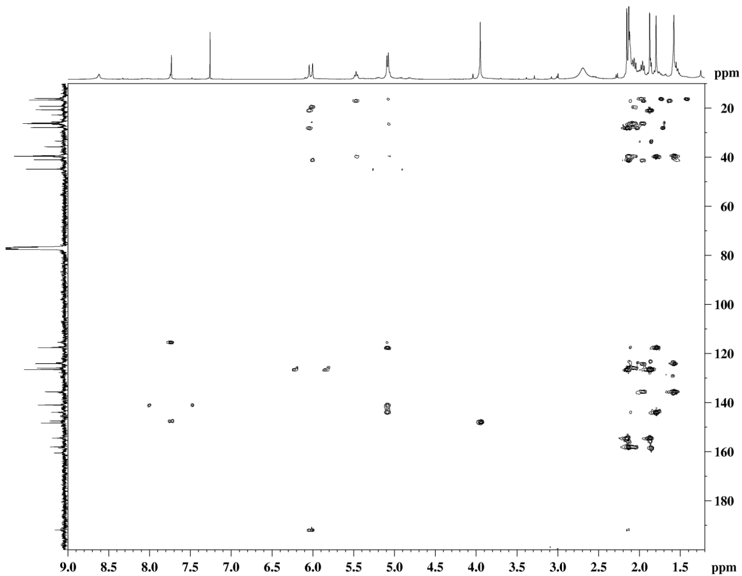
Figure S16. HMBC spectrum of Malonganenone N (3).
