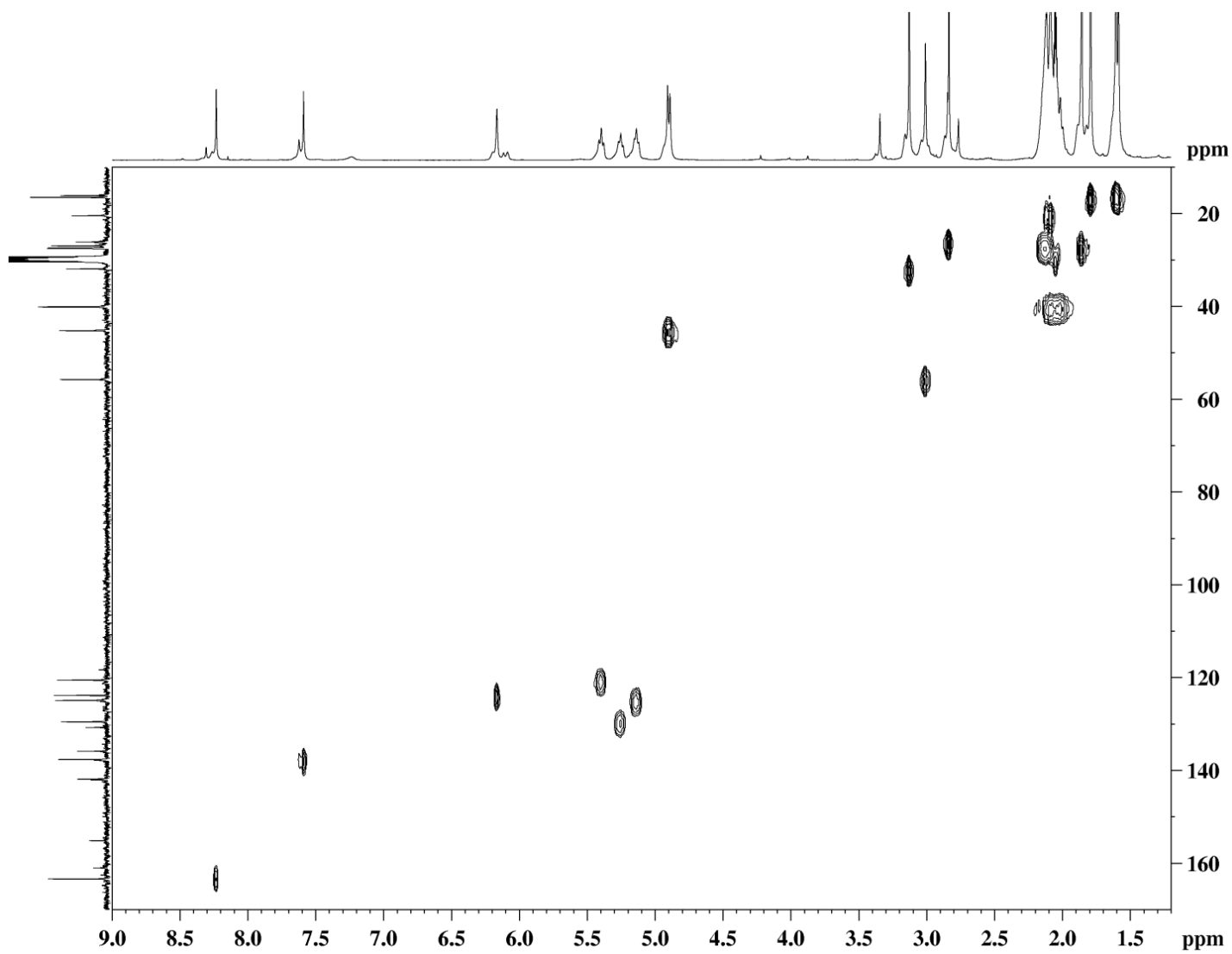
Figure S19. HSQC Spectrum of Malonganenone O (4).
