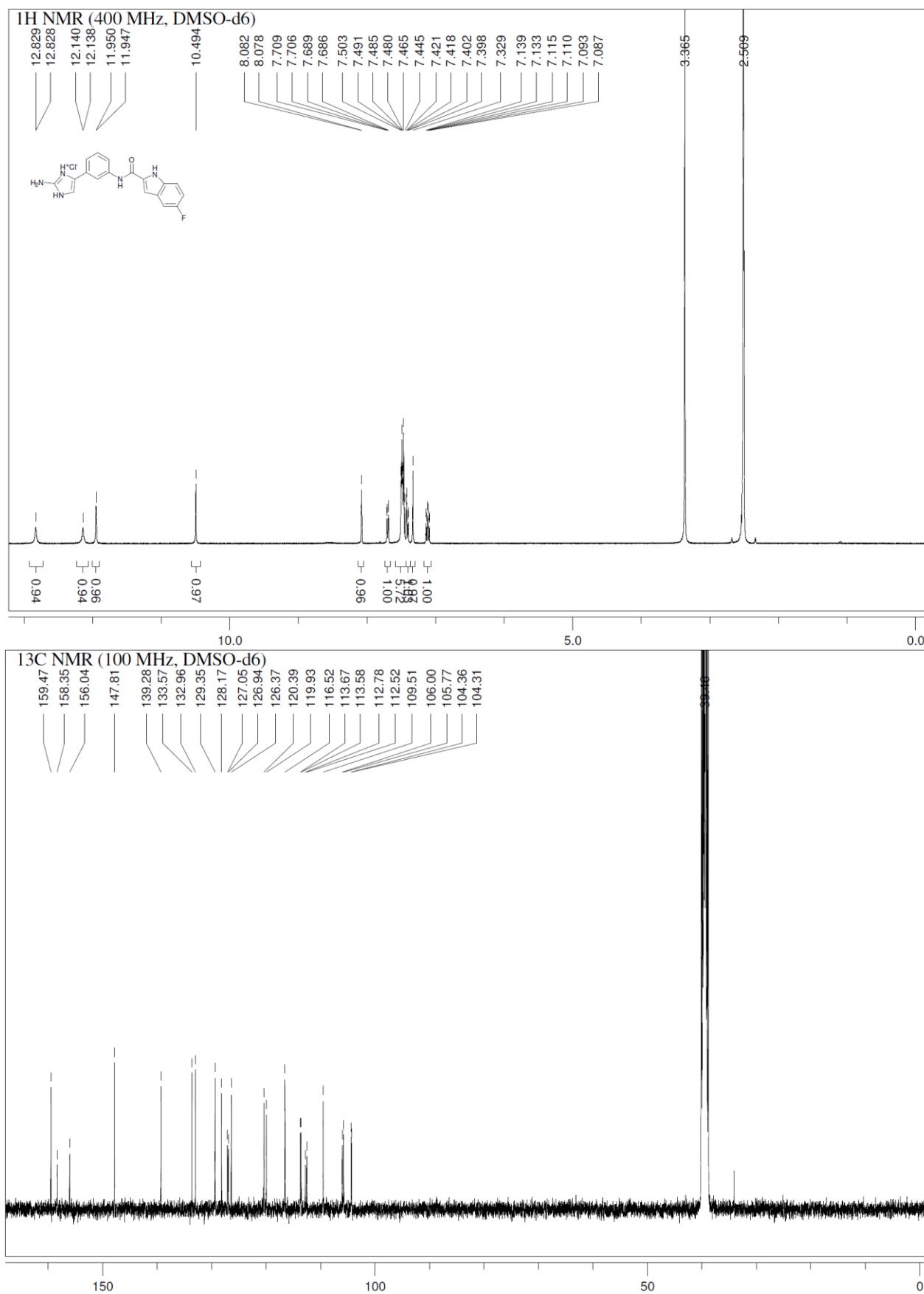
Figure S15. 2-Amino-4-(3-(5-fluoro-1 H -indole-2-carboxamido)phenyl)-1 H -imidazol-3-ium chloride ( 6j ).
