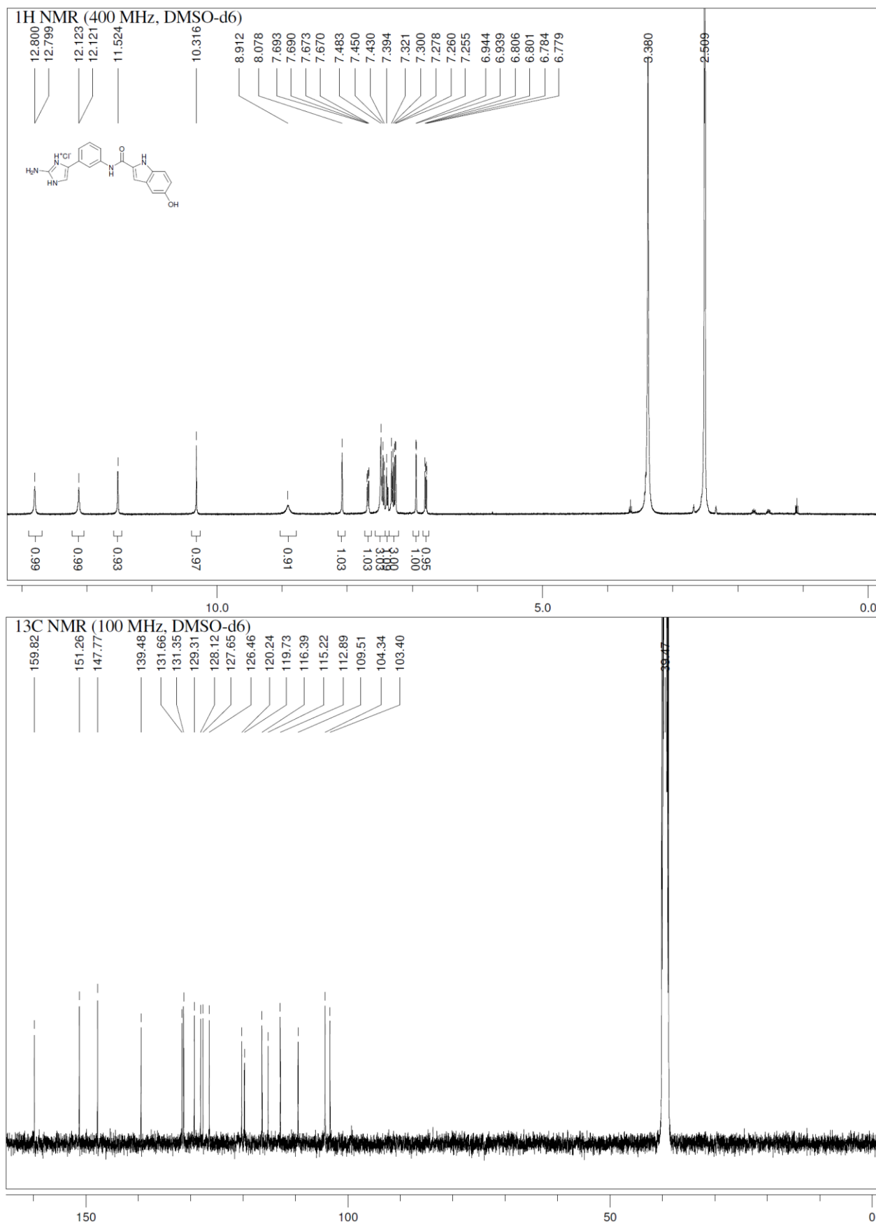
Figure S18. 2-Amino-4-(3-(5-hydroxy-1 H -indole-2-carboxamido)phenyl)-1 H -imidazol-3-ium chloride ( 8 ).
