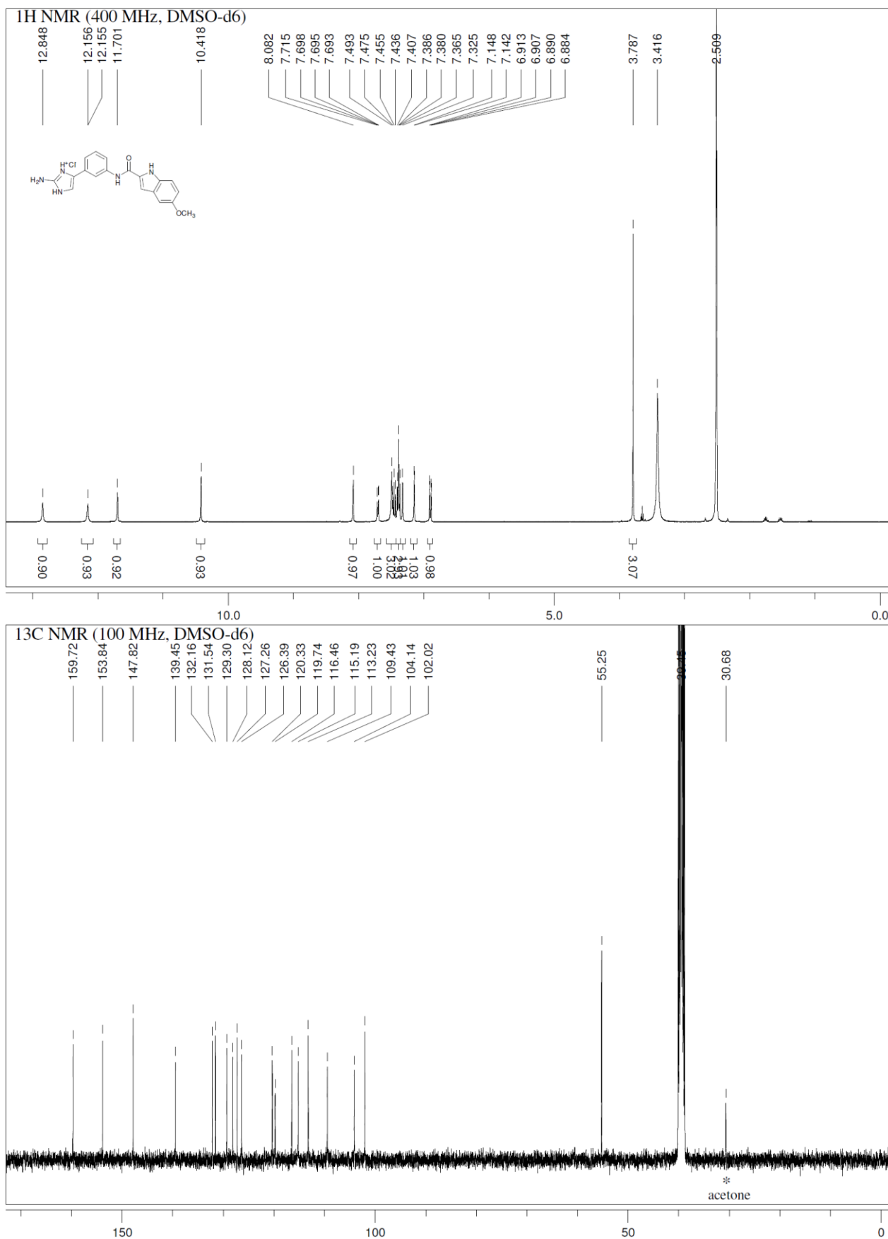
Figure S11. 2-Amino-4-(3-(5-methoxy-1H-indole-2-carboxamido)phenyl)-1H-imidazol-3-ium chloride ( 6f ).
