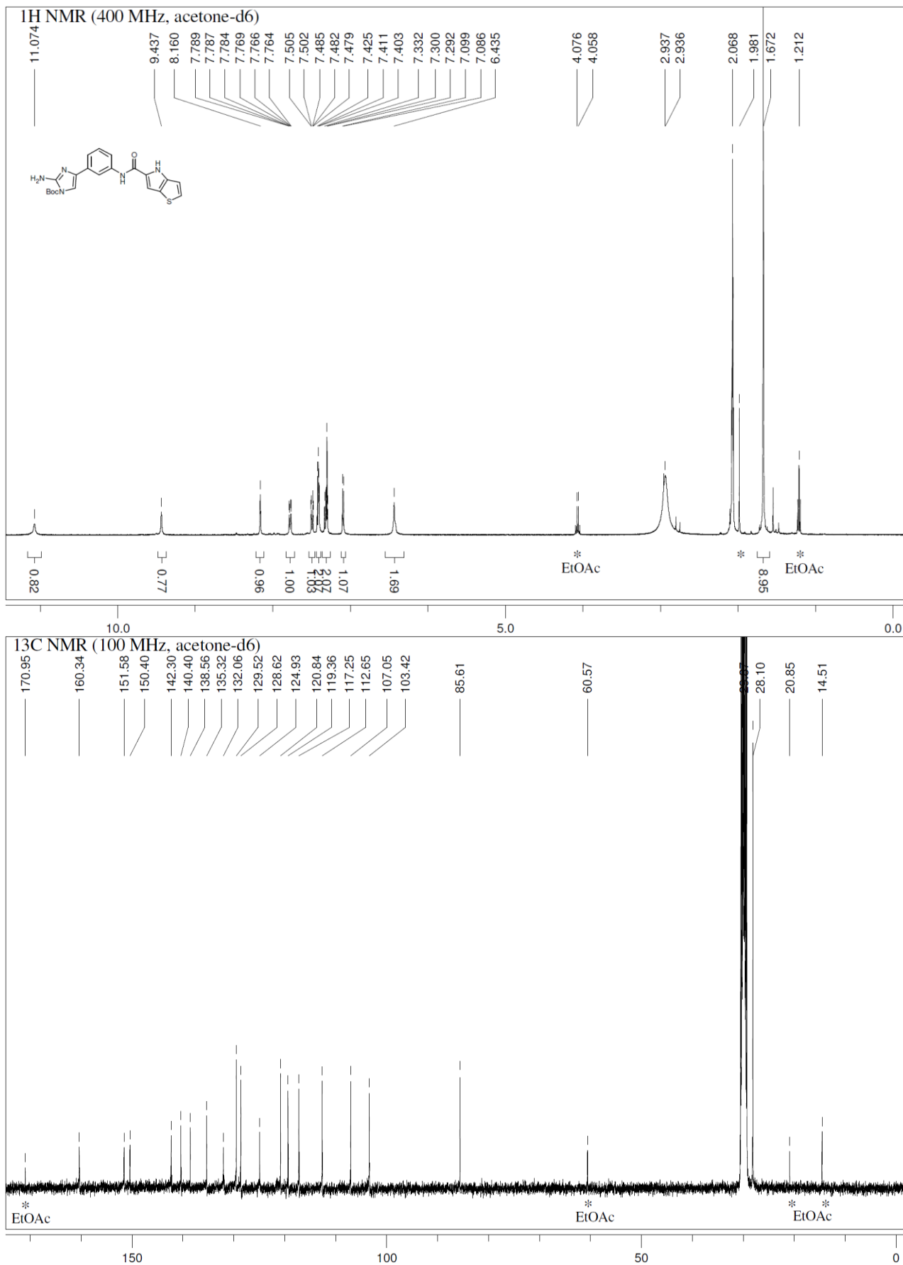
Figure S10. tert -Butyl 4-(3-(4 H -thieno[3,2- b ]pyrrole-5-carboxamido)phenyl)-2-amino-1- H -imidazole-1-carboxylate ( 5k ).
