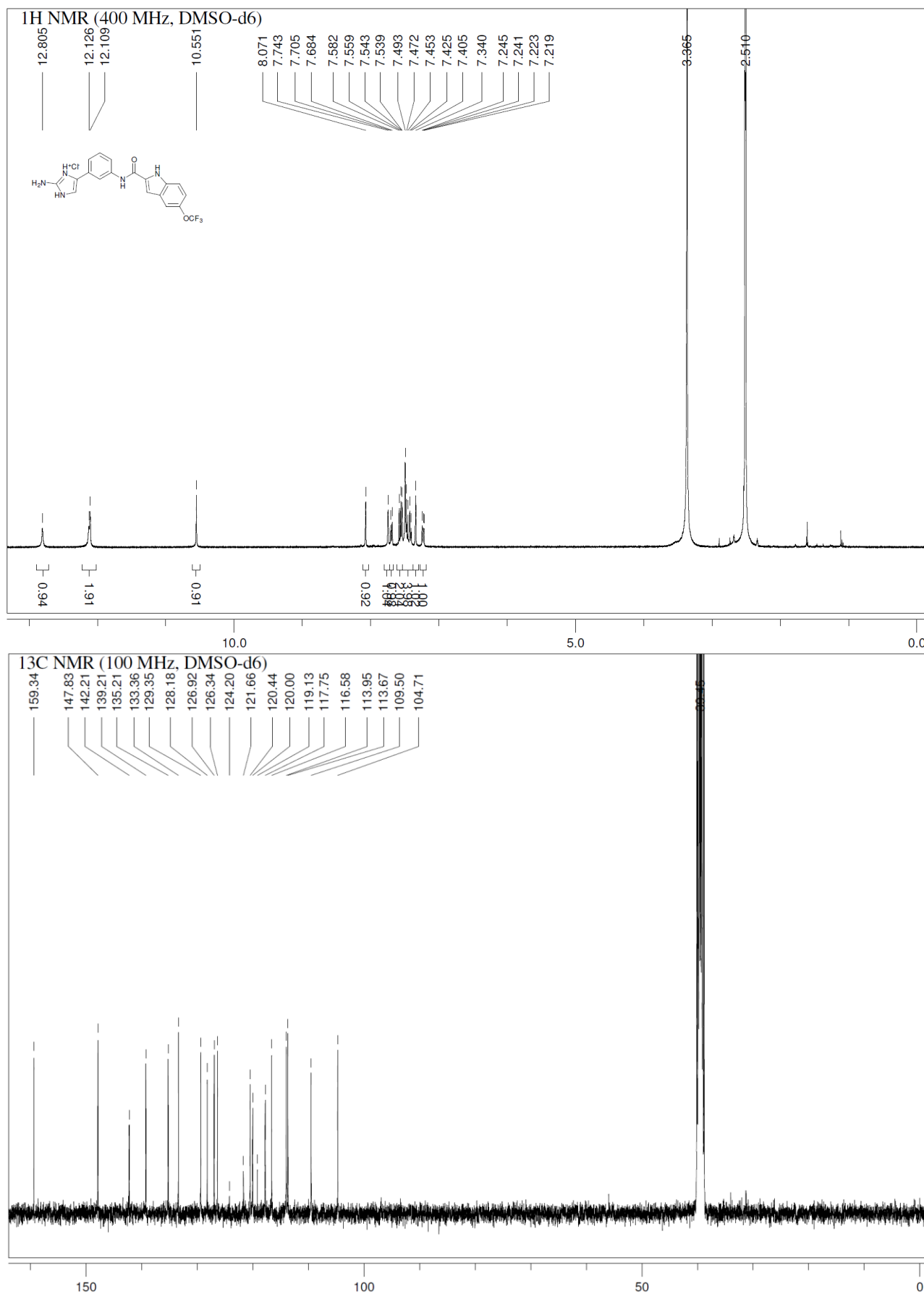
Figure S12. 2-Amino-4-(3-(5-(trifluoromethoxy)-1 H -indole-2-carboxamido)phenyl)-1 H -imidazol-3-ium chloride ( 6g ).
