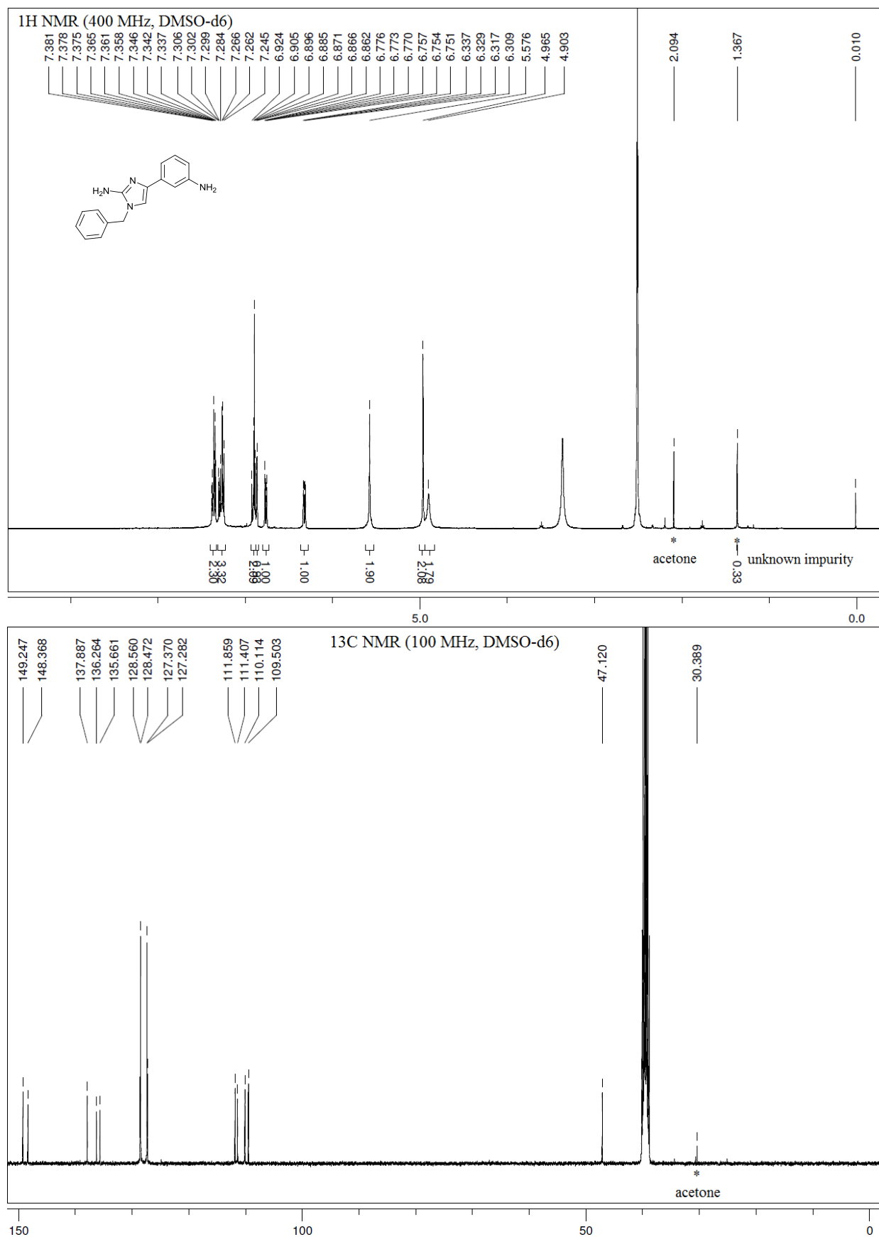
Figure S20. 4-(3-Aminophenyl)-1-benzyl-1H-imidazol-2-amine (14).
