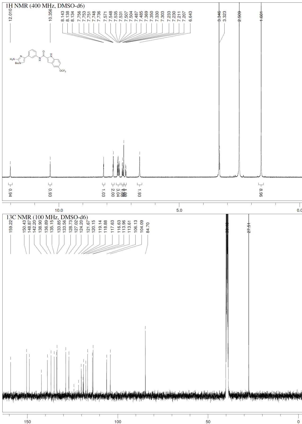
Figure S6. tert -Butyl 2-amino-4-(3-(5-(trifluoromethoxy)-1 H -indole-2-carboxamido)phenyl)-1 H -imidazole-1-carboxylate ( 5g ).
