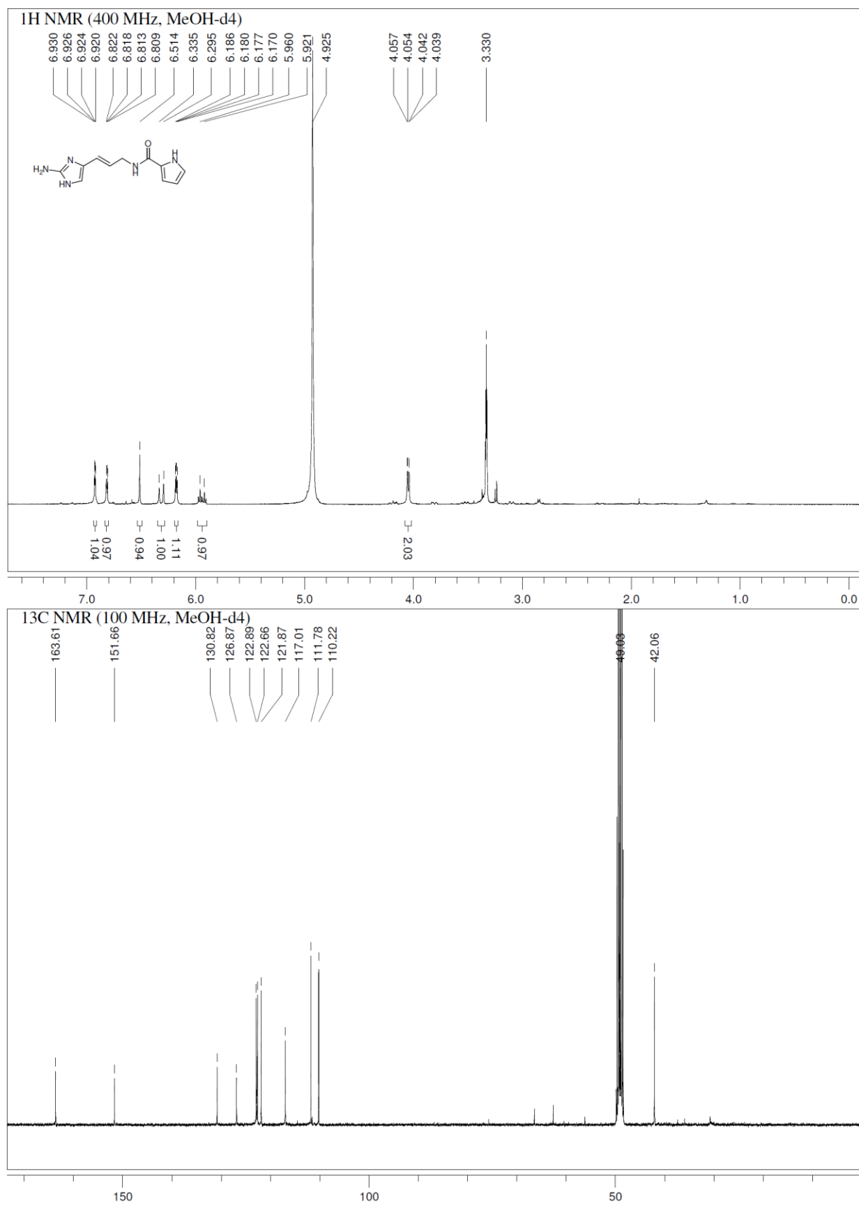
Figure S1. ( E )- N -(3-(2-amino-1 H -imidazol-4-yl)allyl)-1 H -pyrrole-2-carboxamide ( 2a ).
