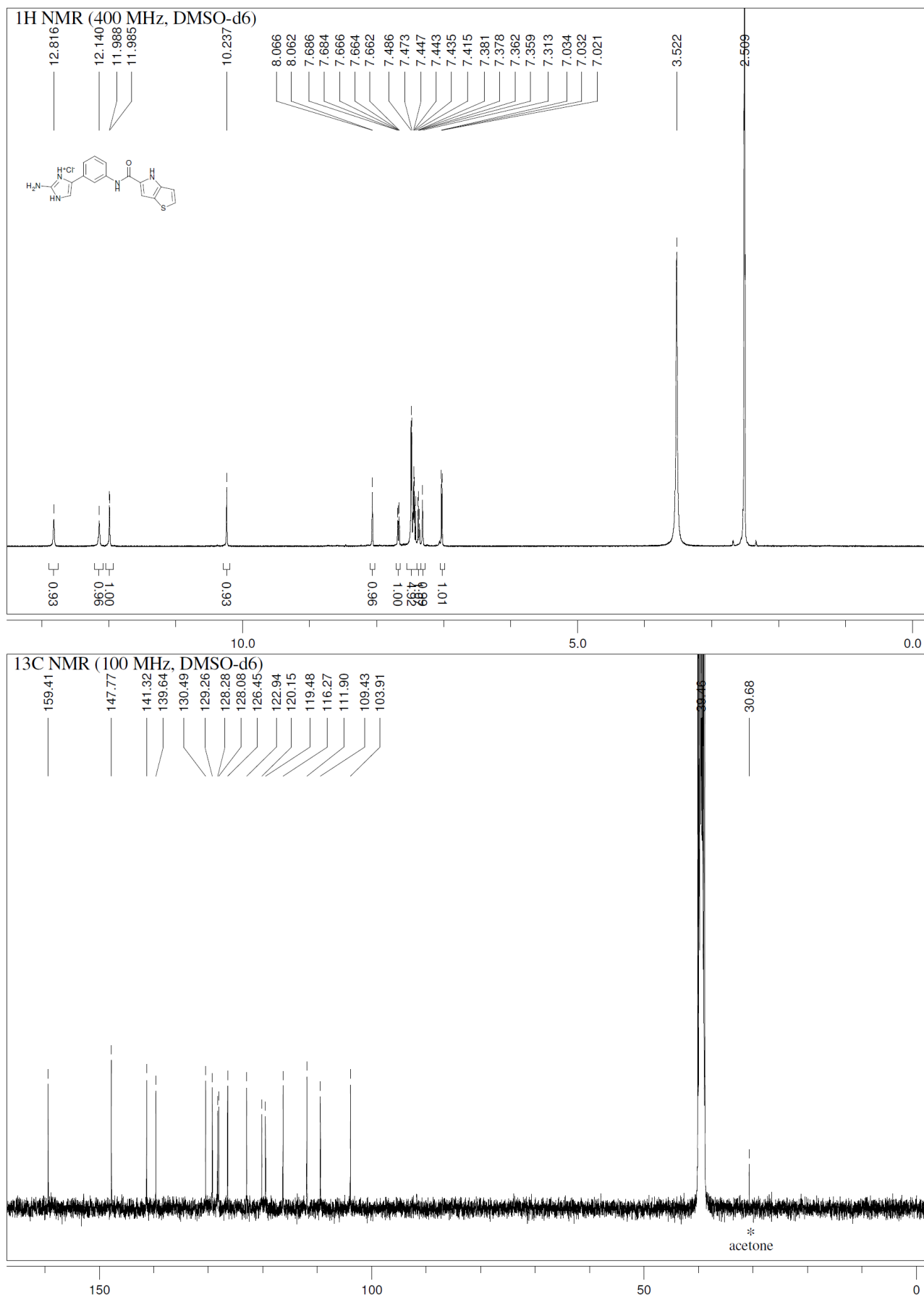
Figure S16. 4-(3-(4 H -Thieno[3,2- b ]pyrrole-5-carboxamido)phenyl)-2-amino-1 H -imidazol-3-ium chloride ( 6k ).
