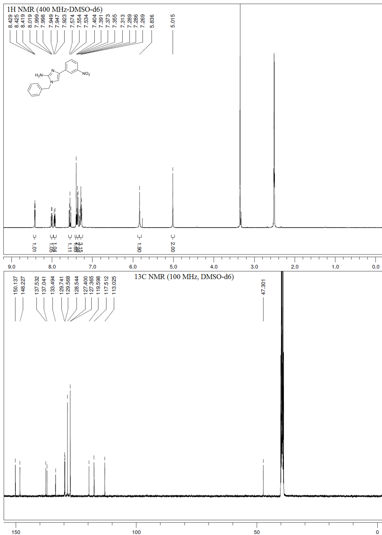
Figure S19. 1-Benzyl-4-(3-nitrophenyl)-1H-imidazol-2-amine (13).
