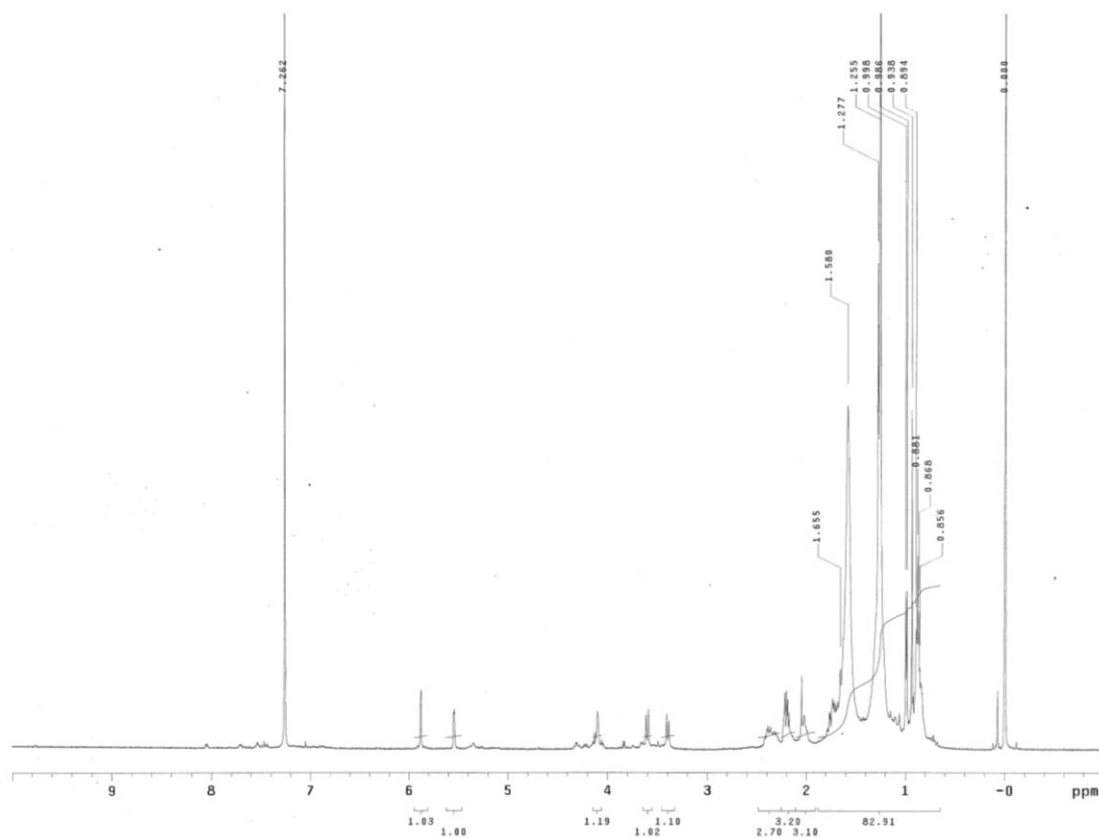
Figure S4. ^{13}\text{C} NMR spectrum of 2 in \text{CDCl}_3 .
