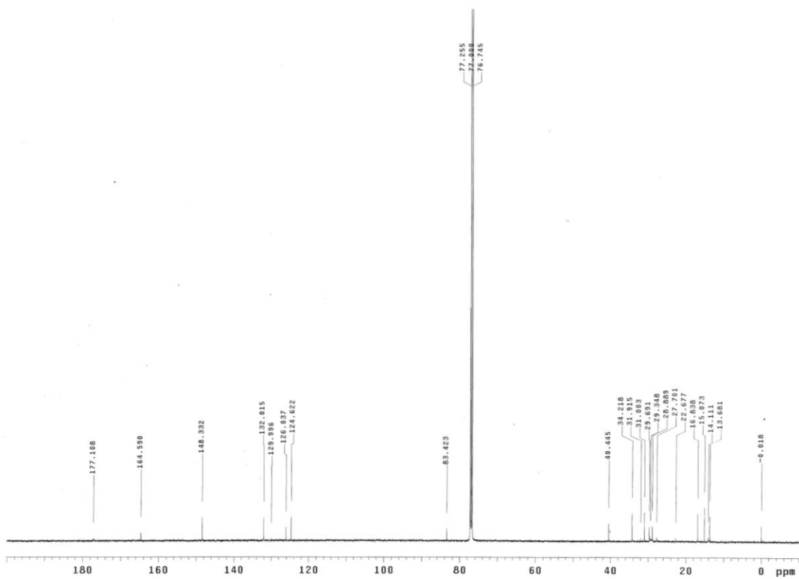
Figure S6. ^{13}\text{C} NMR spectrum of 3 in \text{CDCl}_3 .
