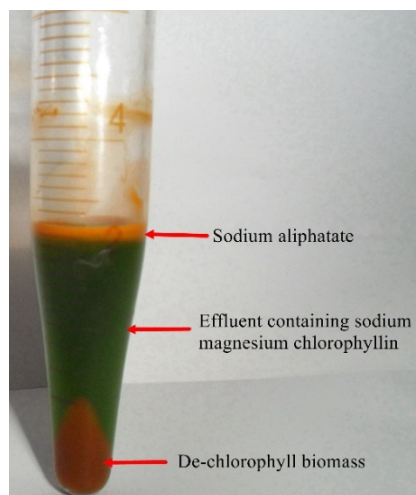
Figure S1. Biomass treated with saponification reagent (ethanol-NaOH).
