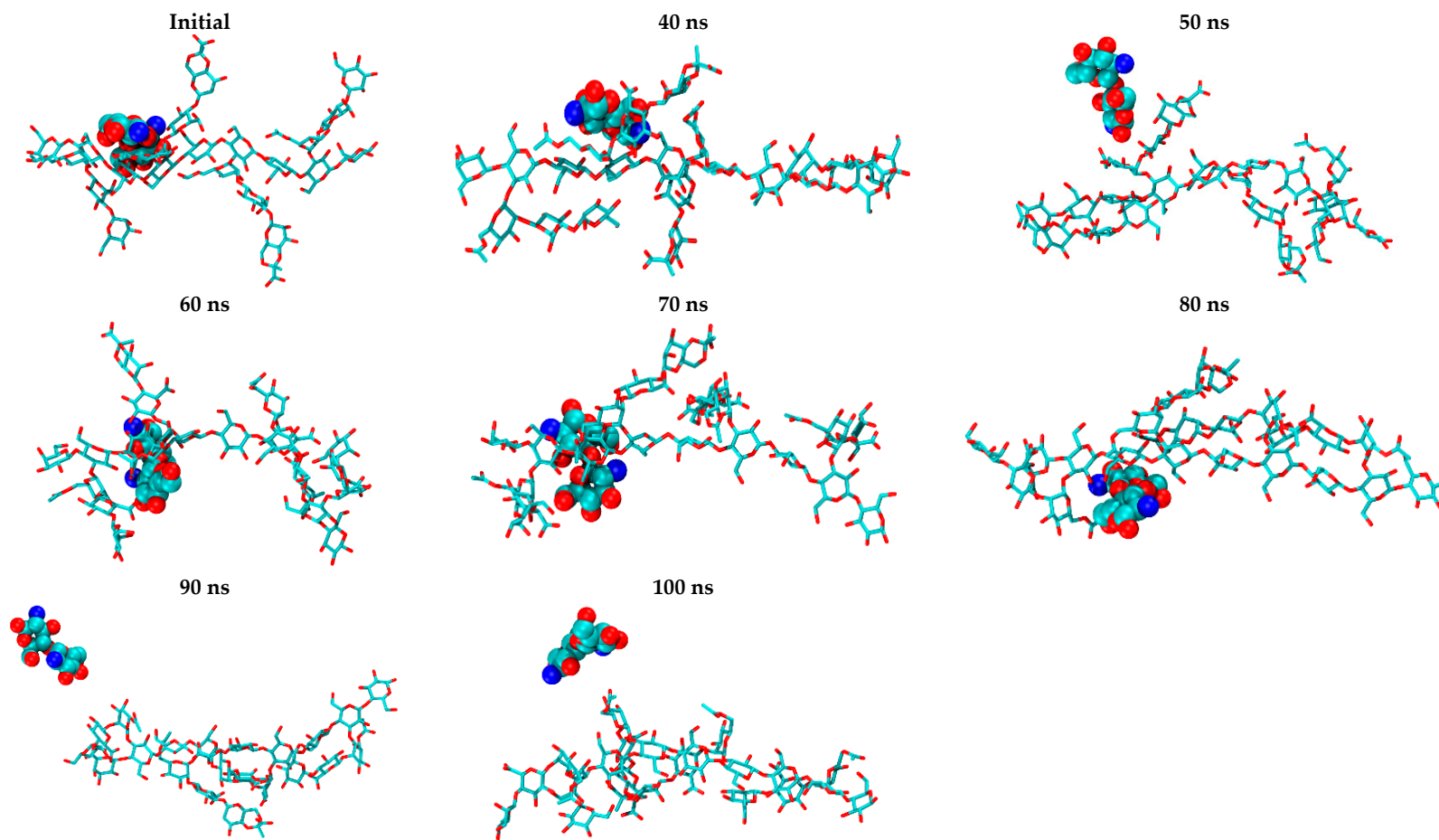
Figure 8. Snapshots of H 0 A 0 /XG complexes extracted from a 100 ns MD simulation.
