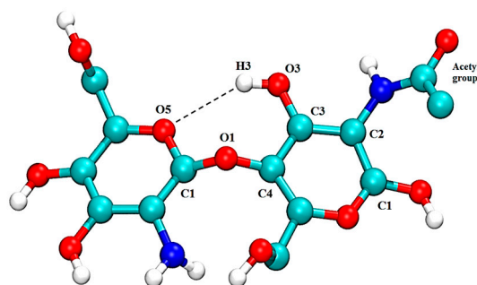
Figure 11. Molecular representation of a CS dimer, 50% acetylated, with \phi and \psi dihedral angles defined by atoms O 5 –C 1 –O 1 –C 4 and C 1 –O 1 –C 4 –C 3 , respectively. The dashed line represents the intramolecular hydrogen bond OH 3 –O 5 .
