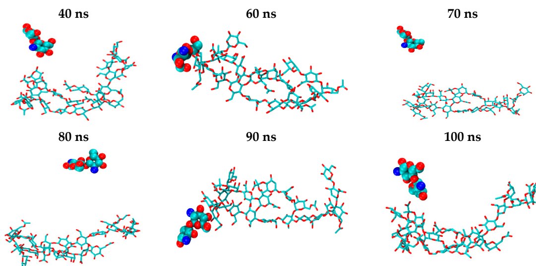
Figure 10. Snapshots of H 2 A 0 complexed with neutral XG extracted from a 100 ns MD simulation.
