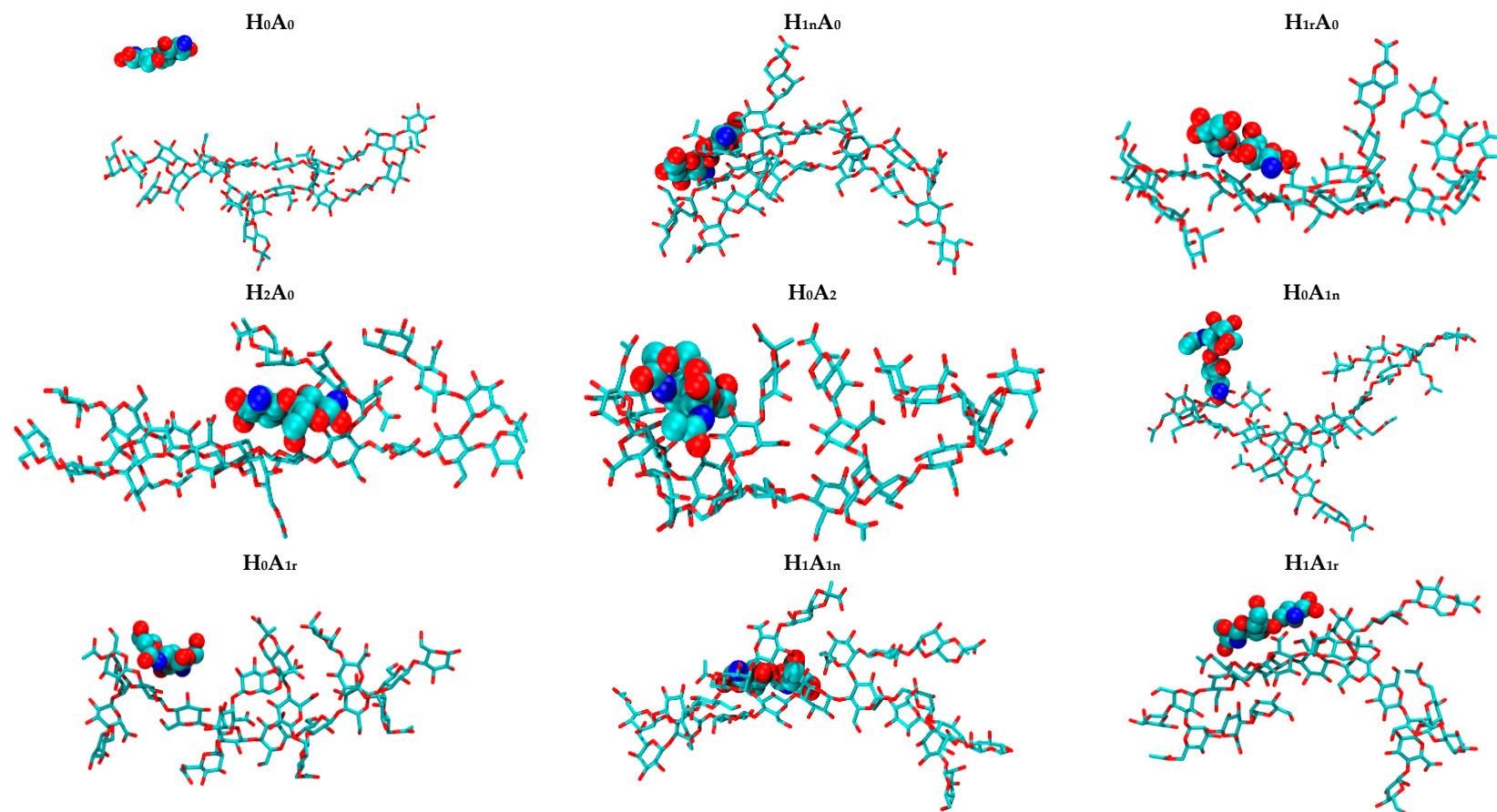
Figure 7. Average structure of each CS-XG complex during molecular dynamic simulations (MDs). Hydrogen atoms are excluded for clarity.
