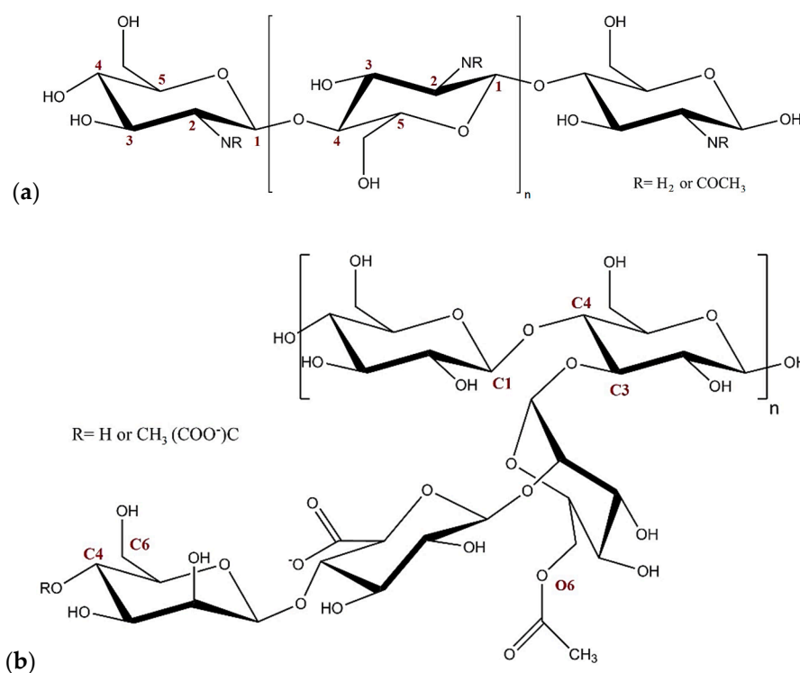
Figure 1. Schematic representation of the structure of: (a) chitosan (CS), and (b) xanthan gum (XG).
