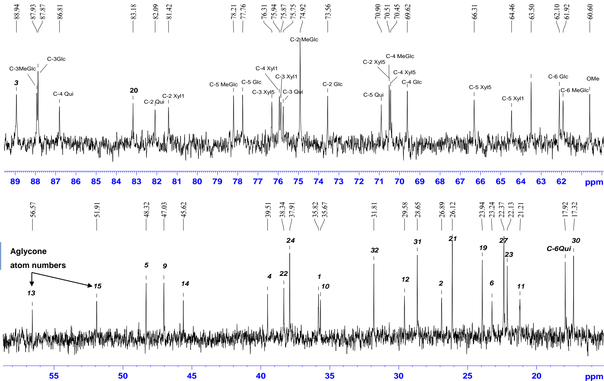
Supplementary Fig. S2. The assignment of signals in the ^{13}\text{C} NMR spectrum of cucumarioside \text{A}_2\text{-2} .
