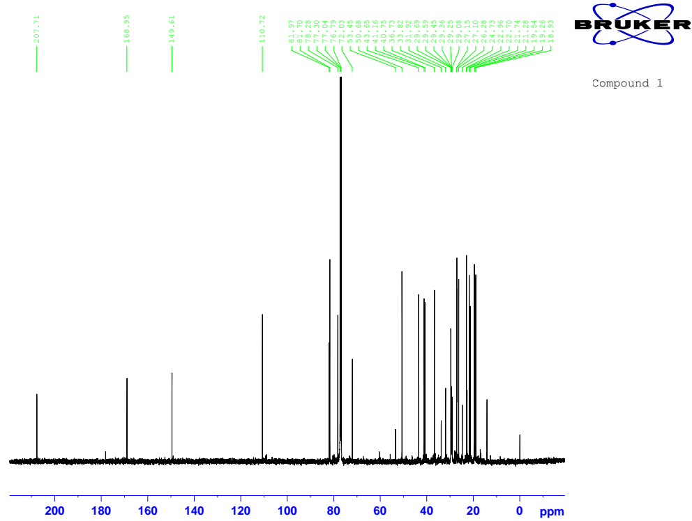
Figure S2. ^{13}\text{C} NMR spectrum of Compound 1 in \text{CDCl}_3 (125 MHz).
