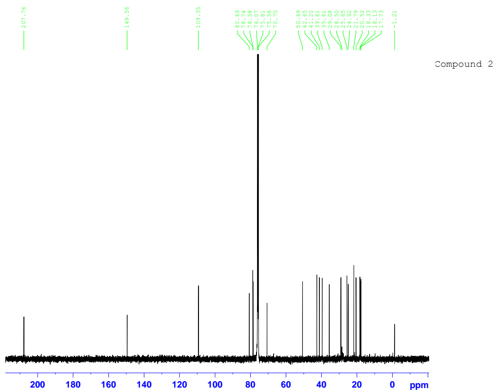
Figure S11. 13 C NMR spectrum of Compound 2 in CDCl 3 (125 MHz).
