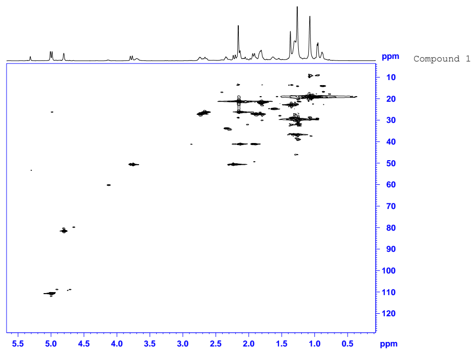
Figure S6. HSQC spectrum of Compound 1 in CDCl 3 .
