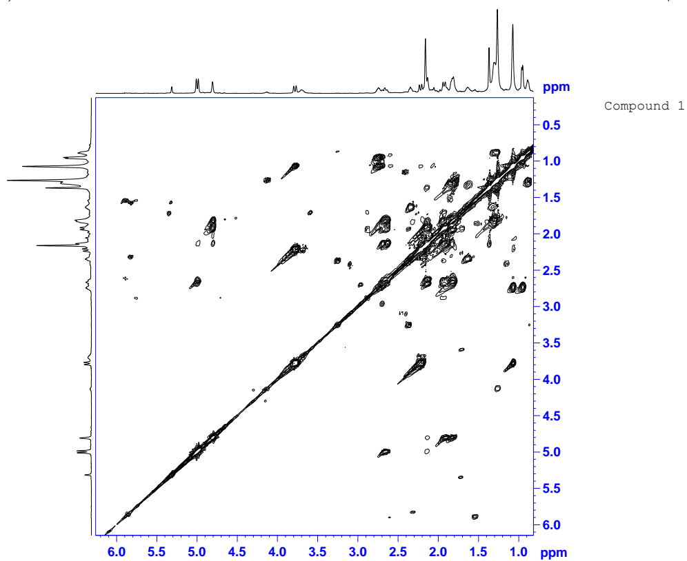
Figure S5. COSY spectrum Compound 1 in CDCl 3 .
