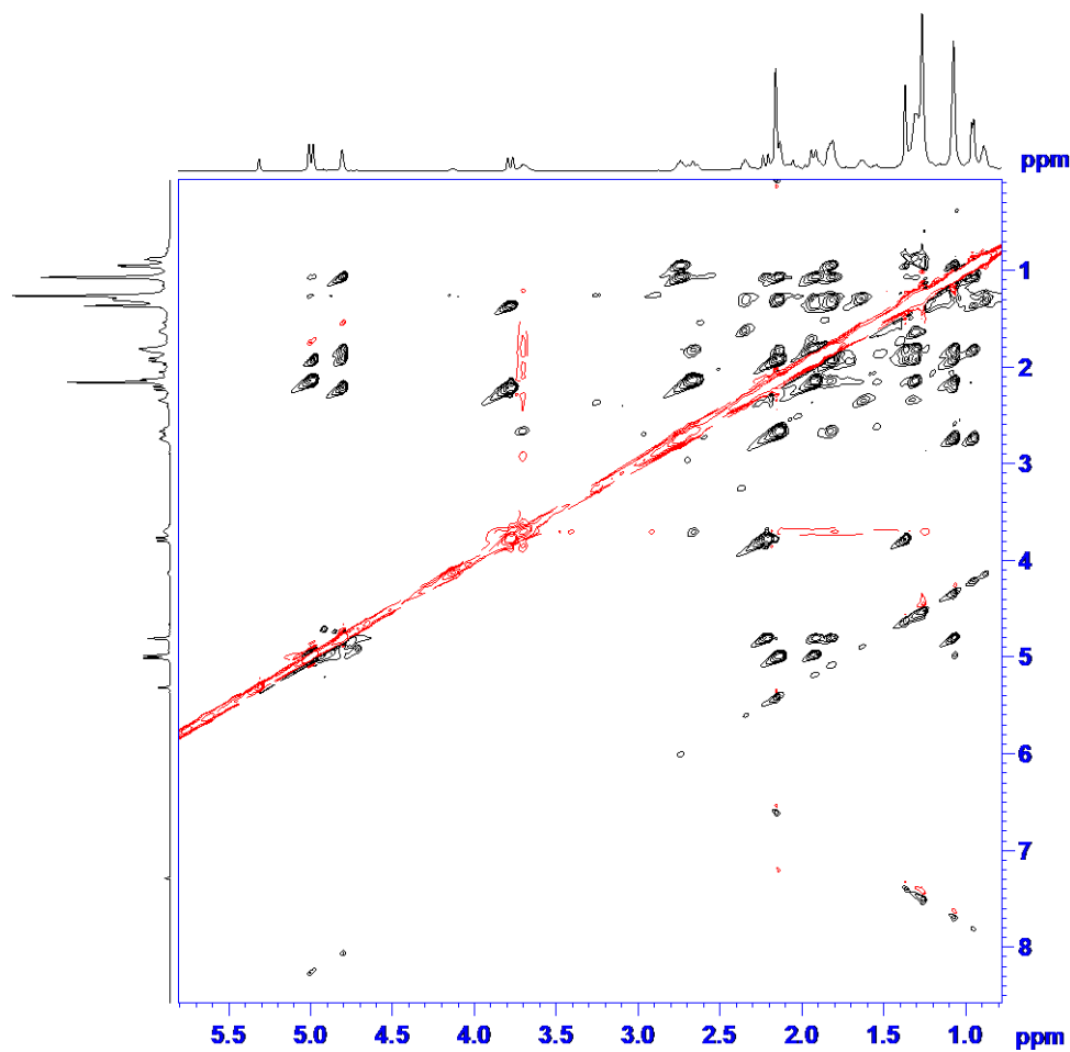
Figure S8. NOESY spectrum of Compound 1 in CDCl 3 .
