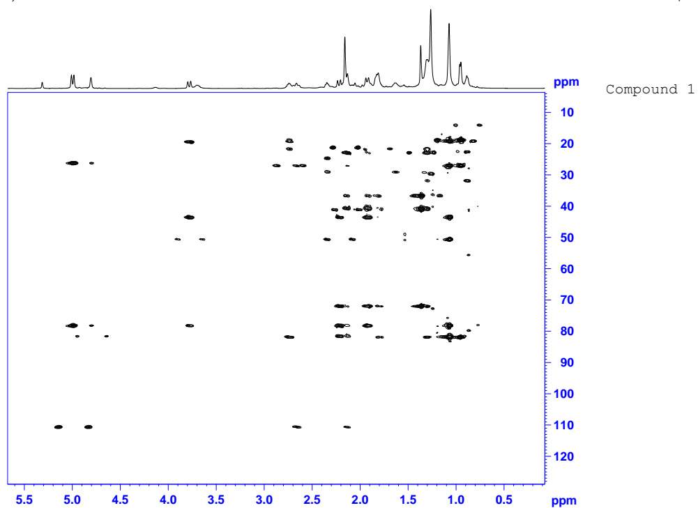
Figure S7. HMBC spectrum Compound 1 in CDCl 3 .
