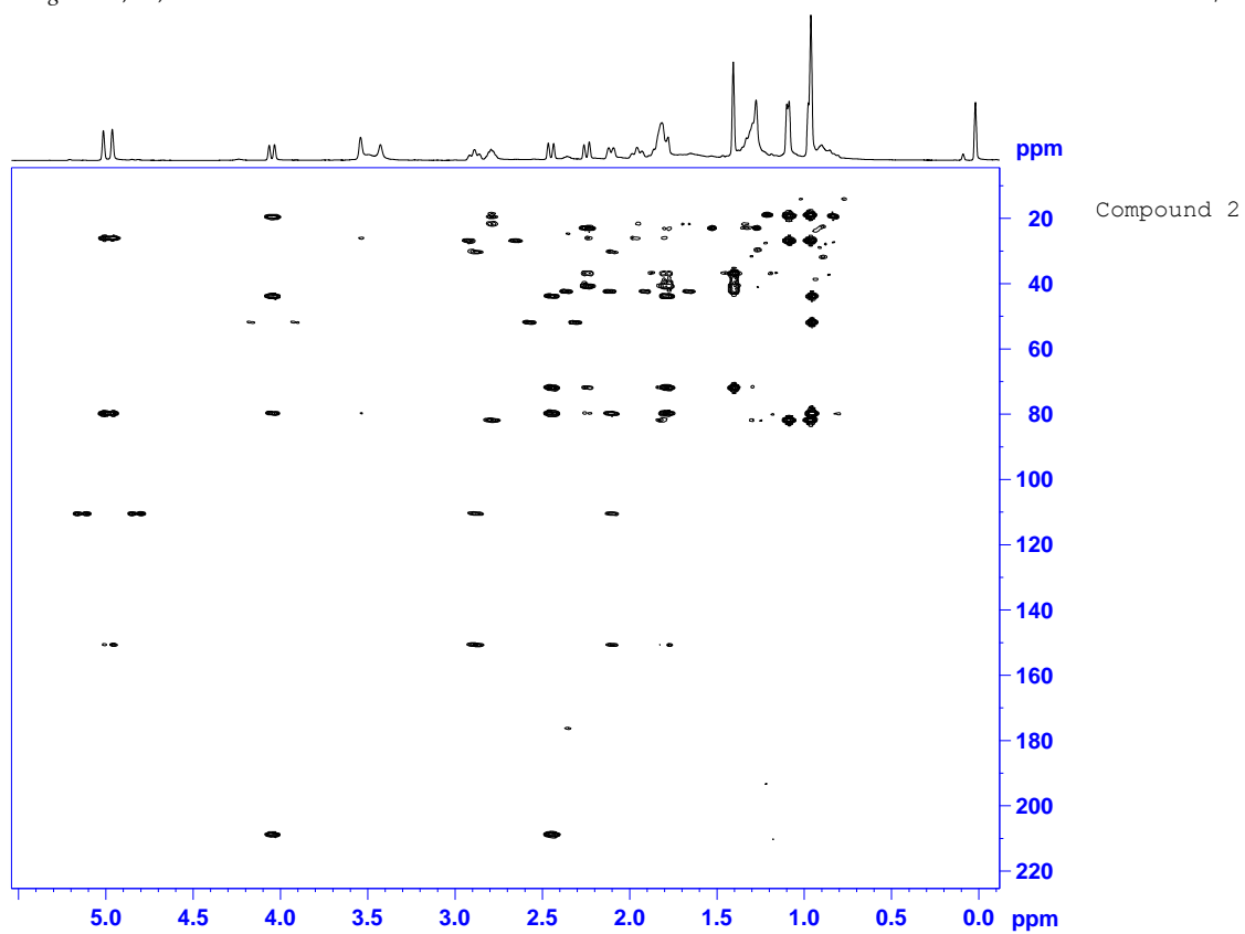
Figure S16. HMBC spectrum of Compound 2 in CDCl 3 .
