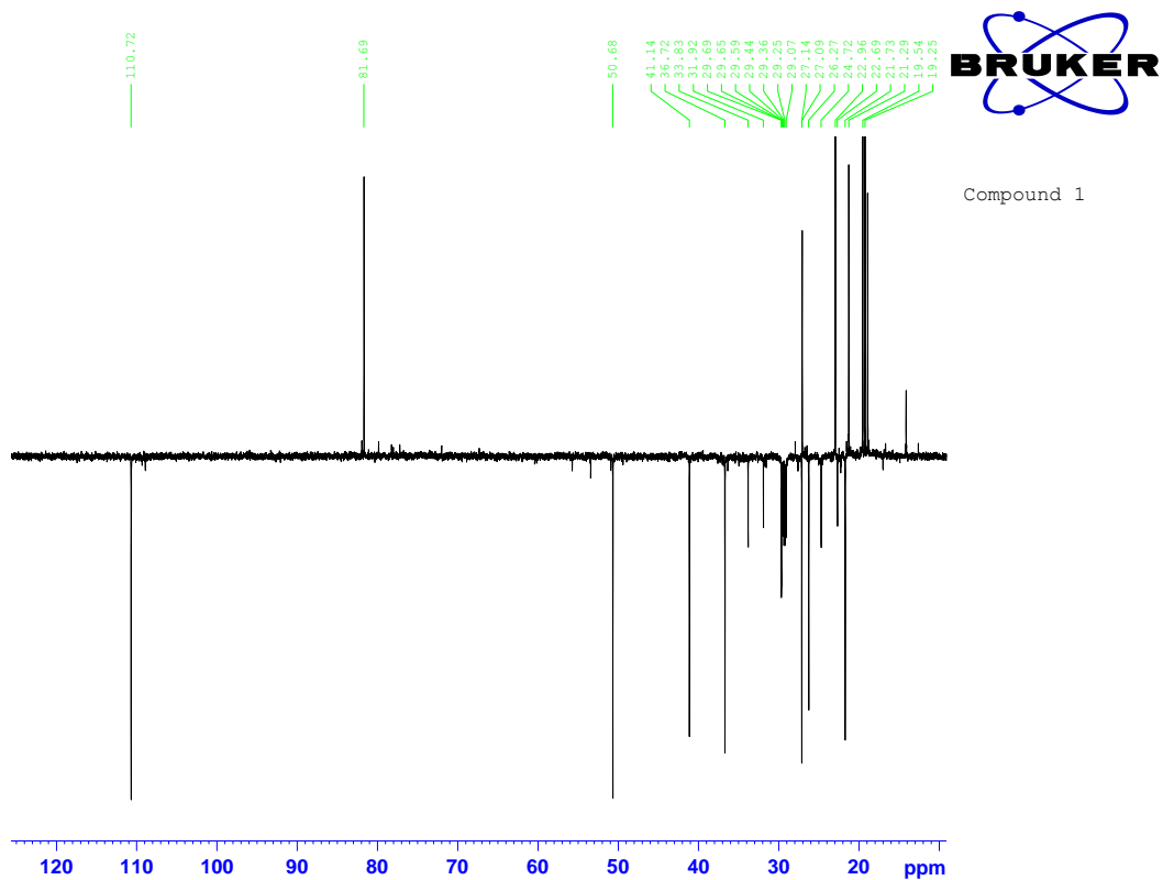
Figure S4. DEPT 135 NMR of spectrum of Compound 1 in CDCl 3 (125 MHz).
