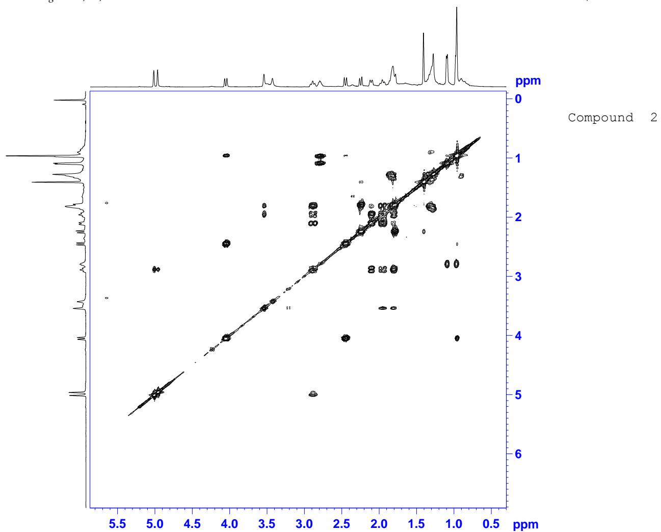
Figure S14. COSY spectrum Compound 2.
