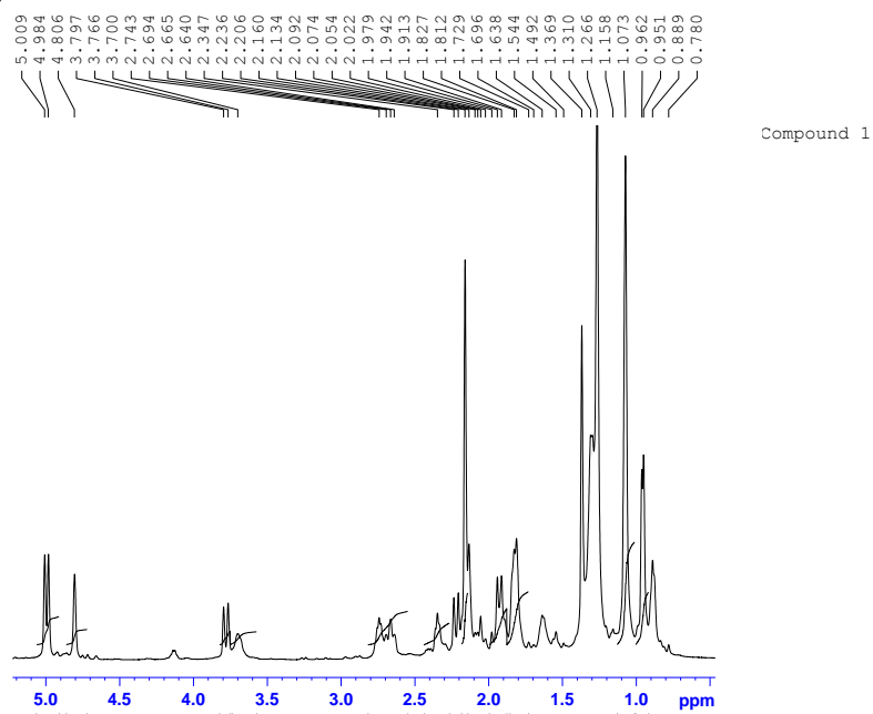
Figure S1. ^1\text{H} NMR spectrum of Compound 1 in \text{CDCl}_3 (500 MHz).
