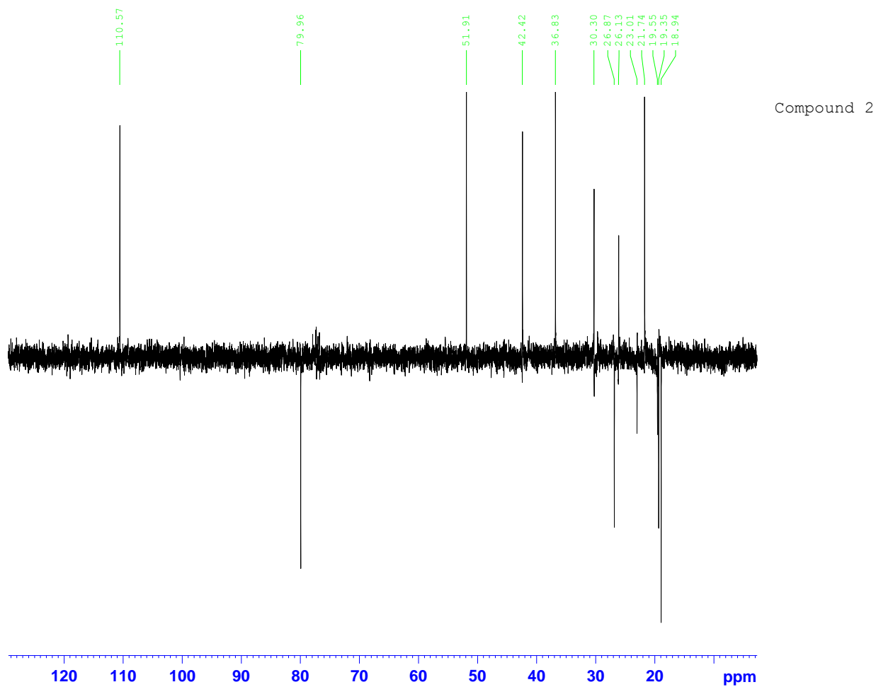
Figure S13. DEPT 135 NMR spectrum of Compound 2 in CDCl 3 (125 MHz).
