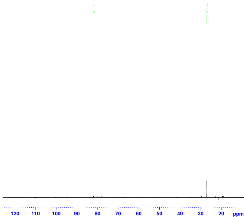
Figure S3. DEPT 90 NMR spectrum of Compound 1 in CDCl 3 (125 MHz).
