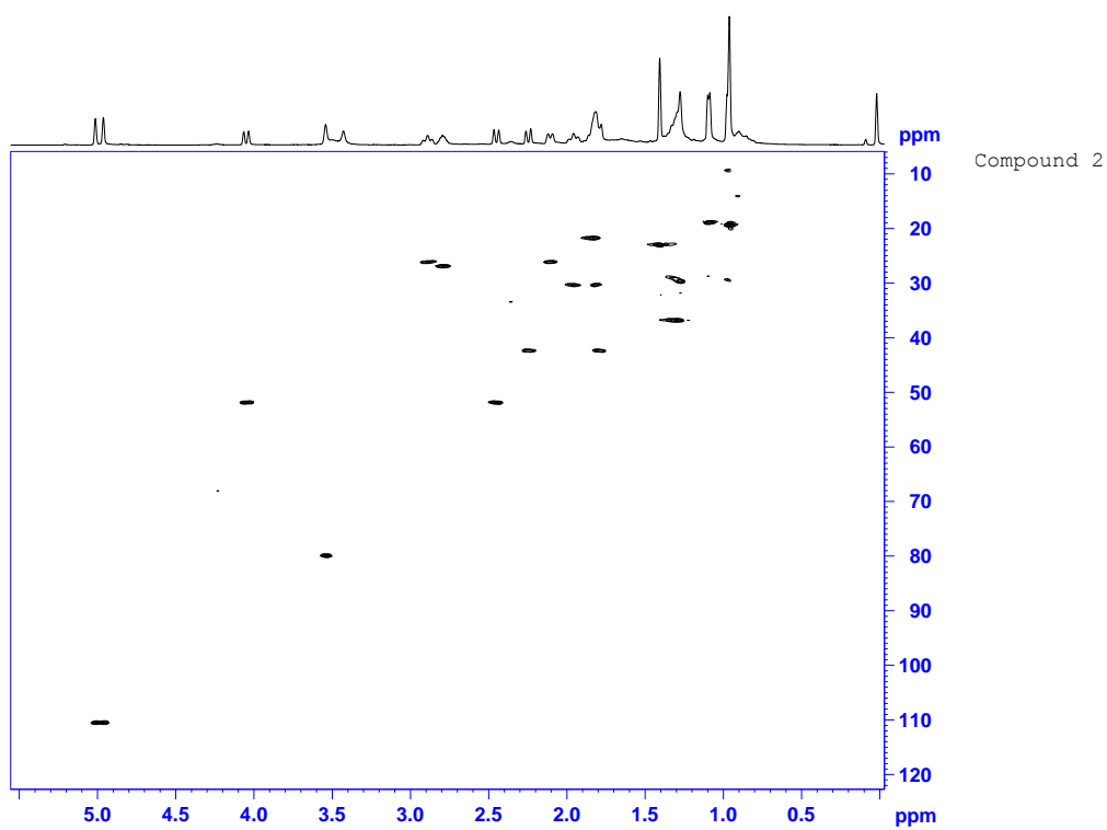
Figure S15. HSQC spectrum of Compound 2 in CDCl 3 .
