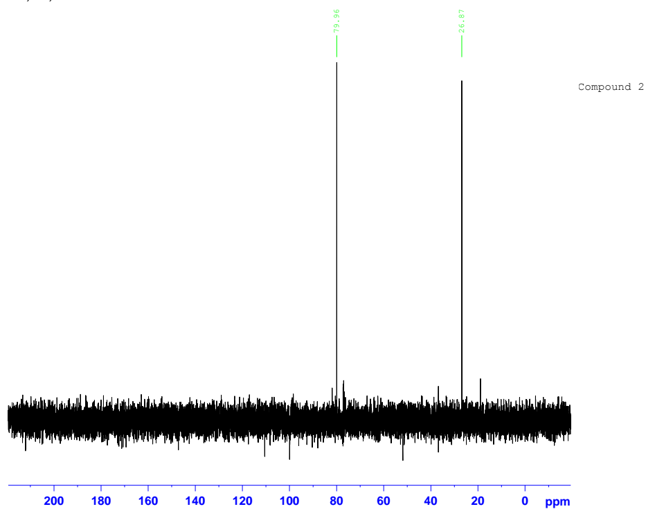
Figure S12. DEPT 90 NMR spectrum of Compound 2 in CDCl 3 (125 MHz).
