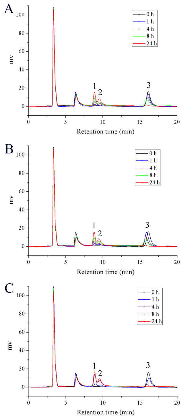
Figure S1. HPLC-RID profiles of hydrolysis of lactose in milk at 4 °C (A), 10 °C (B) and 25 °C (C). (1) Glucose; (2) Galactose; (3) Lactose.
