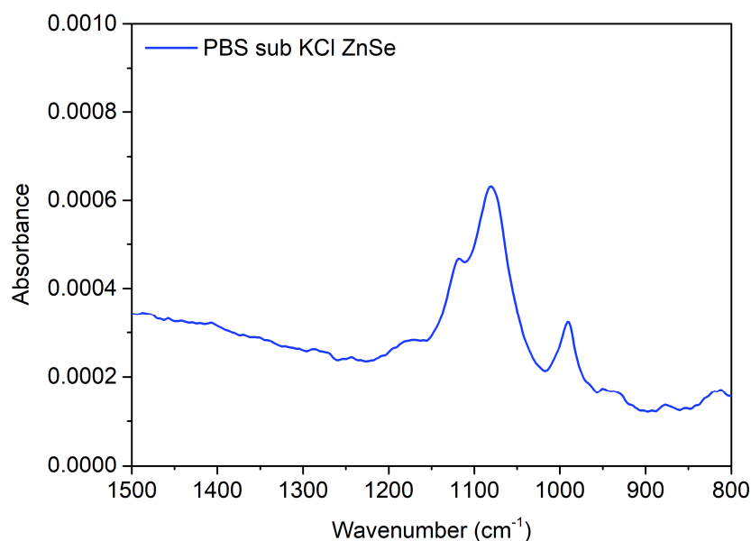
Figure S.1 ATR FTIR spectrum of PBS on a ZnSe IRE after a KCl spectrum has been subtracted to remove the contribution of the O-H bending mode of water. This spectrum has been corrected for water vapour contributions.
