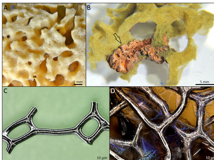
Figure 3. Spongin of the bath sponges origin (A) has been recently recognized as unique marine biomaterial for development of metal oxide-based composites (B, arrow) and the source for creation of mechanically stable 3D turbostratic graphite (C), which can be further functionalized with selected metals (D). For details, see [86].
