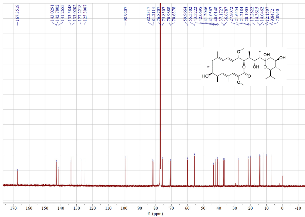
Figure S2. 13 C NMR (125 MHz, CDCl 3 ) spectrum of bafilomycin A1
