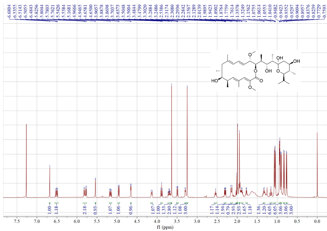
Figure S1. 1 H NMR (500 MHz, CDCl 3 ) spectrum of bafilomycin A1
