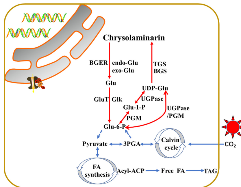
Figure 2. Schematic representation of the central synthesis pathway of chrysolaminarin in stramenopiles.
