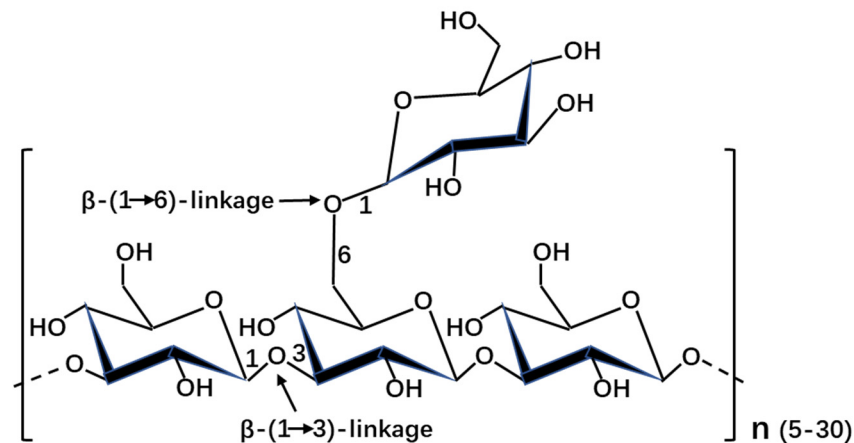
Figure 1. Schematic depiction of the structure of laminarin in stramenopiles.
