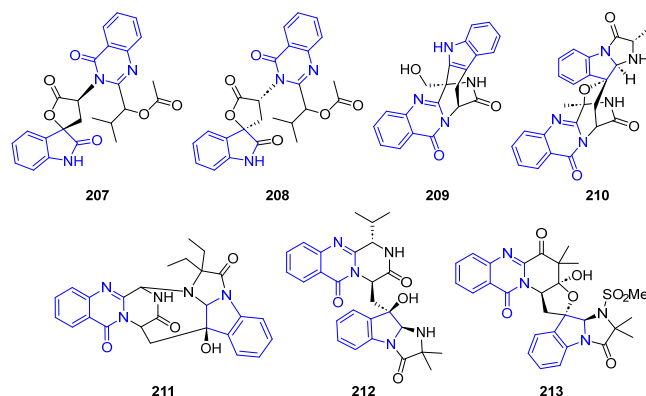
Figure 45. Structures of compounds 207–213.
