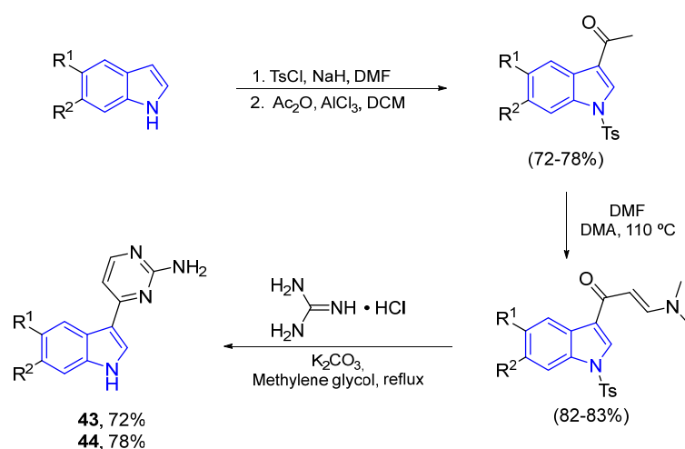
Figure 15. Fresneda and Molina's synthesis of Meridianins C (43) and D (44).
