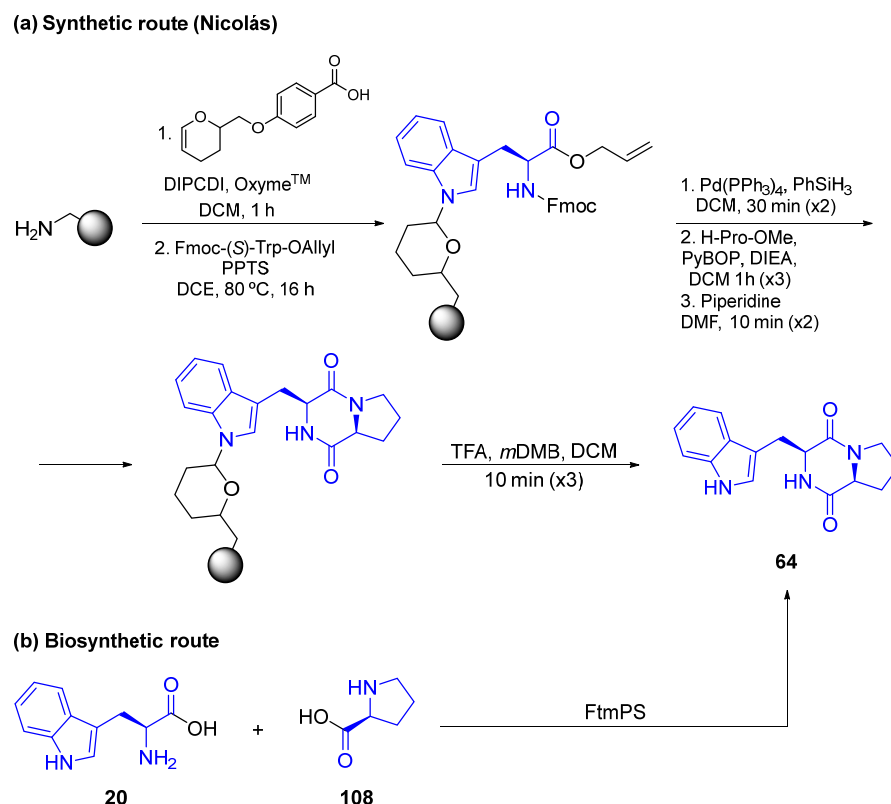
Figure 28. Synthesis and biosynthesis of Brevianamide F ( 64 ).
