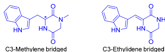
Figure 21. Basic structures of Simple Diketopiperazines.
