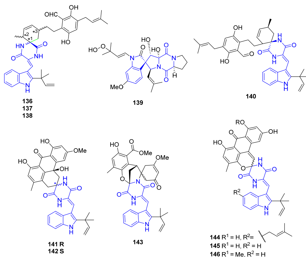
Figure 35. Structures of compounds 136–146.
