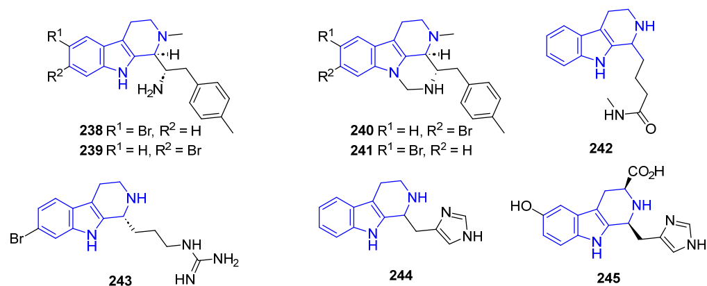
Figure 50. C1-substituted \beta C compounds 238–245.
