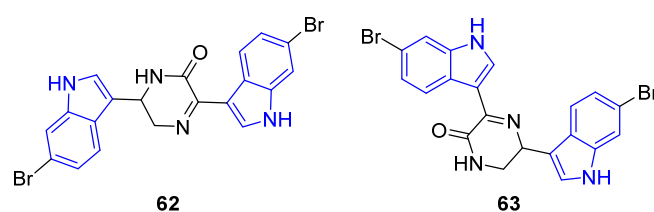
Figure 19. Structure of Hamacanthins A–B (62–63).
