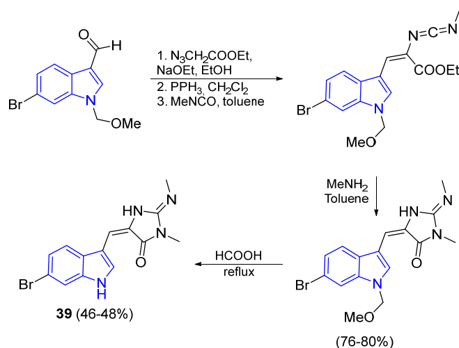
Figure 12. Stanovnik and Svetec's synthesis of Aplysinopsin derivate 39 .
