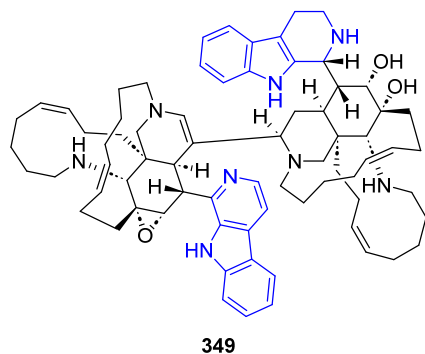
Figure 70. Structure of Kauluamine (349).
