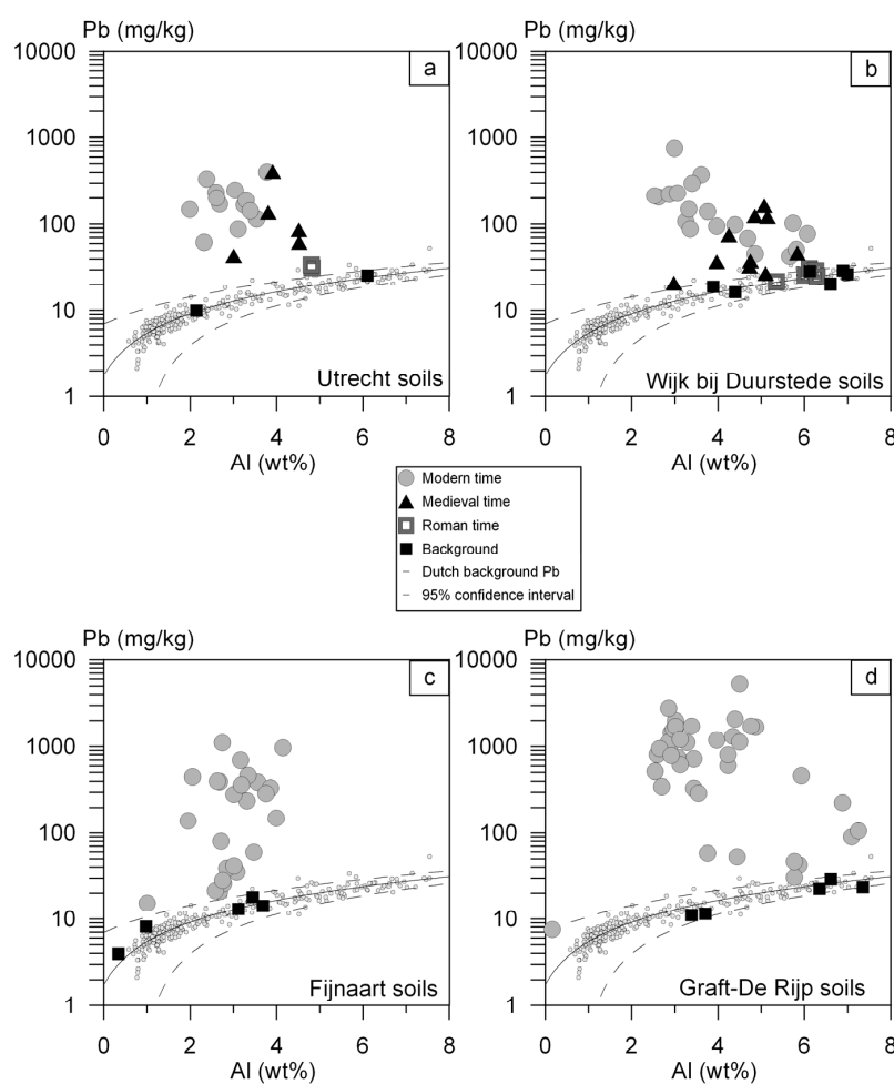
Figure 2. Pb content (mg/kg) of the soil samples—background or influenced in the Roman, Medieval or Modern time—versus Al content (wt.%) per city/village. The line indicates the average relationship between the Al and Pb content of unpolluted Dutch sedimentary soils, based on 303 samples [47]. The dashed lines are the 95% confidence intervals of the relationship between Al and Pb. a = Utrecht; b = Wijk bij Duurstede; c = Fijnaart; d = Graft-De Rijp.
