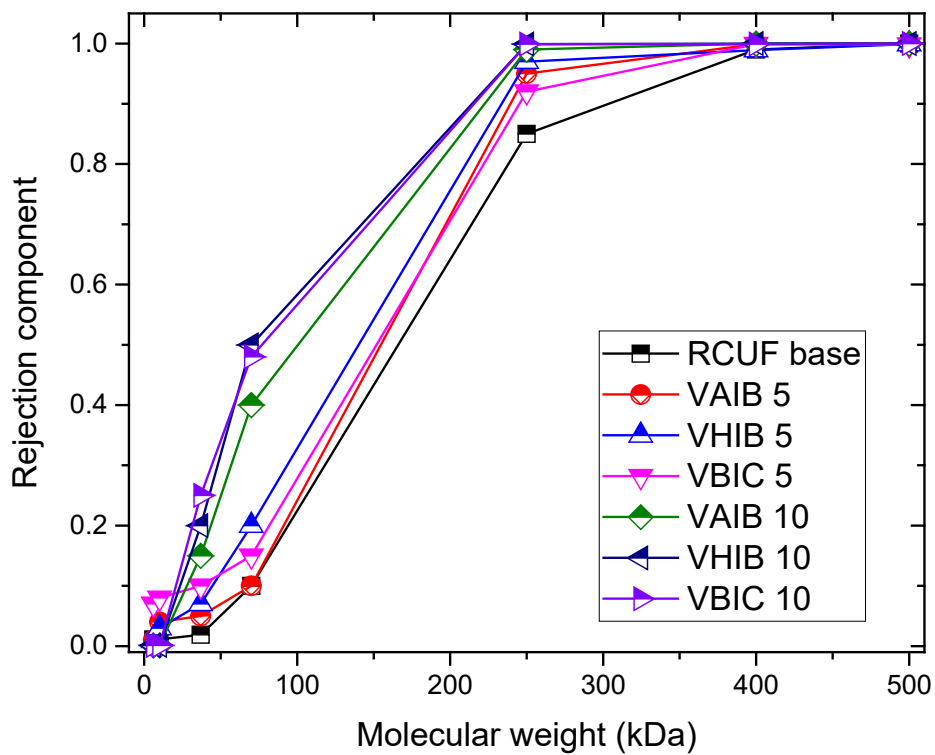
Figure S1. The dextran rejection curves for responsive membranes without any applied electric field based on size exclusion chromatography.
