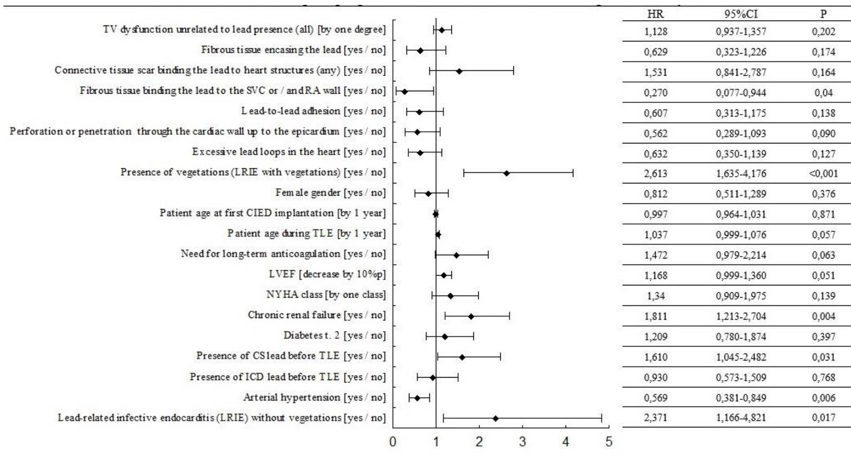
Figure S1. Prognostic value of TEE findings in follow-up of 2 years in TLE patients after adjustment of the Cox regression model for common risk factors for poor prognosis, results of multivariable Cox regression analysis.
