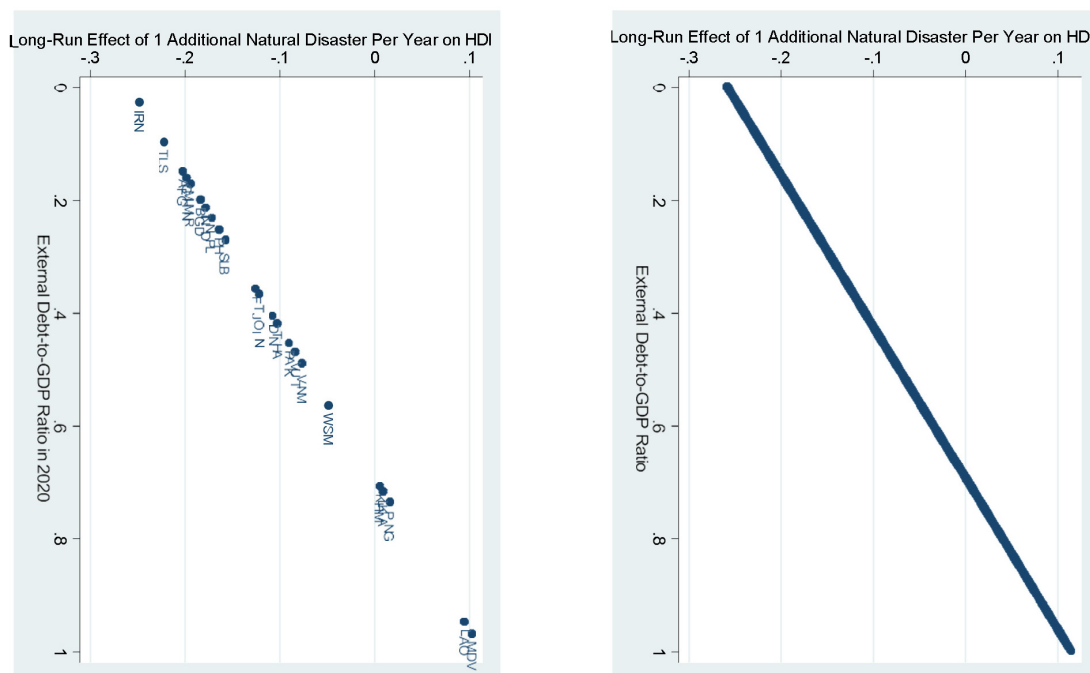
Figure 1. Effects of natural disasters on the human development index: the role of external debt.
