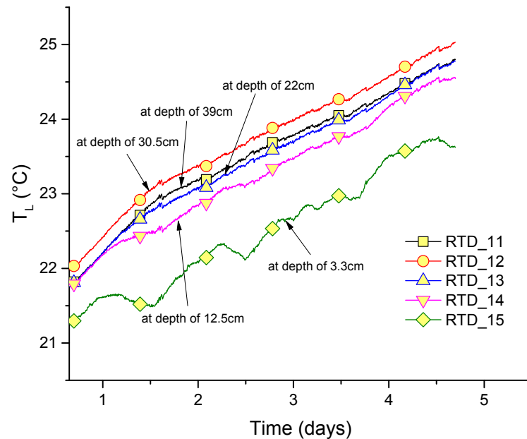
Figure 5. Time-history of the temperature on the left side of the pile.
