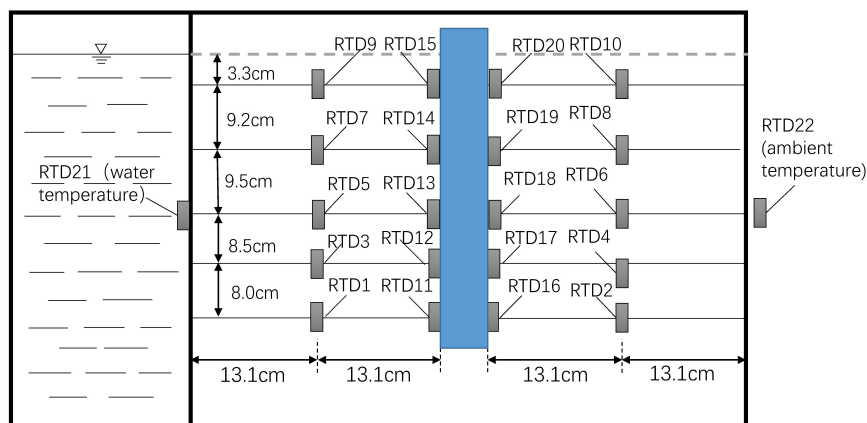
Figure 3. Layout of temperature sensors.
