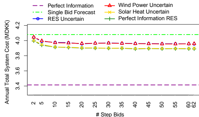
Figure 5. Comparison of different uncertainty setups and number of steps in the bidding curves in the day-ahead market optimization. The values shown are total annual system cost.
