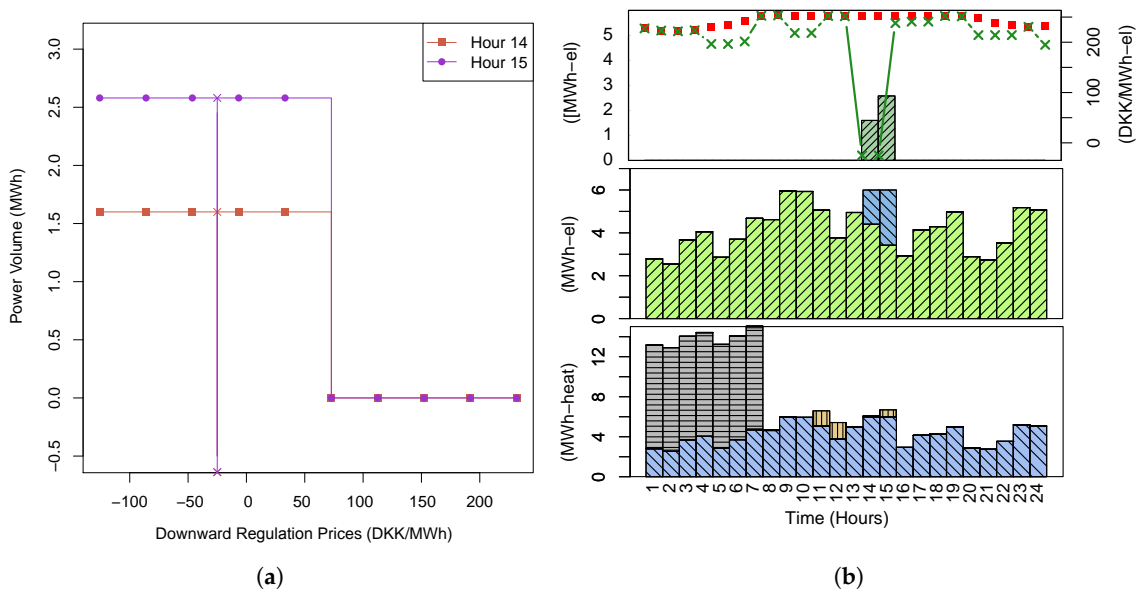
Figure 11. Downward regulation provided on 6 February 2017. (a) Bidding curves and won bids (marked with ×); (b) system operation: day-ahead committed amount, downward regulation amount, as well as day-ahead and balancing prices (top), power production (middle), and heat production (bottom).
