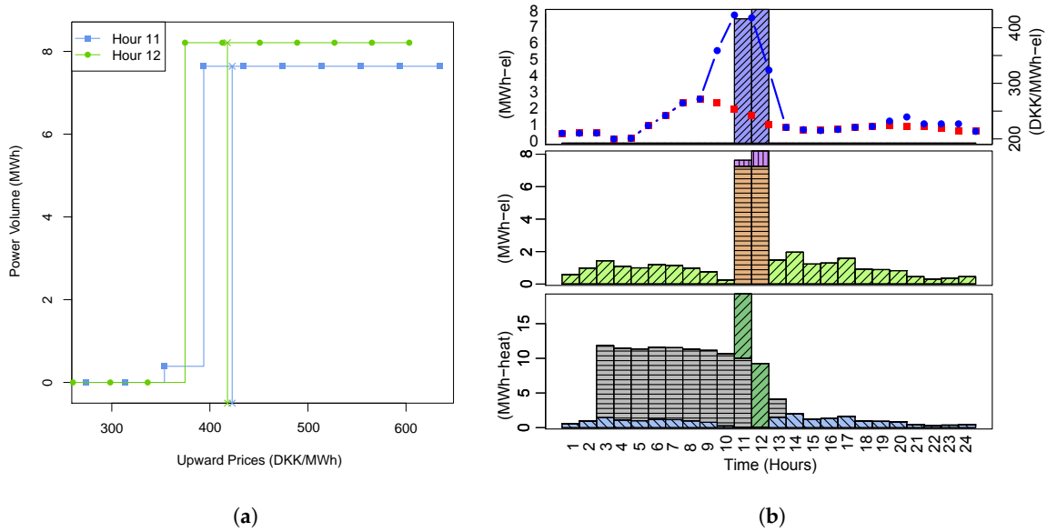
Figure 10. Upward regulation provided on 27 March 2017. (a) Bidding curves and won bids (marked with ×); (b) system operation: upward regulation amount including day-ahead and balancing prices (top), power production (middle), and heat production (bottom).
