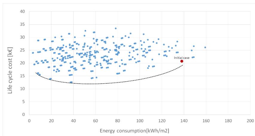
Figure 12. 30-year life cycle analysis [€] vs. heating and cooling demand (Wh).
