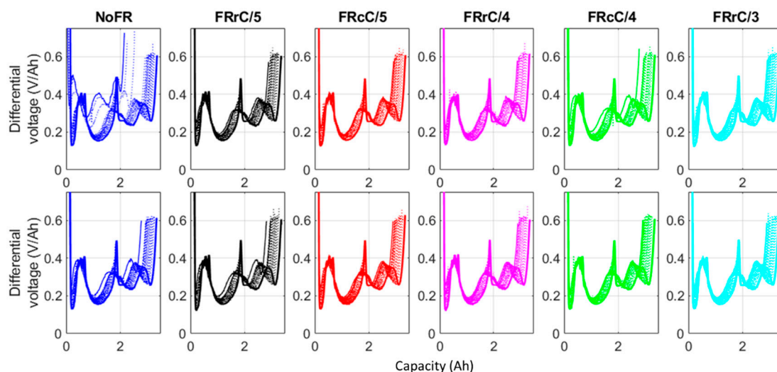
Figure S3. Differential voltage (DV) signatures for all the cells throughout the experiment.
