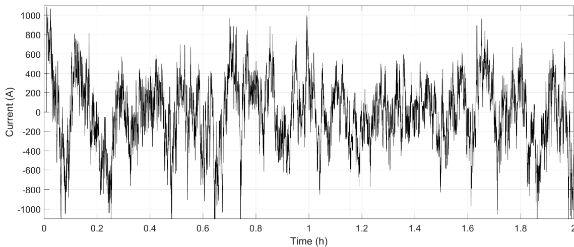
Figure S1. Frequency regulation schedule from the 1MW system.
