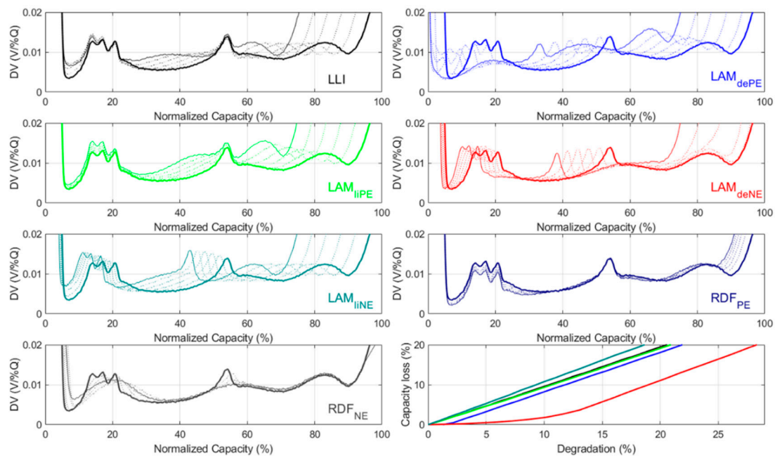
Figure S4. DV degradation map.
