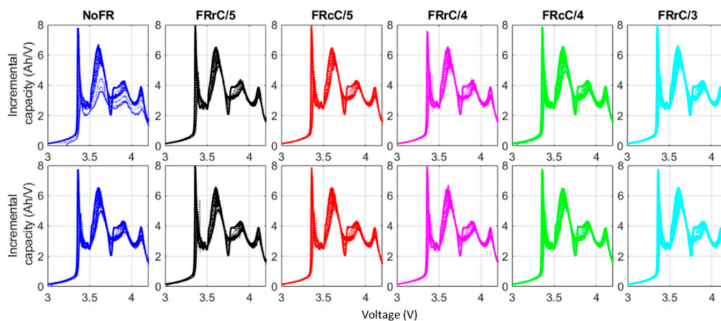
Figure S2. IC signatures for all the cells throughout the experiment.
