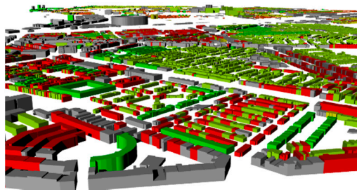
Figure 7. Rendered 3D close-up image of the Feijenoord district's heat demand.
