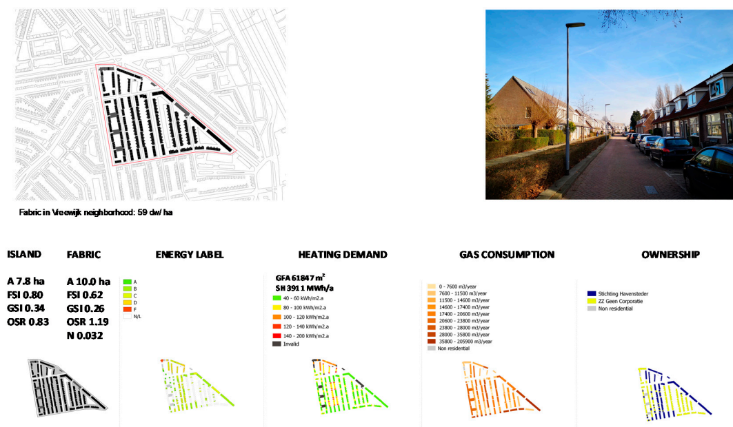
Figure 5. Mapping energy consumption levels and densification on the urban fabric of the Feijenoord district between 1990 and 2010.
