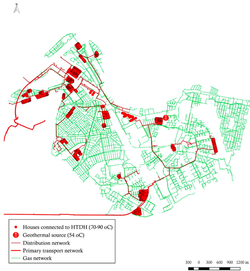
Figure 9. Centralised scenario.
