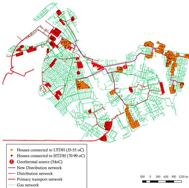
Figure 10. Decentralised scenario.
