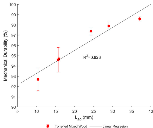
Figure 8. Mechanical durability values of torrefied mixed wood pellets versus the L_{50} of various length distributions. Error bars show the standard deviation.
