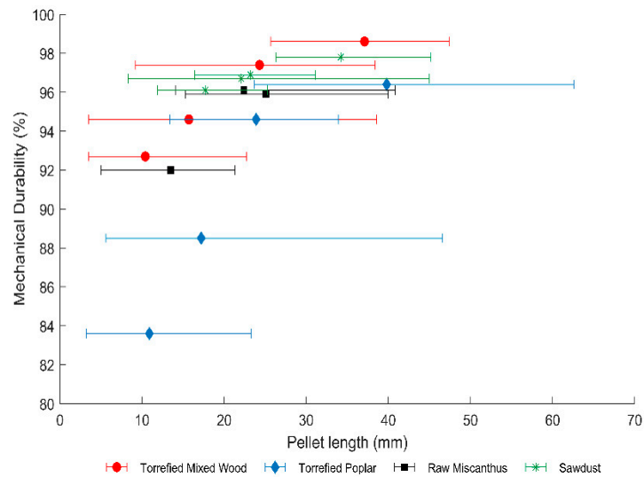
Figure 9. Mechanical durability value versus pellet length distribution intervals before mechanical durability test (solid markers show the L 50 ).
