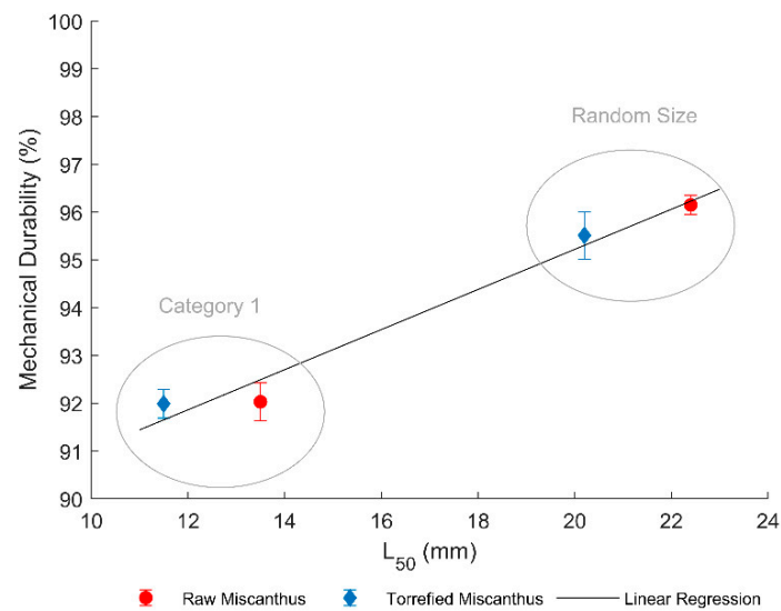
Figure 12. Mechanical durability values of raw and torrefied miscanthus pellets. Error bars show the standard deviation.
