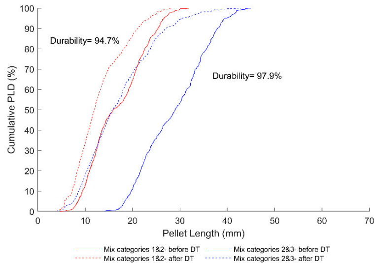
Figure 7. Pellet length distributions and mechanical durability values of torrefied mixed wood pellets: combination of categories.
