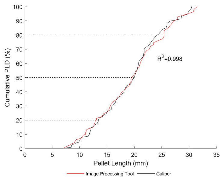
Figure 3. Pellet length distribution (PLD) measured by caliper and the in-house image processing tool.
