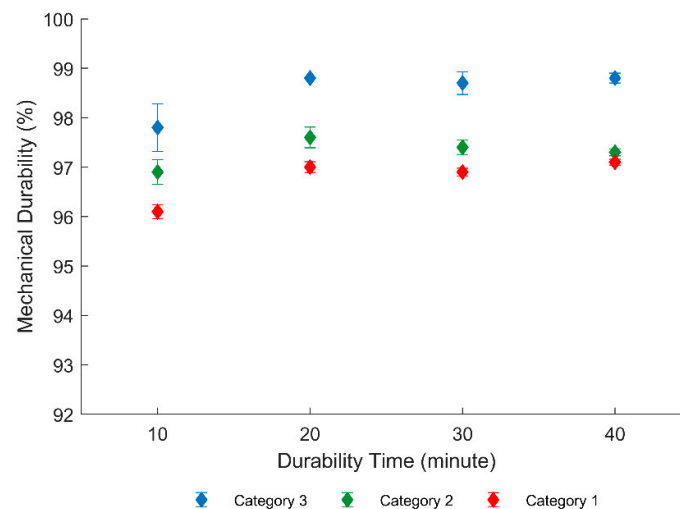
Figure 11. Mechanical durability values of sawdust pellets after several mechanical durability tests. Error bars show the standard deviation.
