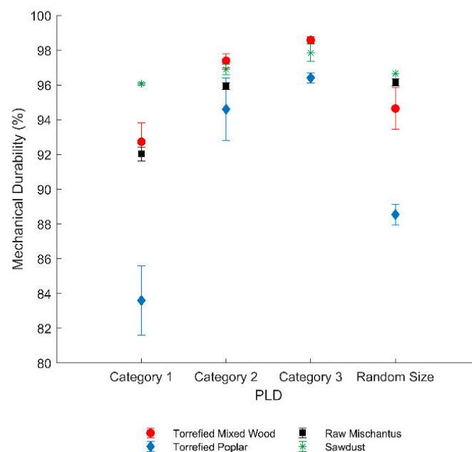
Figure 5. Mechanical durability results of different biomass pellets based on their pellet length distributions. Error bars show the standard deviation.
