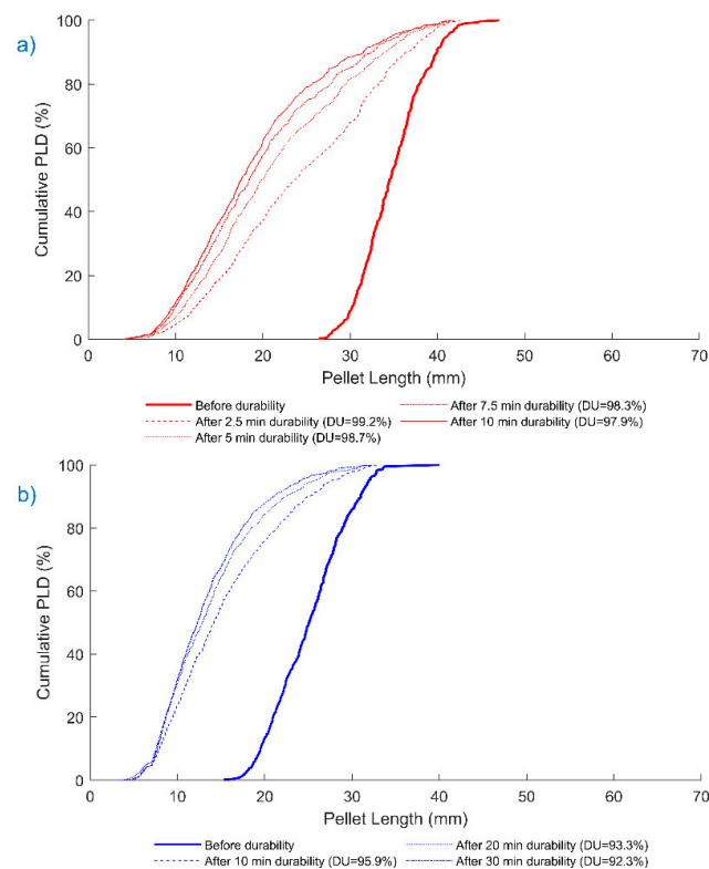
Figure 10. Pellet length distributions of (a) torrefied mixed wood and (b) raw miscanthus before and after different mechanical durability tests (DU: mechanical durability).
