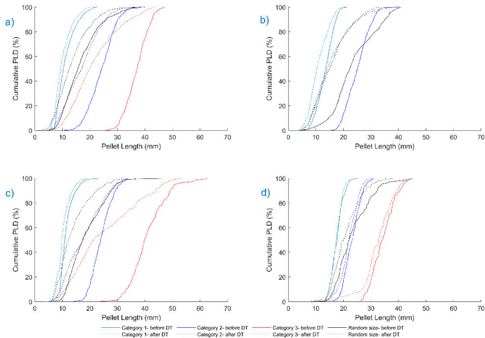
Figure 6. Pellet length distributions before and after mechanical durability tests for (a) torrefied mixed wood, (b) raw miscanthus, (c) torrefied poplar, and (d) sawdust pellets (DT: Durability test).
