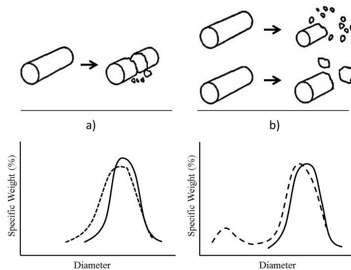
Figure 13. Two different breakage mechanisms of pellets. (a) fragmentation, (b) abrasion and their particle size distribution curves adapted from [37].
