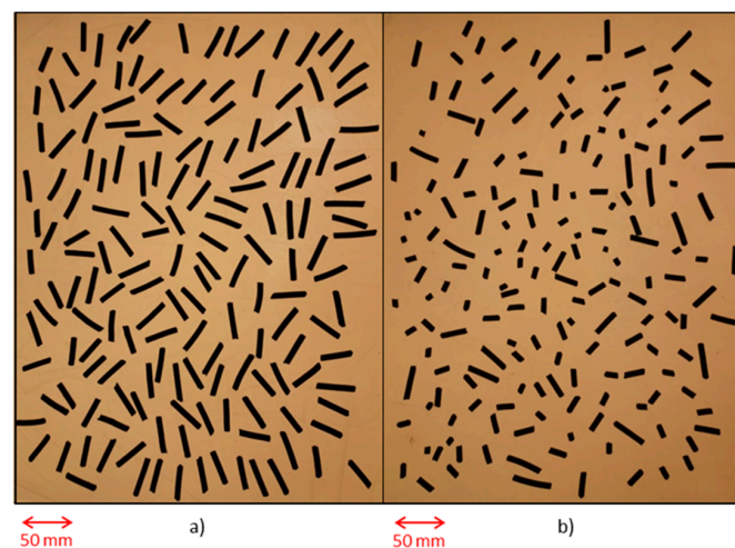
Figure 4. A sample image taken from the torrefied mixed wood pellets, (a) before and (b) after mechanical durability test.
