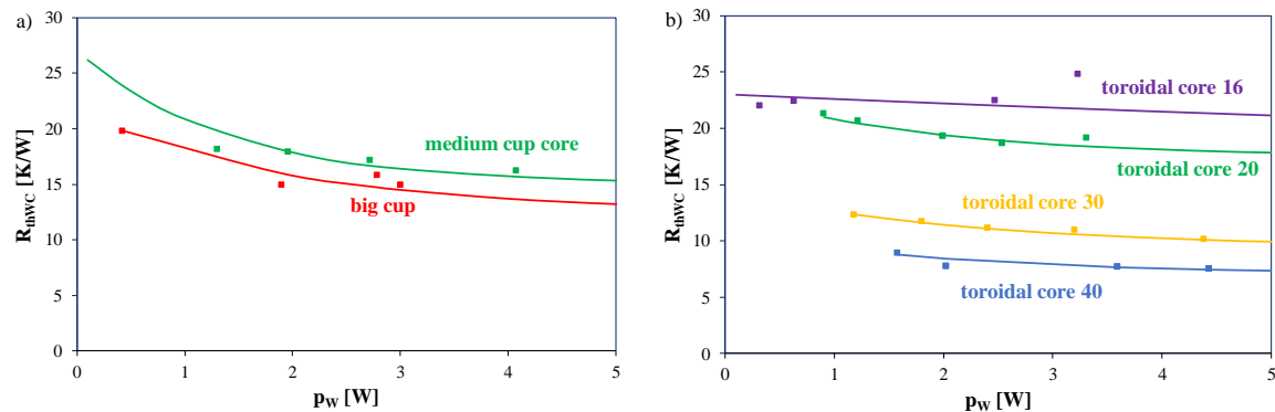
Figure 15. Measured and calculated dependences of thermal resistance R_{thWC} of inductors with (a) cup cores and (b) toroidal core on dissipated power in the winding.
