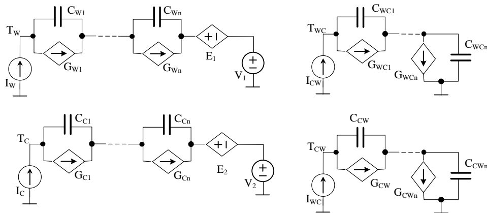
Figure 1. Nonlinear compact thermal model of the inductor.
