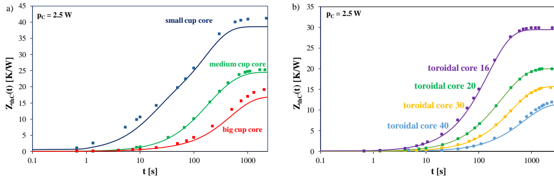
Figure 6. Measured and calculated waveforms of transient thermal impedance of the core for inductors with (a) cup and (b) toroidal cores of different dimensions.
