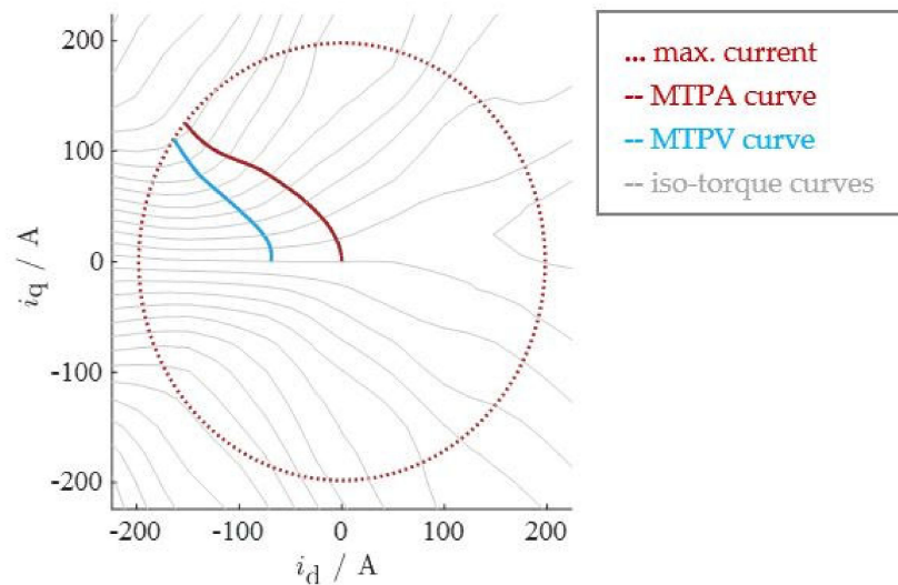
Figure 1. Result of the reference torque calculation. The x-axis denotes the direct current, the y-axis the quadrature current. The torque hyperbolas (iso-torque curves) in grey are calculated considering the machines flux-linkages and currents. The maximum current magnitude is the red dotted circle. The maximum torque per ampere (MTPA) locus for maximum torque at minimum current is the solid red line. The maximum torque per volt/voltage (MTPV) locus for maximum torque at constrained voltage is the solid blue line.
