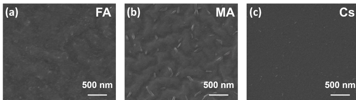
Figure S1. Top-view SEM images of quasi-2D perovskite films with (a) FA, (b) MA, and (c) Cs cations.
