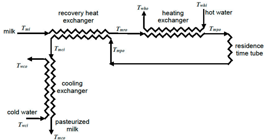
Figure 1. Flow chart of thermal exchangers system of the milk pasteurization.
