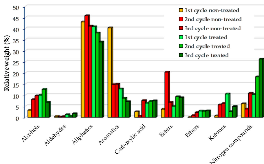
Figure 3. GC-MS bio-oil based on groups for catalyst regeneration of treated and non-treated microalgae.
