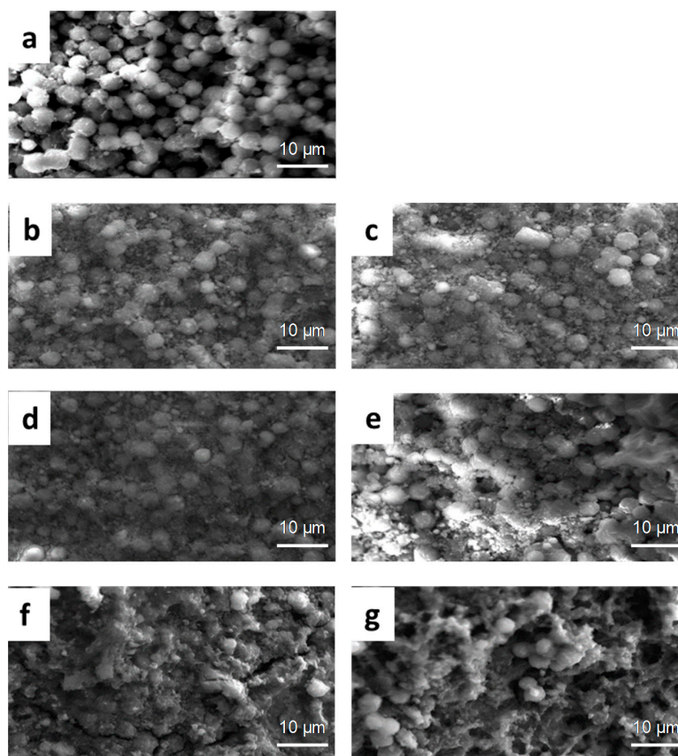
Figure 4. SEM micrograph of fresh (a) and spent catalysts after 1st, 2nd and 3rd pyrolysis experiments with (b–d) non pre-treated and (e–g) pre-treated microalgae.
