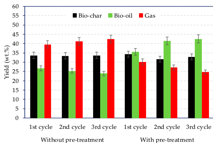
Figure 2. Products yield distribution with and without pre-treatment over three consecutive cycle catalyst regeneration.
