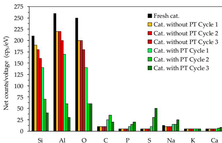
Figure 5. EDS of the spent catalysts after the pyrolysis experiments.
