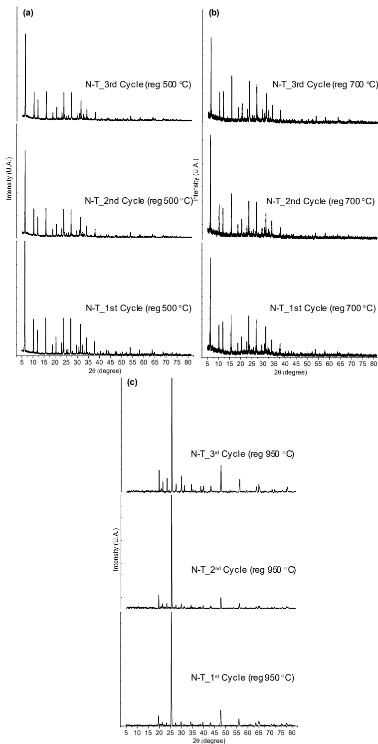
Figure 6. XRD of Li-LSX zeolite (non-treated microalgae) regenerated at (a) 500 °C, (b) 700 °C and (c) 950 °C.
