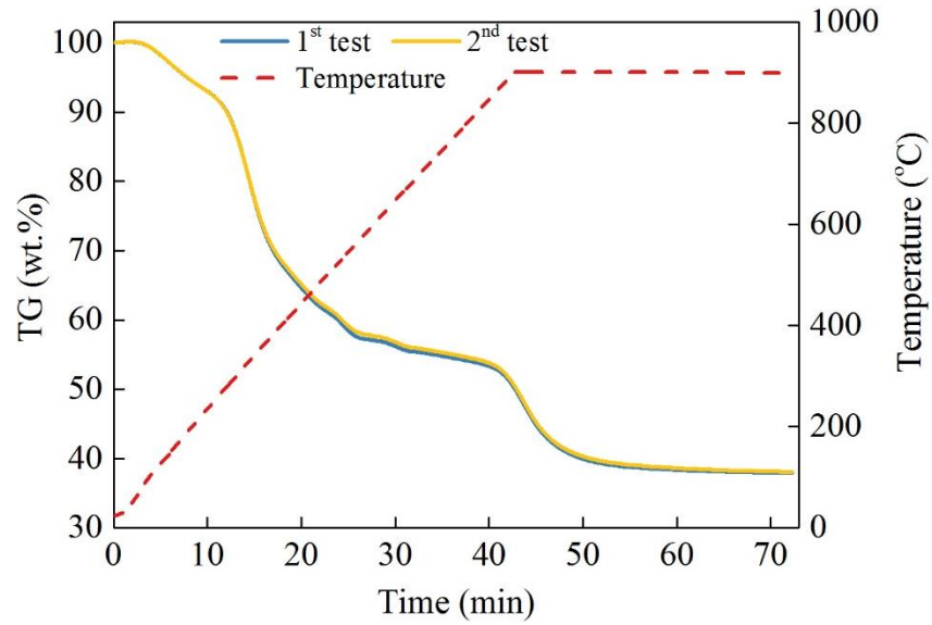
Figure S1. The repeated TGA experiment of the mixture fuel with 82 wt.% cyanobacteria and 18 wt.% coal (82CYA sample).
