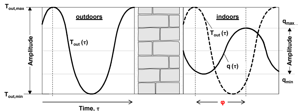
Figure 2. Schematic of the periodic heat transfer process in an external wall.
