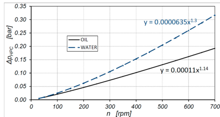
Figure 18. Characteristics of the pressure increase \Delta p_{HPC} = f(n) calculated according to Formula (9)—motor supplied with oil and water.
