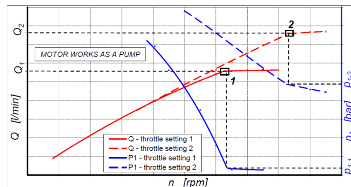
Figure 4. Delivery Q of motor 1 working as a pump and the pressure p_1 in the suction port of motor 1 for two different settings of throttle valve TV —according to the scheme in Figure 3 [23].
