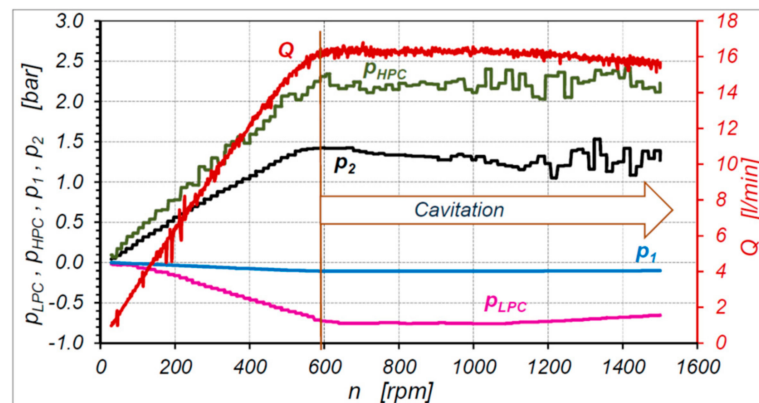
Figure 15. Characteristics of p_1 = f(n) , p_2 = f(n) , p_{HPC} = f(n) , p_{LPC} = f(n) and Q = f(n) over the entire range of the motor shaft speed n —motor supplied with oil [23].
