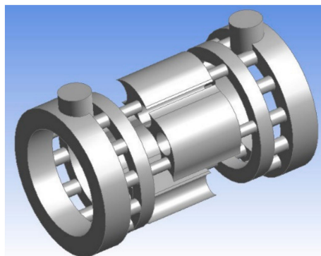
Figure 23. Simplified model of liquid volume in the motor [28].
