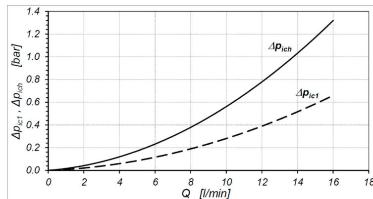
Figure 19. Characteristics of the total pressure drop \Delta p_{ich} = f(Q) in the motor and the pressure drop \Delta p_{ic1} = f(Q) in one internal channel of the motor—motor supplied with water [23].
