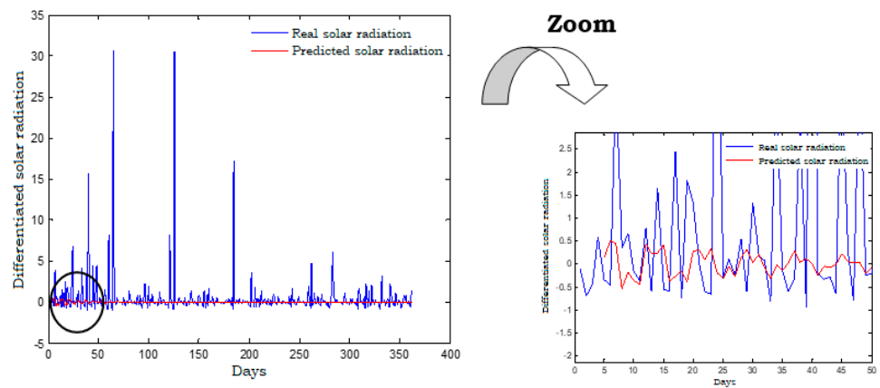
Figure 18. Solar radiation prediction using the ARMA (4,4) model.
