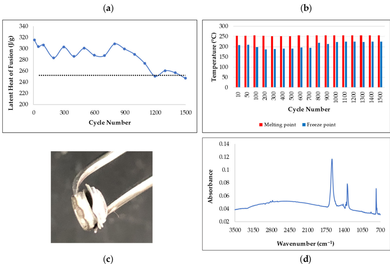
Figure 2. (a) Latent heat of sodium formate as a function of thermal cycles, (b) plot of melting and freezing points of sodium formation as a function of thermal cycles, (c) Image of ruptured differential scanning calorimetry (DSC) pan, and (d) FTIR spectrum of cycled sodium formate phase change material (PCM), showing degradation to sodium oxalate.
