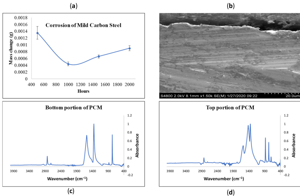
Figure 5. (a) Corrosion of mild carbon steel in molten sodium formate. Corrosion data are expressed as average mass change of coupons with standard error over 2000 h, measured at 500-h increments. (b) SEM images of cross sectioned carbon steel coupon after 2000-h immersion in molten sodium formate. Magnification 1500 \times . (c) FTIR of the bottom portion of the PCM after corrosion experiment was completed. (d) FTIR of the top portion of the PCM after corrosion experiment was completed.
