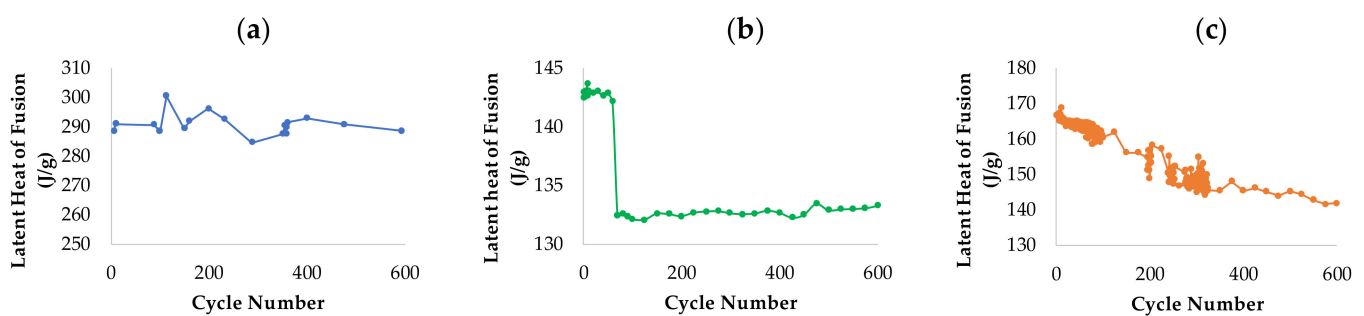
Figure 1. (a) Latent heat ( H_f ) as a function of cycle number up to 600 cycles for sodium formate, (b) sodium/potassium formate, and (c) sodium/calcium formate.
