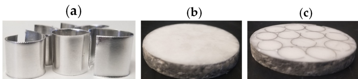
Figure 4. (a) Image of aluminum 6061 rings, (b) image of PCM without aluminum rings, (c) image of eutectic PCM with aluminum rings PCM discs were nominally 8 mm thick and 50 mm in diameter.
