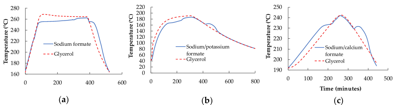
Figure 3. T-history experimental results of PCM vs. glycerol reference: (a) sodium formate, (b) sodium/potassium formate, and (c) sodium/calcium formate. The temperature difference between the onset of the hump in the cool-down curve and the maximum rise in the hump represents the degrees of supercooling [13].
