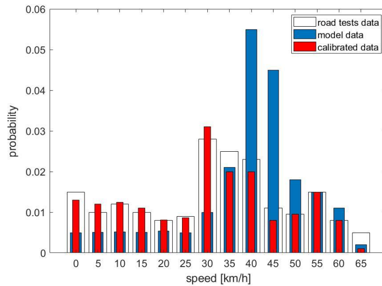
Figure 11. The speed for road tests, model and calibrated data.
