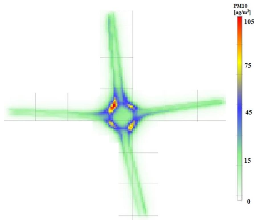
Figure 17. PM10 concentration from the tested two-lane roundabout according to the VERSIT + model for the share of 25% of electric vehicles.
