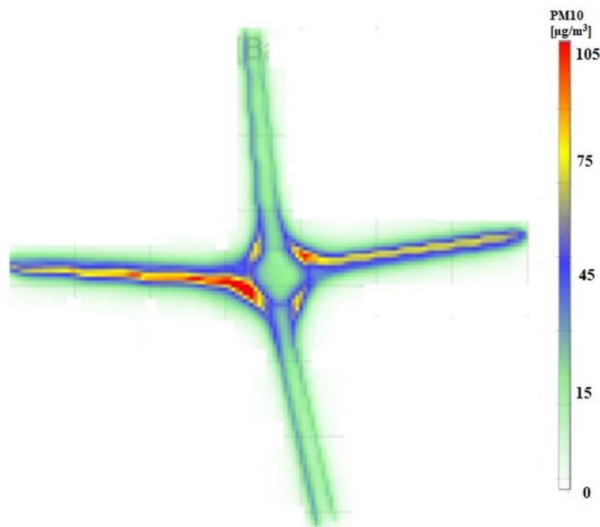
Figure 16. PM10 concentration from an alternative turbo roundabout according to the VER-SIT + model.
