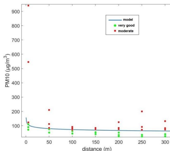
Figure 13. Comparison of the results of PM10 concentration from the model and from real data, when the air quality was very good or moderate for the area of a two-lane roundabout.
