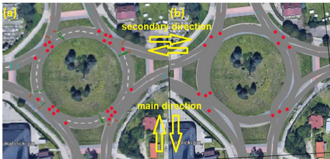
Figure 4. Researched roundabouts solutions modelled in Vissim: (a) two-lane (b) turbo (red dots are conflict points).
