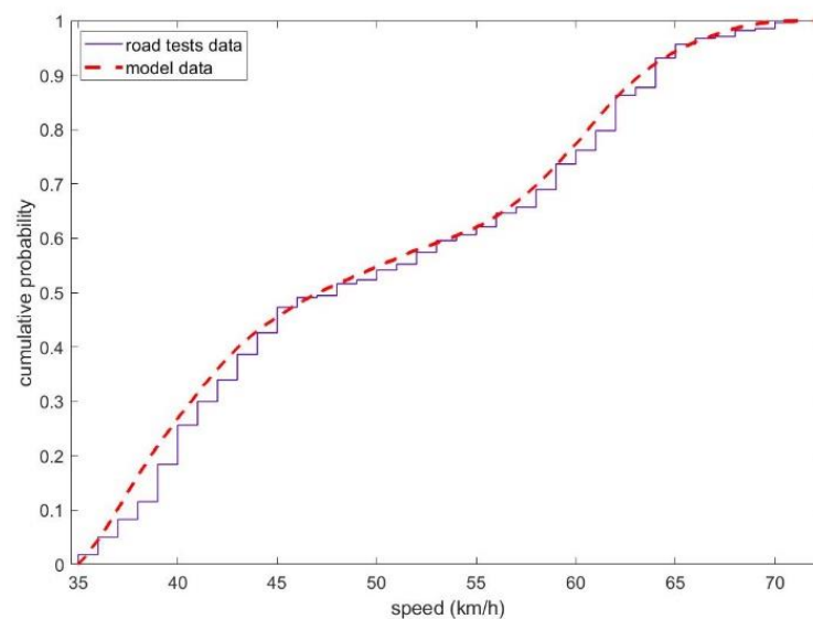
Figure 9. Cumulative frequency distribution of the desired speed of the real test data.
