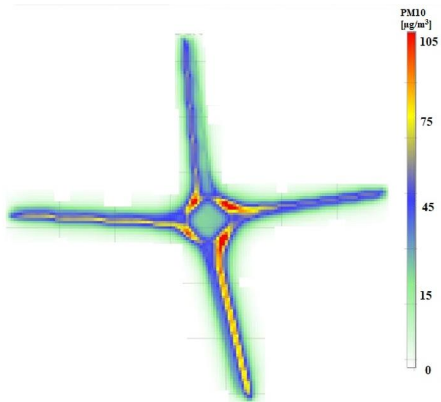
Figure 15. PM10 concentration related to monitored case study (two-lane roundabout) based on the VERSIT + model.
