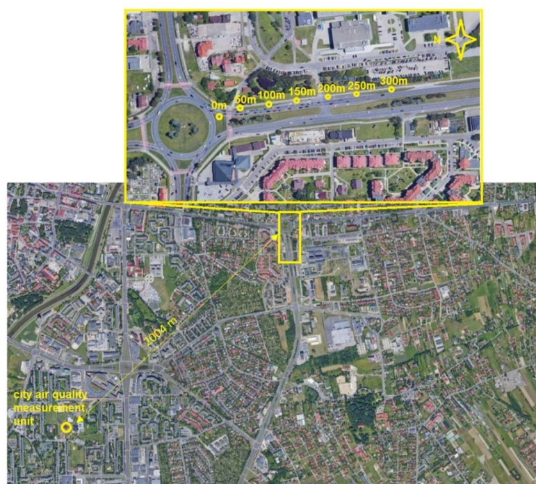
Figure 8. Place of measurement of particulate matter (PM) concentrations for the researched case study roundabout.
