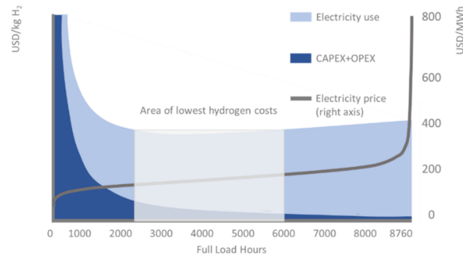
Figure A1. Levelized Cost of Hydrogen (LCOH) as a function of annual full load hours. Up to 2500 h, CAPEX costs dominate and costs decrease, OPEX other than electricity decreases as well and is included in CAPEX + OPEX. Above 6000 h OPEX related to electricity is most important. The optimum for this example case is between 2500 and 6000 h. (adapted from [81] with permission from IEA 2019).
