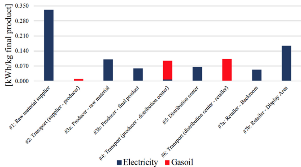
Figure 2. Specific energy consumption for each energy carrier and each actor of the cold chain.
