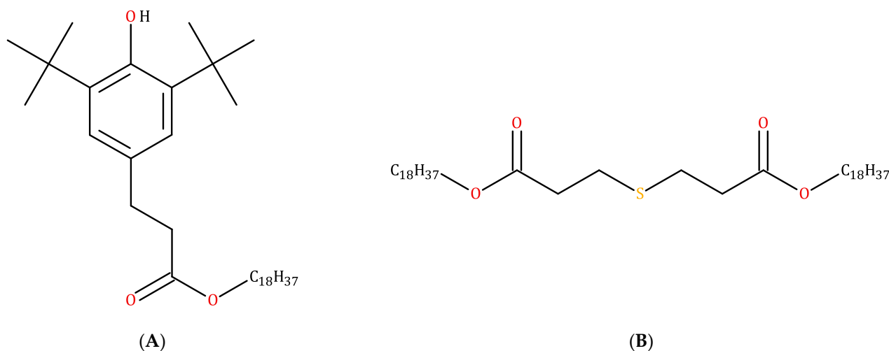
Figure 1. Chemical formula of antioxidants Irganox 1076 (A) and Irganox PS802 (B).
