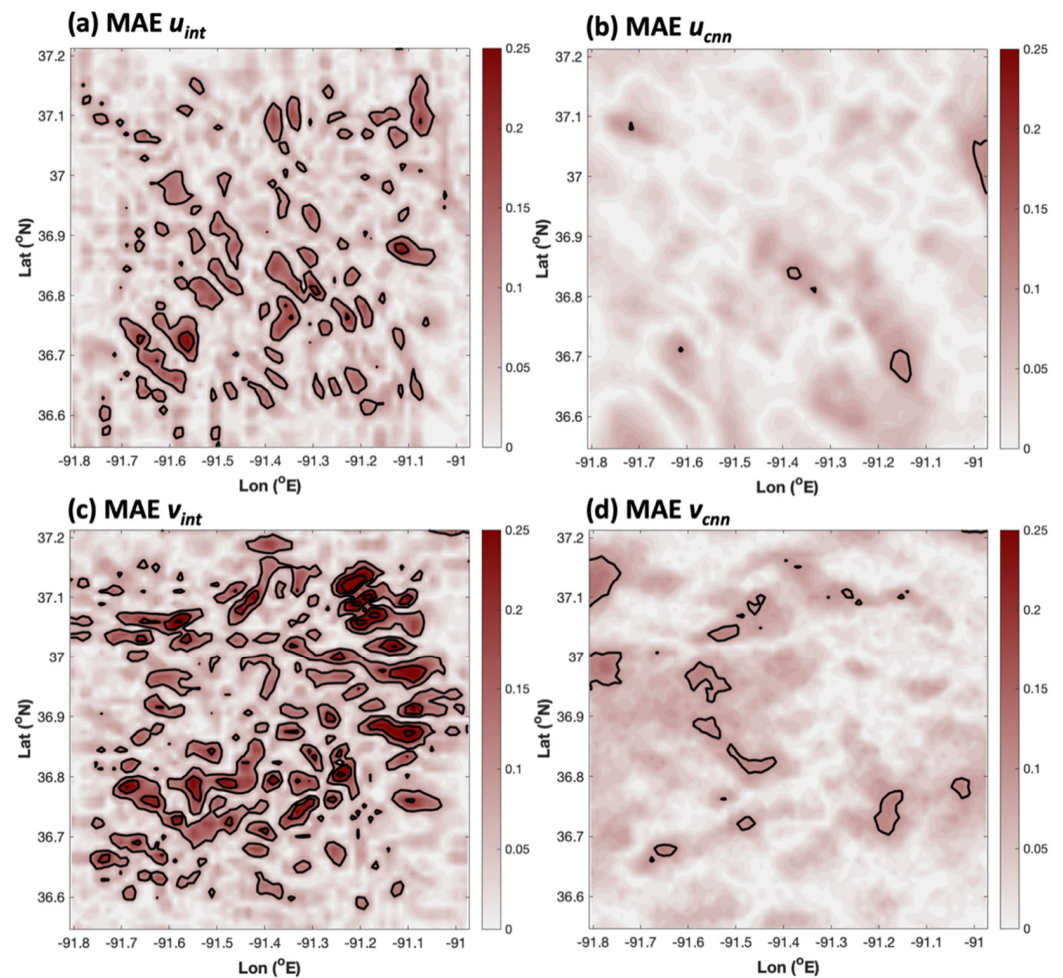
Figure 10. The grid 4 spatial distribution of MAE for (a) interpolated u (domain average MAE_{ave} = 0.050 \text{ m s}^{-1} ), (b) the CNN-produced u ( MAE_{ave} = 0.029 \text{ m s}^{-1} ), (c) interpolated v ( MAE_{ave} = 0.068 \text{ m s}^{-1} ), and (d) CNN-produced v ( MAE_{ave} = 0.041 \text{ m s}^{-1} ). Here, solid contours are plotted every 0.1 \text{ m s}^{-1} .
