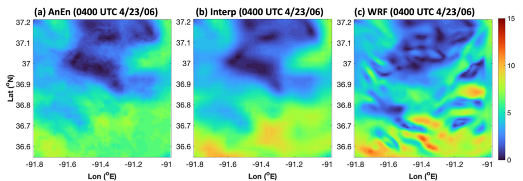
Figure 8. An example of a poor AnEn reconstruction of grid 4 winds for the total wind speed ( \text{RMSE} = 1.6 \text{ m s}^{-1} ). Plotted here is the grid 4 wind speed ( \text{m s}^{-1} ) at 0400 UTC 23 April 2006 produced by (a) the AnEn, (b) the interpolation, and (c) the WRF.
