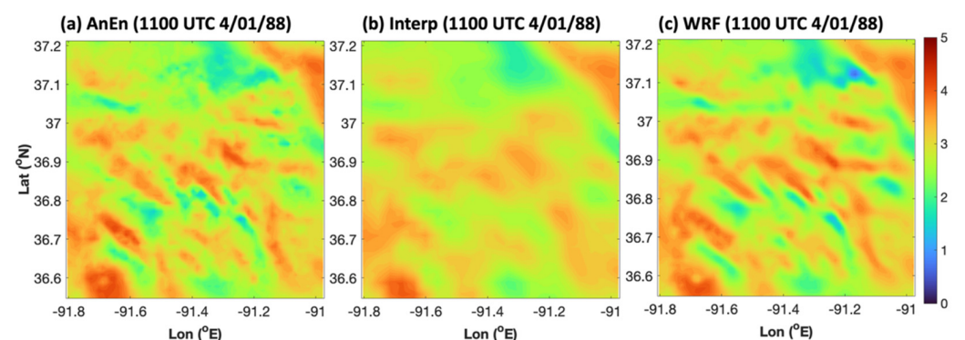
Figure 9. An example of a typical AnEn reconstruction of the total wind speed ( \text{RMSE} = 0.2 \text{ m s}^{-1} ). Plotted here is the grid 4 wind speed ( \text{m s}^{-1} ) at 1100 UTC 1 April 1988 produced by (a) the AnEn, (b) the interpolation, and (c) the WRF.
