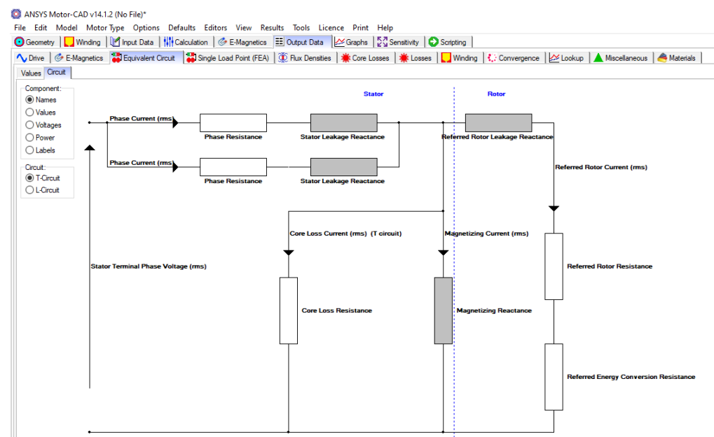
Figure 4. Equivalent Circuit Obtained from ANSYS MotorCAD.
