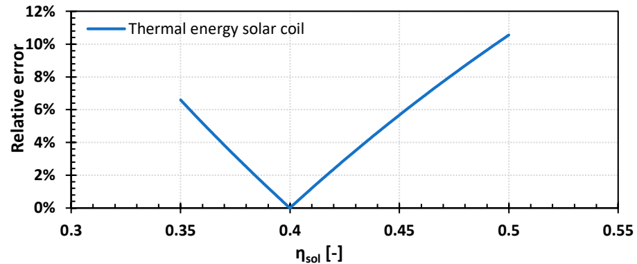
Figure 7. Relative error (absolute) of thermal energy from PVT delivered in the solar buffer tank vs. the effectiveness of the solar coil, \eta_{\text{sol}} .
