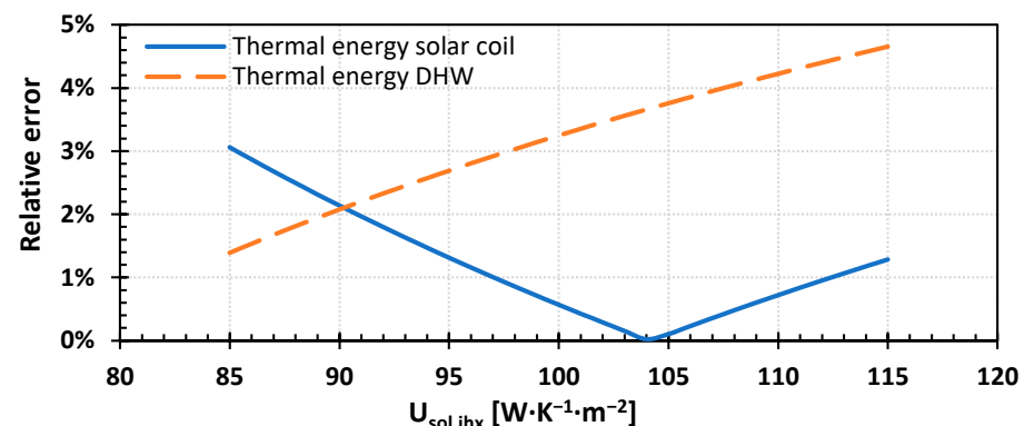
Figure 8. Relative errors (absolute) of thermal energy from PVT delivered in the DHW tank (continuous) and absorbed by the DHW (dotted) vs. heat transfer coefficient of the solar IHX, U_{\text{sol.ihx}} .
