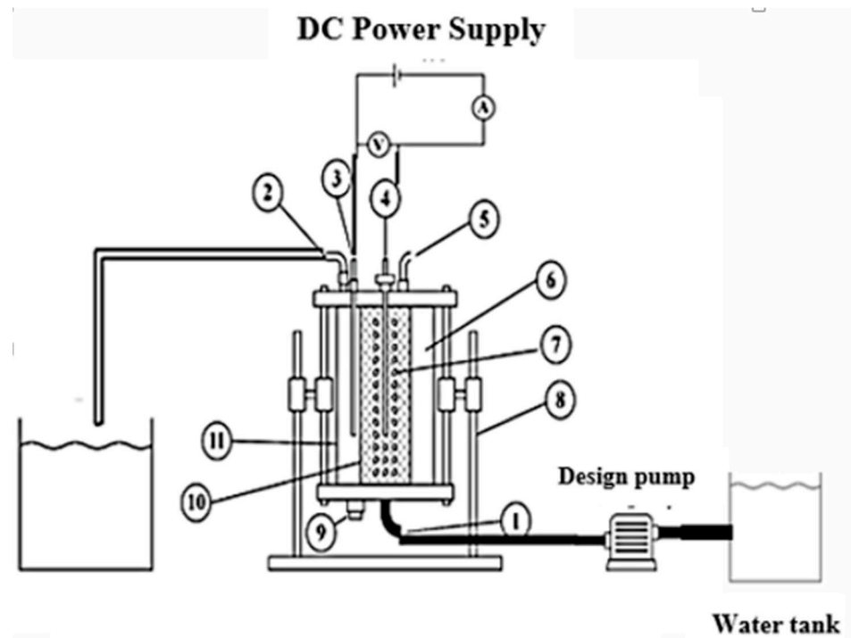
Figure 2. Electrochemical cell for the treatment of salty water using a flow-by electrode. 1. Feed inlet; 2. Outlet; 3. Rod ( D = 0.8 cm) anode current collector; 4. Rod ( D = 0.8 cm) cathode current collector; 5. Gas vent; 6. Graphite (granules); 7. Cylindrical tube made of UPVC; 8. Support; 9. Graphite feed inlet; 10. Metal screen; 11. Plexiglas.
