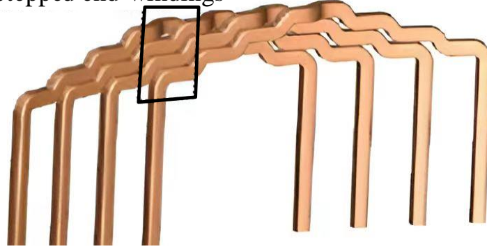
Figure 13. Stepped end-windings.
