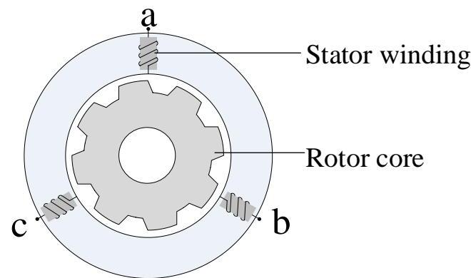
Figure 6. Schematic diagram of SRM (where a,b,c denote 3-phase windings).
