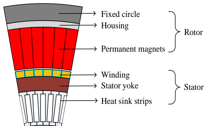
Figure 17. Slotless high-speed propulsion motor.
