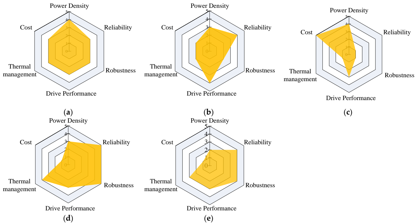
Figure 7. Performance comparison chart for five types of motor. (a) SRM; (b) IM; (c) PMSM; (d) HTSM; (e) WFSM.
