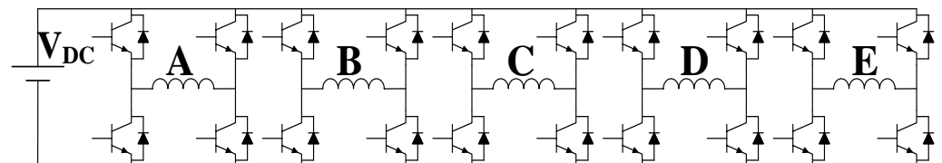
Figure 29. Common DC bus open-winding inverter structure.
