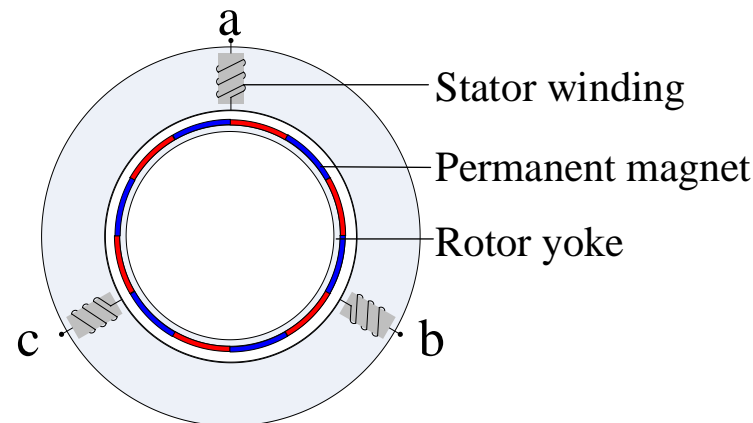
Figure 2. Schematic diagram of the structure of the PMSM (where a,b,c denote 3-phase windings).
