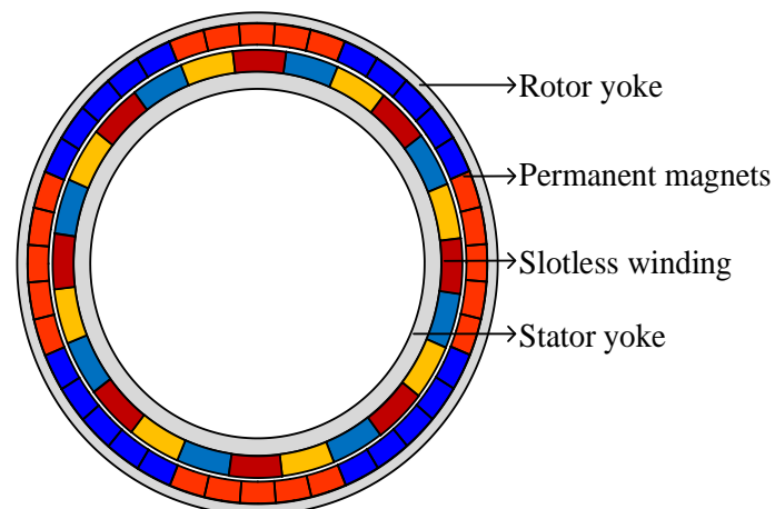
Figure 10. Slotless Halbach array propulsion motor.
