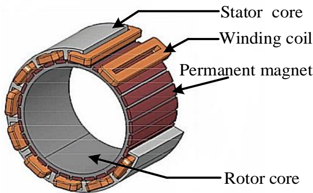
Figure 27. A 4 \times 3 -phase motor structure. (a) 3D structure; (b) winding extension.
