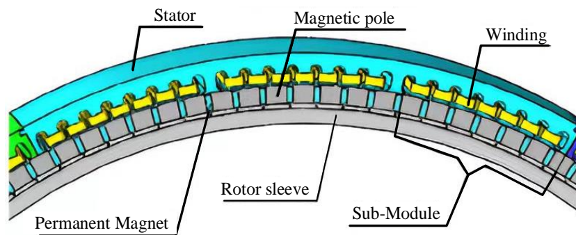
Figure 35. Non-winding winding.
