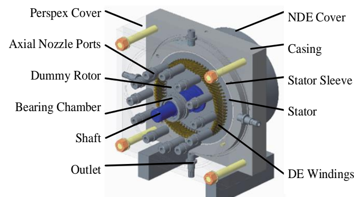
Figure 14. University of Nottingham injection cooling test setup.
