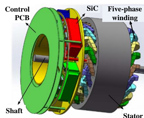
Figure 23. 3D model of integrated motor system.
