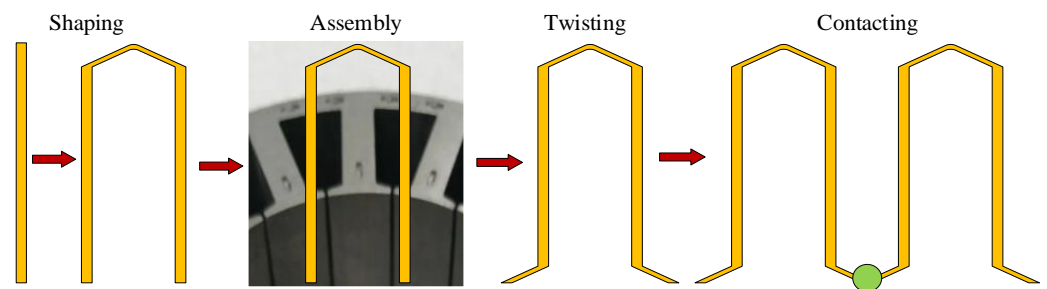
Figure 16. Manufacturing process of hairpin windings.
