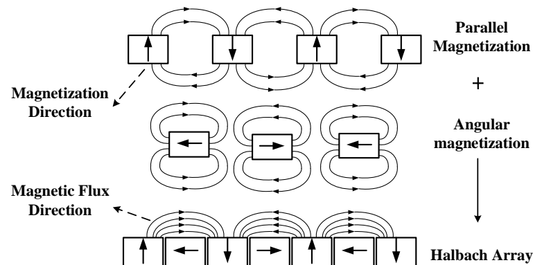
Figure 8. Schematic diagram of Halbach array principle.
