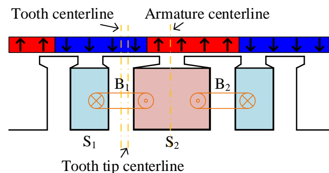
Figure 33. Unequal-width tooth structure.
