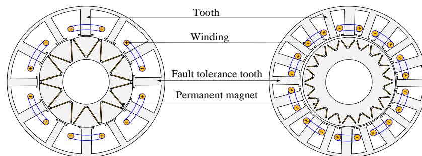
Figure 25. Three-phase and five-phase structures.
