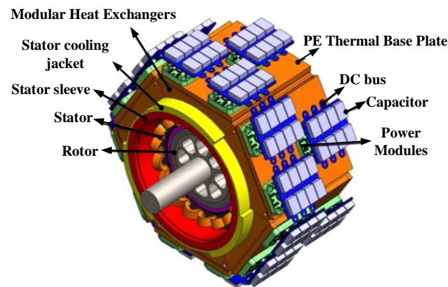
Figure 22. MW-class integrated modular motor drive configuration.
