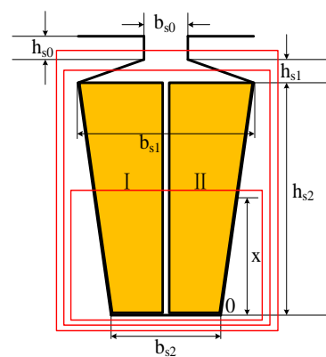
Figure 37. Slot leakage inductance analysis diagram.
