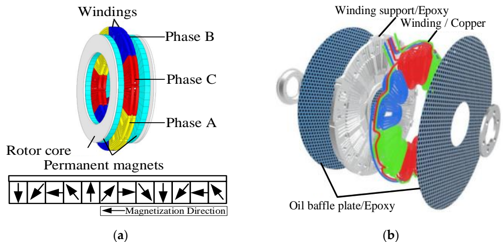
Figure 19. Axial flux high-speed motors. (a) 3D model; (b) non-iron-core stator.
