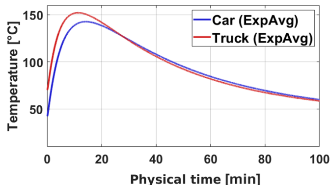
Figure 10. Cool-down curves of TK21 (the cold part right above the heatshield) for car and truck configurations.
