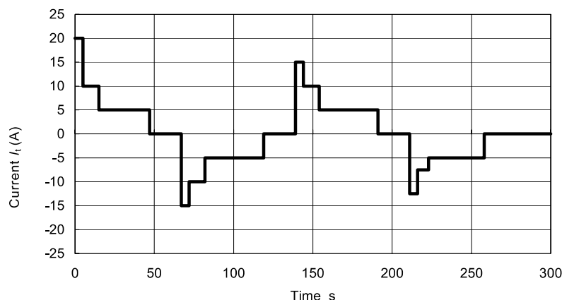
Figure 16. New life cycle method for high power applications [28].
